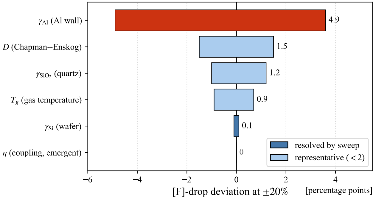
Parameter sensitivity of the wafer [F] drop
