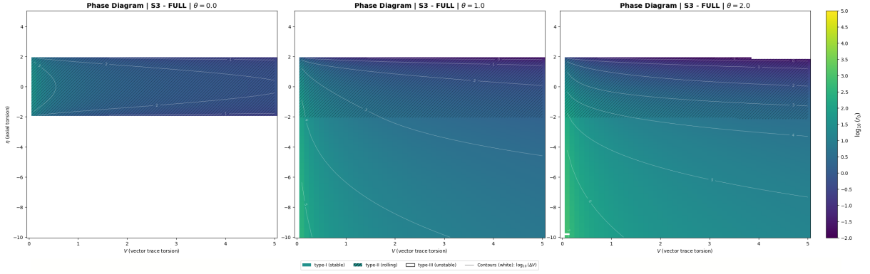
Figure 9: Phase diagram: S^3 \times S^1 ( \theta_{\text{NY}} = 0, 1, 2 ).
