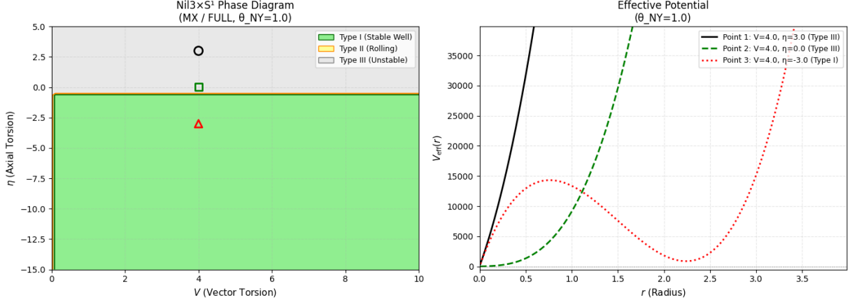
Figure 16: Phase-potential correspondence for \text{Nil}^3 \times S^1 ( \theta_{NY} = 1 ).
