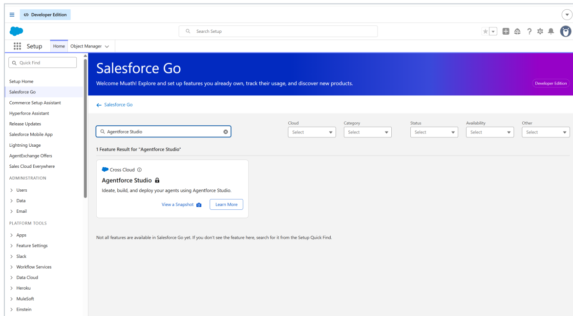
Figure 3 — Salesforce Go returns a single Agentforce Studio feature result, but the tile carries a lock icon indicating it is not enabled.
