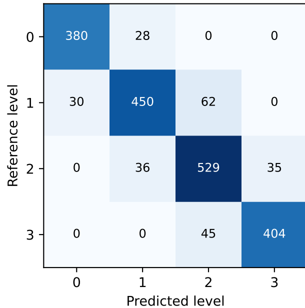
HistGradientBoosting
