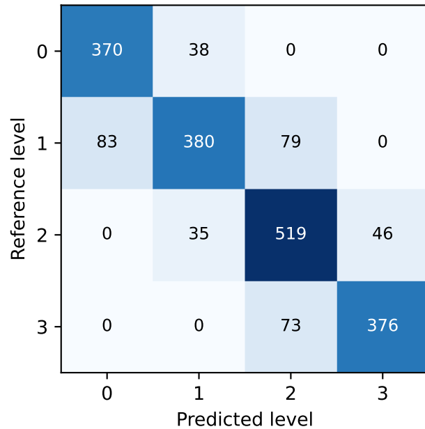
Random Forest
