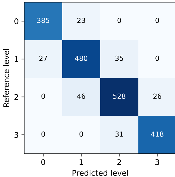
Logistic Regression
