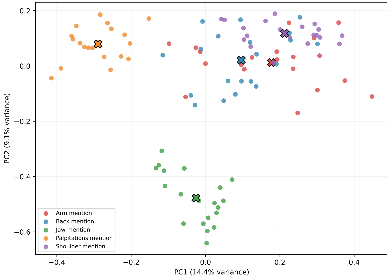
Run 3 | seed 404 | 100 complaints
