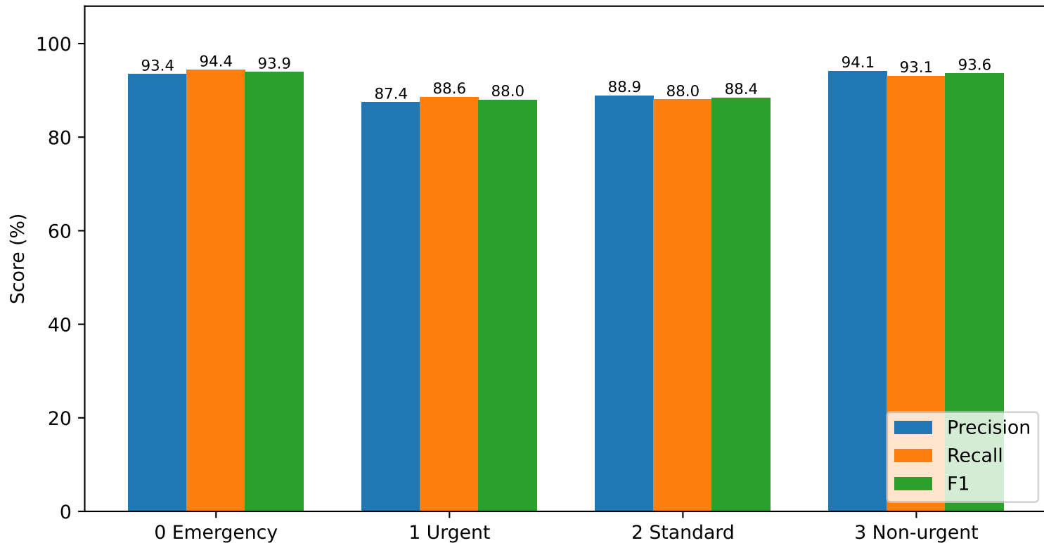
Selected model: individual class performance
