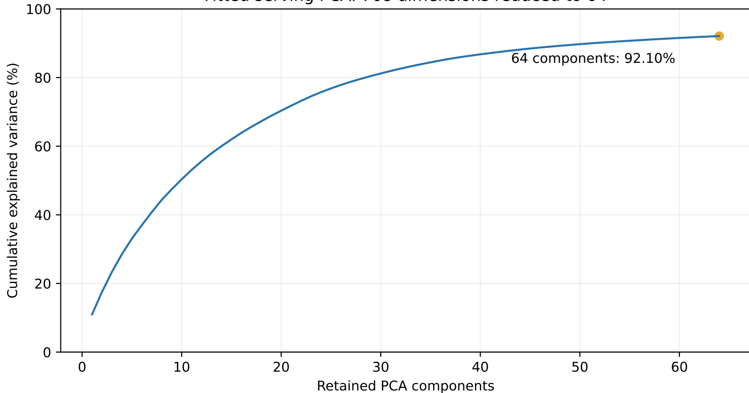
Fitted serving PCA: 768 dimensions reduced to 64
