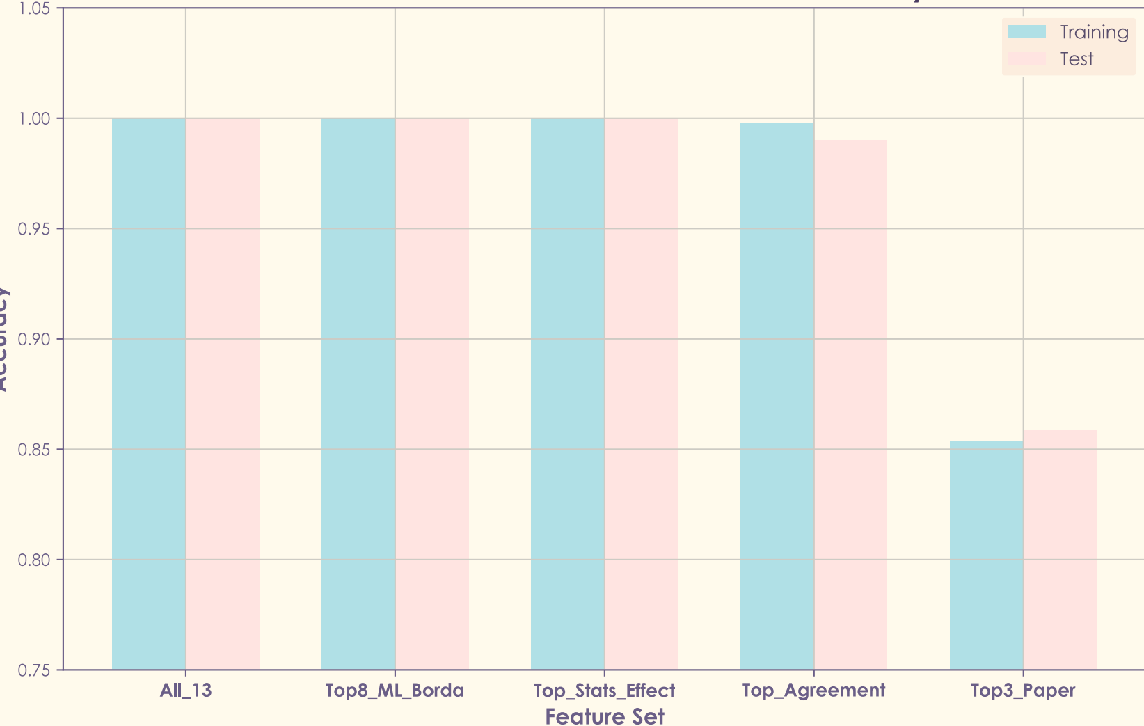
Baseline Performance: Train vs Test Accuracy
