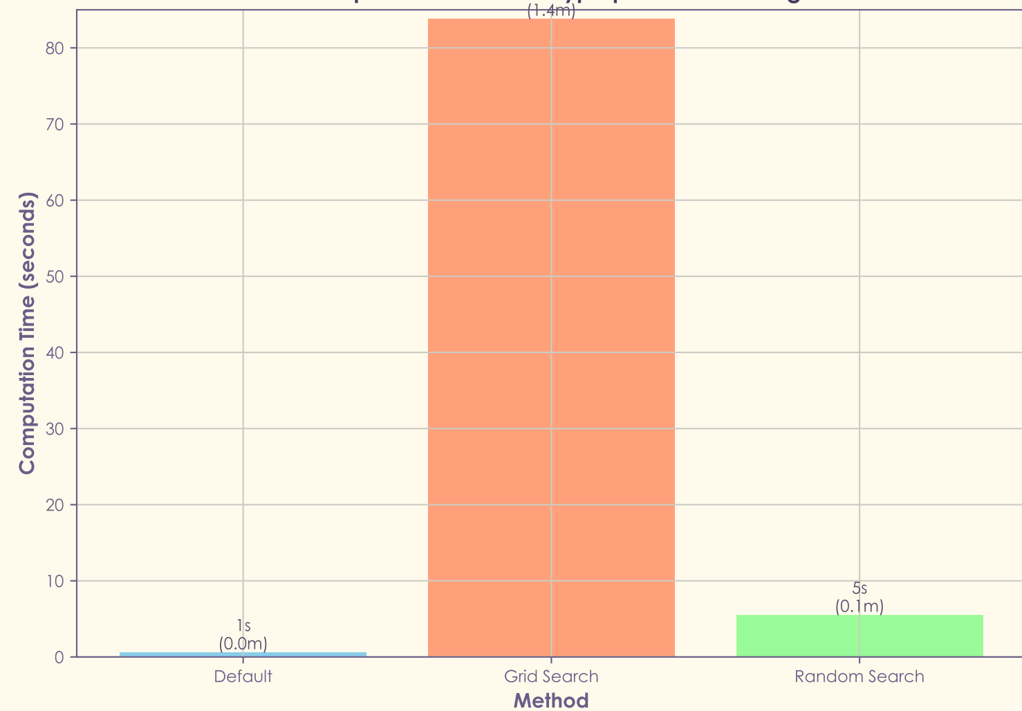
Computational Cost of Hyperparameter Tuning
