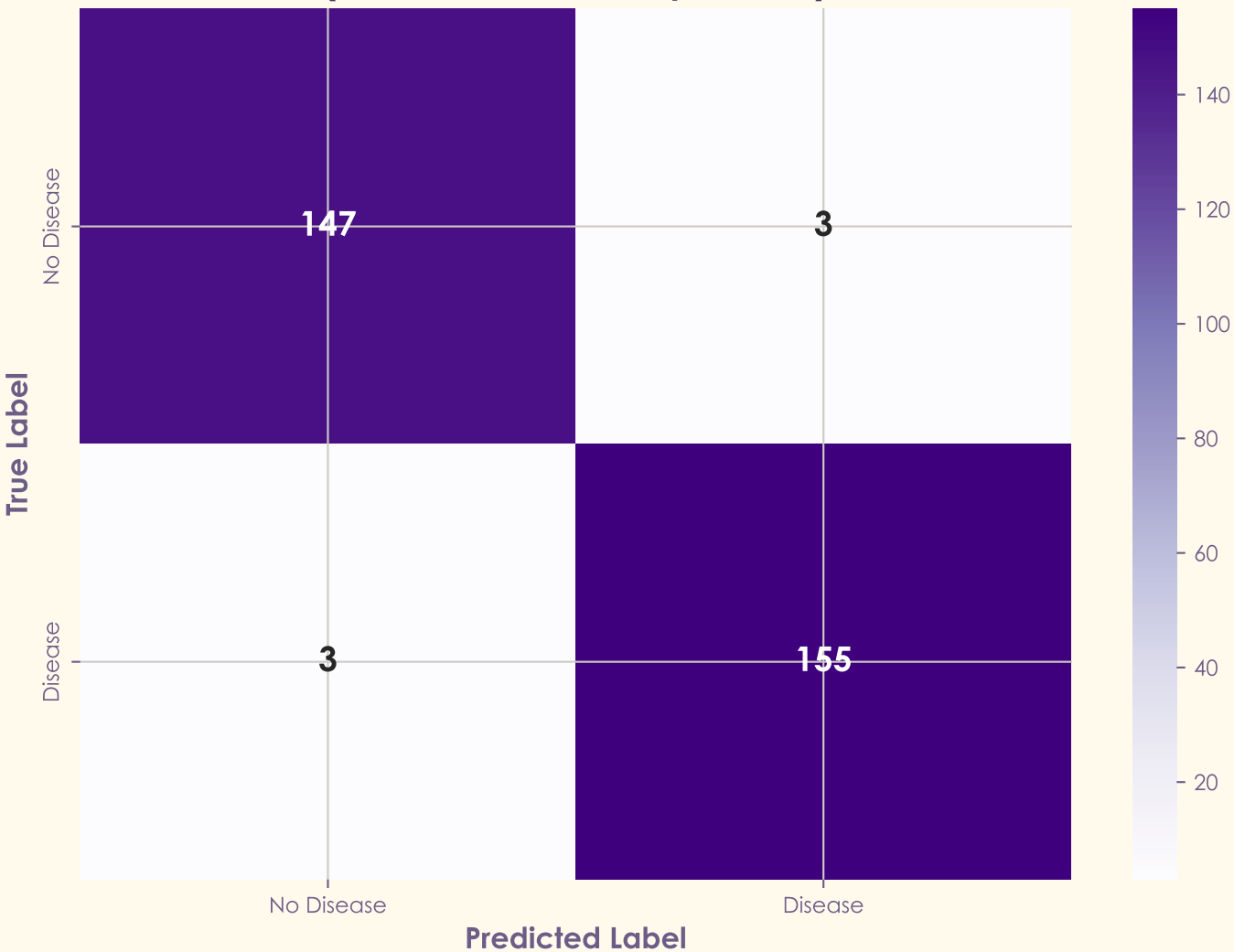
Confusion Matrix: Final Model (8 Features, Accuracy=0.9805)
