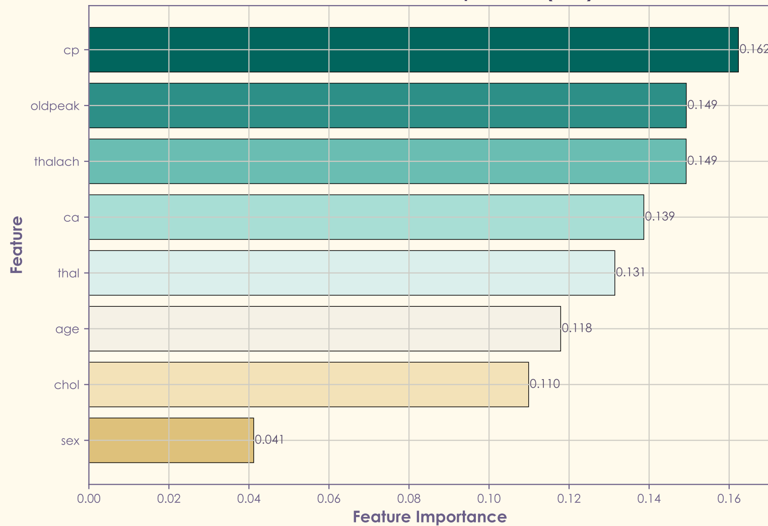
Final Model: Feature Importance (Gini)
