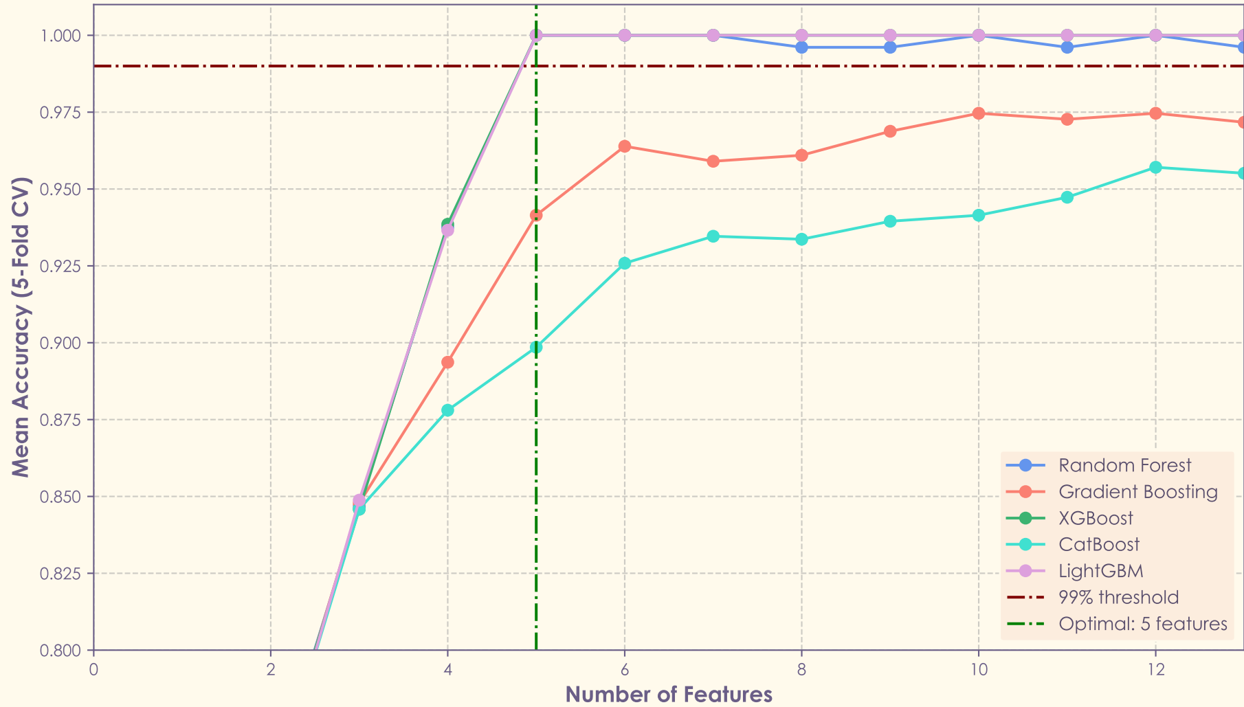
Progressive Feature Selection: All Classifiers (Sophisticated Analysis)
