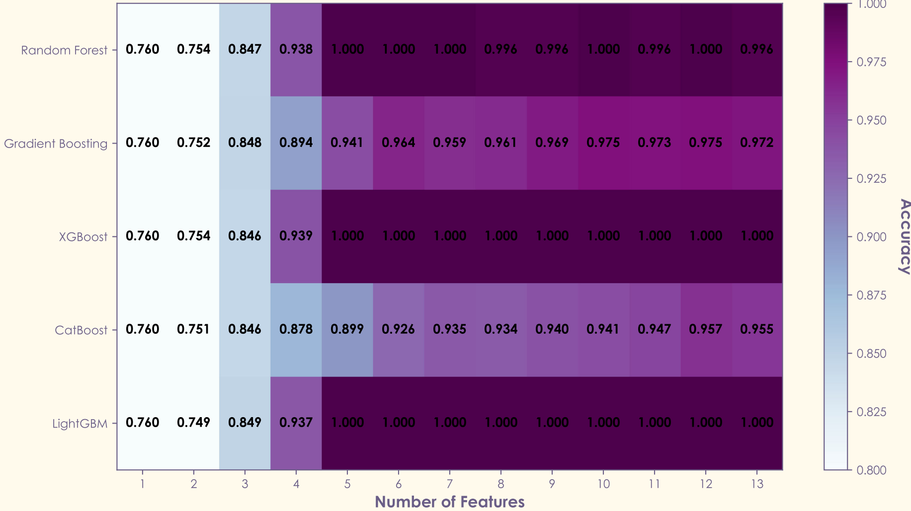
Classifier Performance Heatmap
