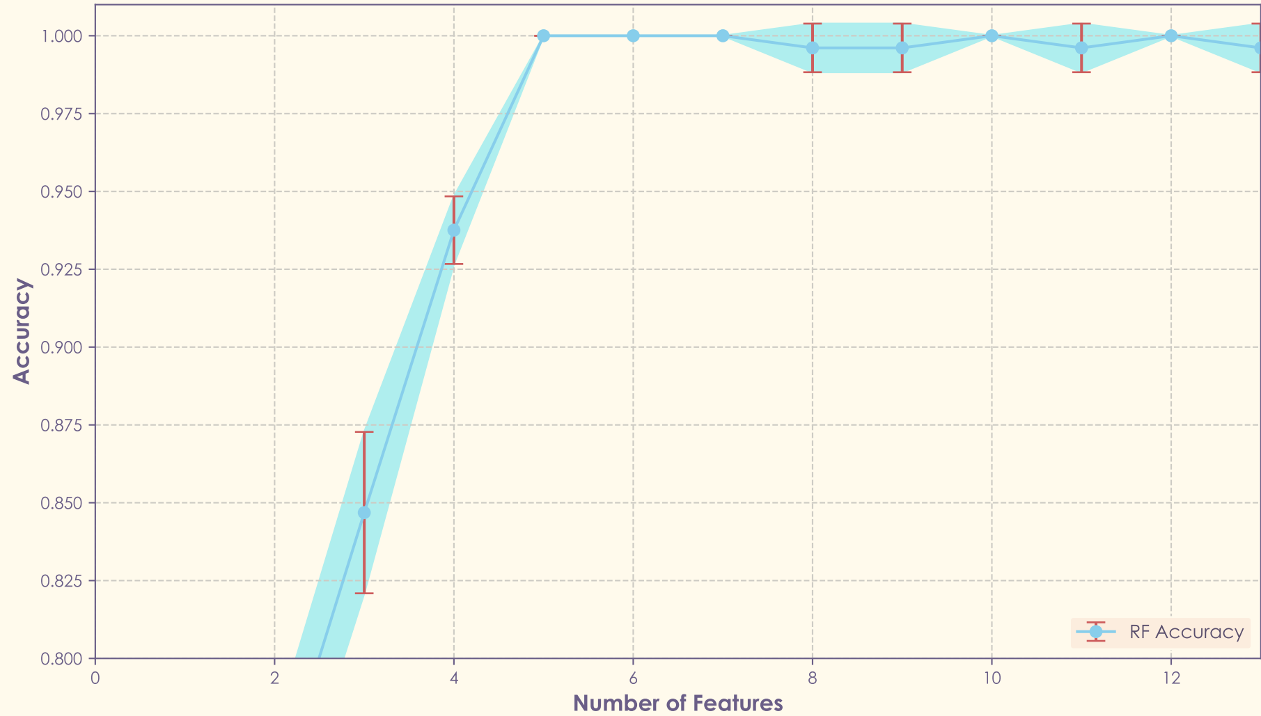
Marginal Performance Improvement (Diminishing Returns)
