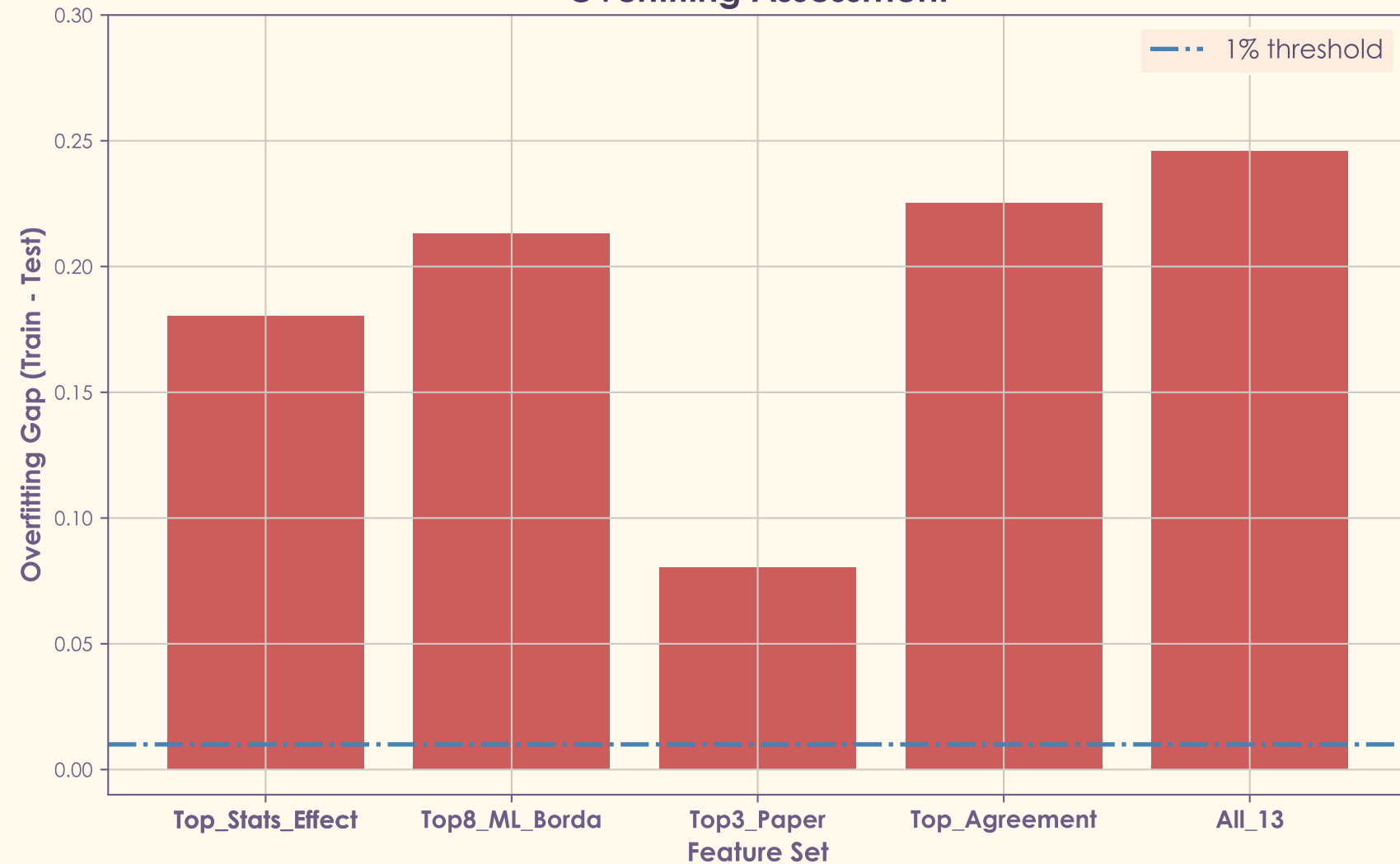
Overfitting Assessment
