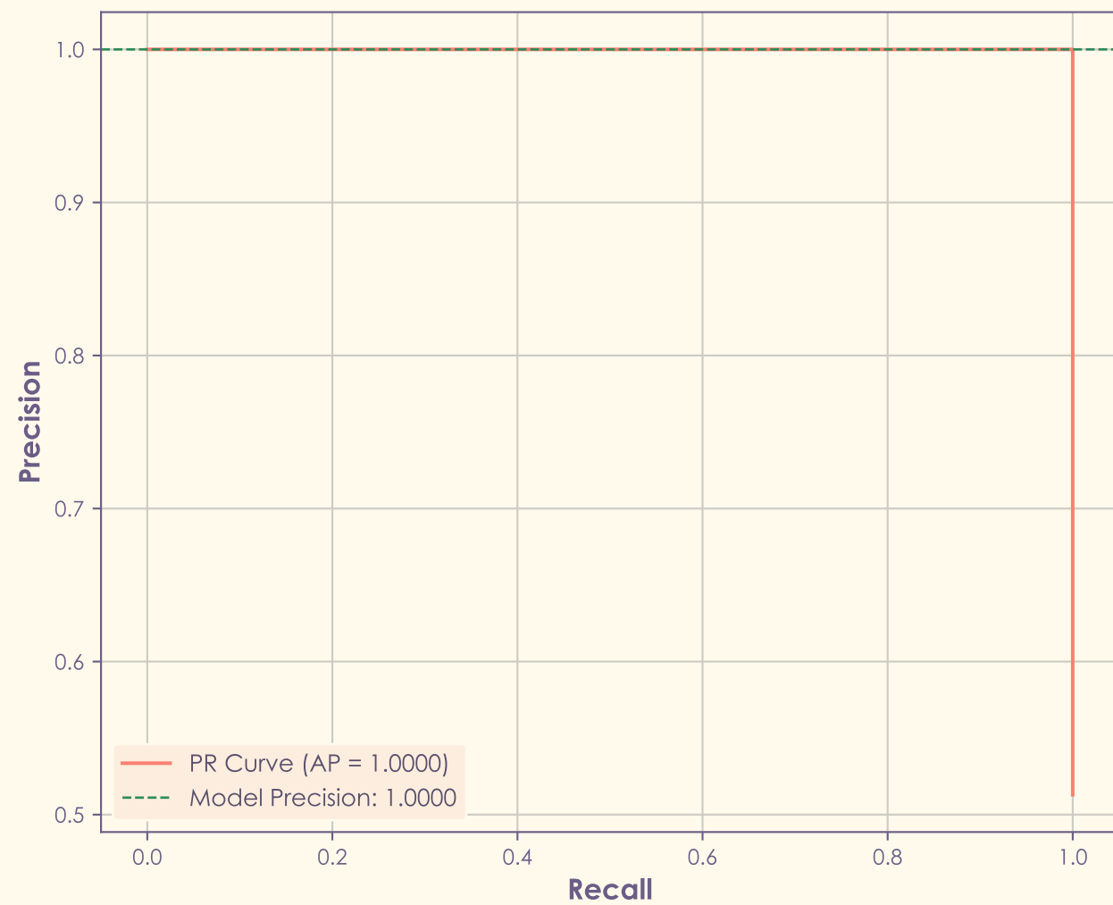
Precision-Recall Curve: Final Model
