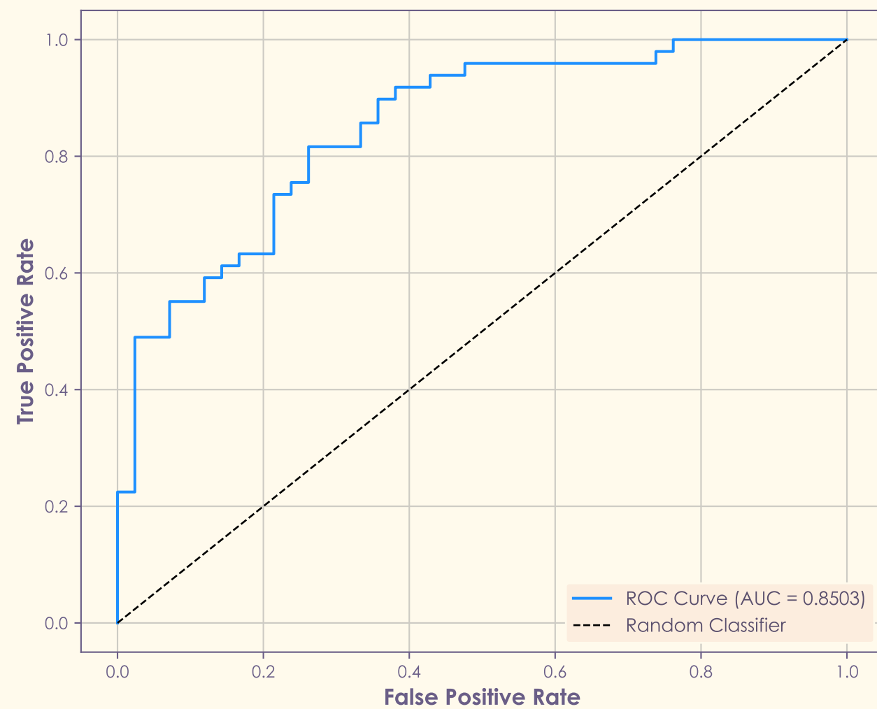
ROC Curve: Final Model
