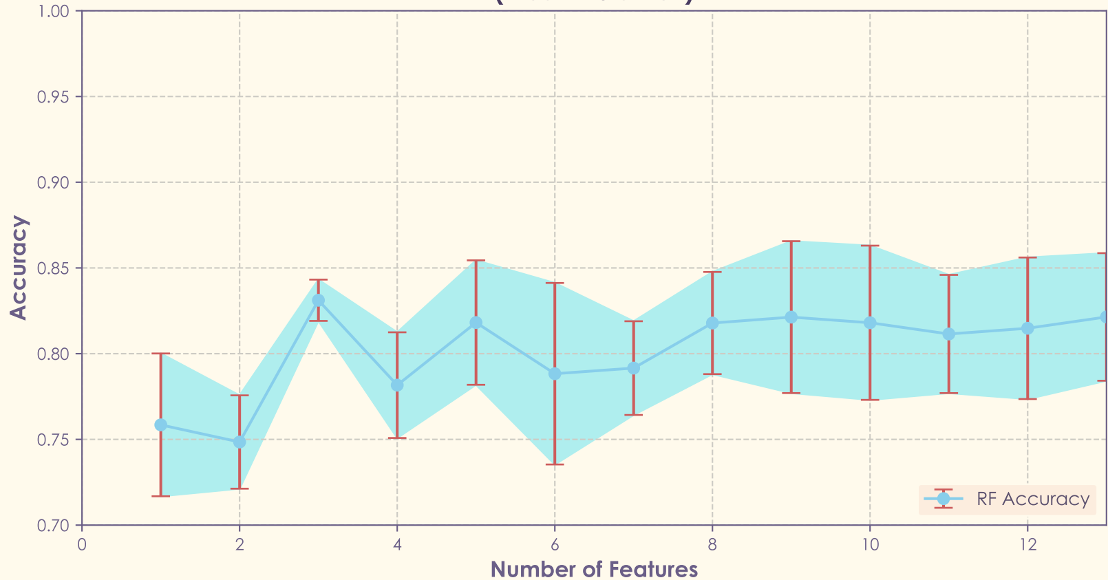
Marginal Performance Improvement (Diminishing Returns)
