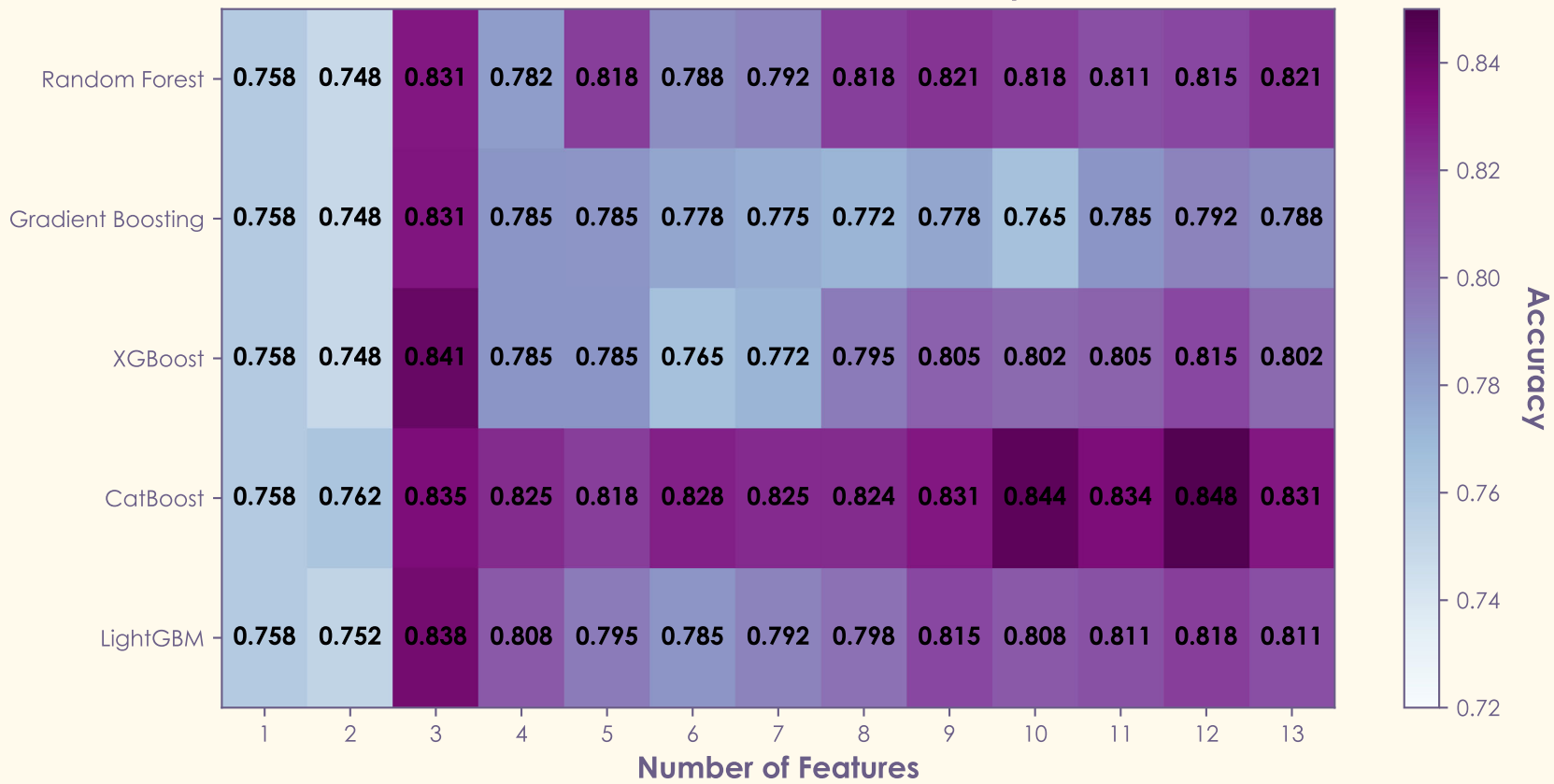
Classifier Performance Heatmap
