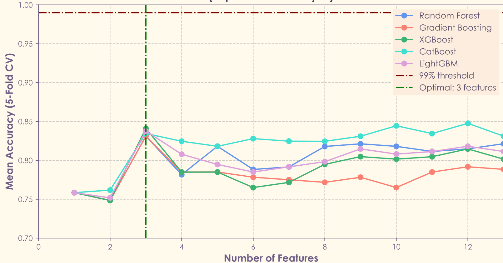
Progressive Feature Selection: All Classifiers (Sophisticated Analysis)
