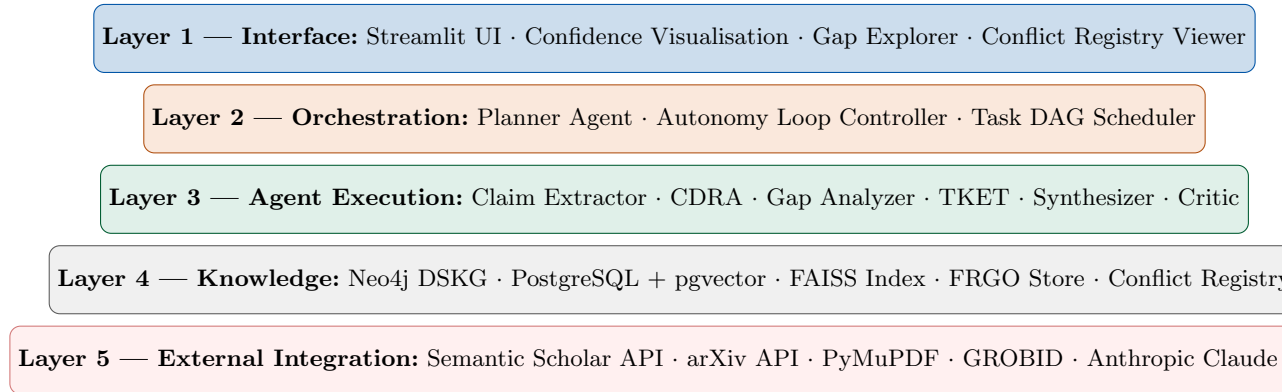
Fig. 6: Layered system architecture. Data flows upward through the stack during synthesis (Layers 5 \rightarrow 1) and downward during refinement cycles (Layer 2 dispatches to Layers 3–5).
