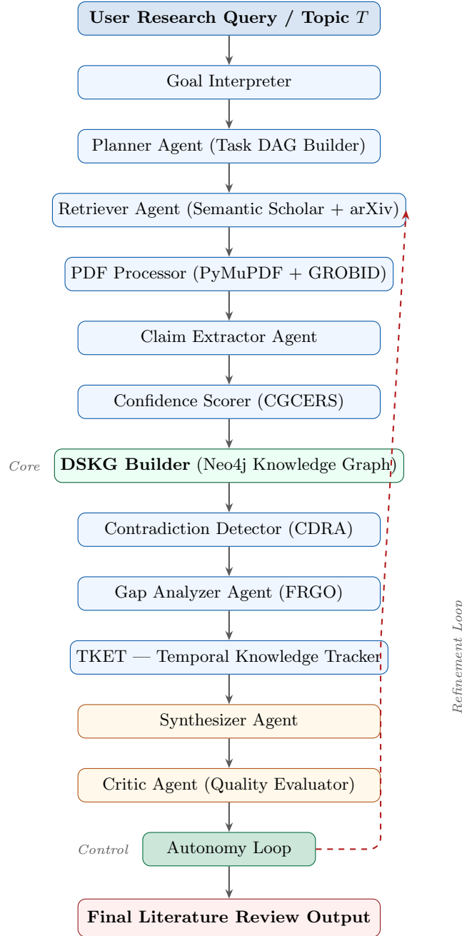
Fig. 1: Complete multi-agent literature review workflow. The dashed red arrow depicts the autonomy feedback loop that triggers targeted re-retrieval when critic quality scores fall below threshold Q^* .
