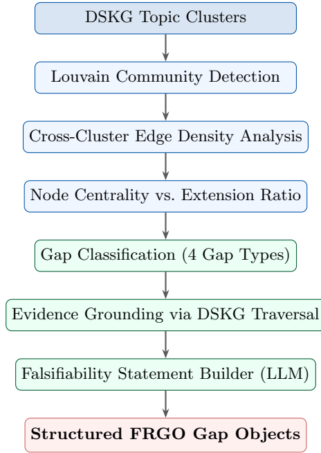
Fig. 3: Research gap generation flow. Structural graph properties—community density, centrality ratios, and contradiction edge clustering—drive automated gap identification before LLM-based formalization.
