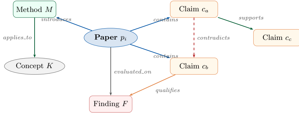
Fig. 4: DSKG heterogeneous graph schema showing node types and typed epistemic edge relationships. Dashed red edges represent contradiction links; all other edges encode supportive or relational epistemic connections.
