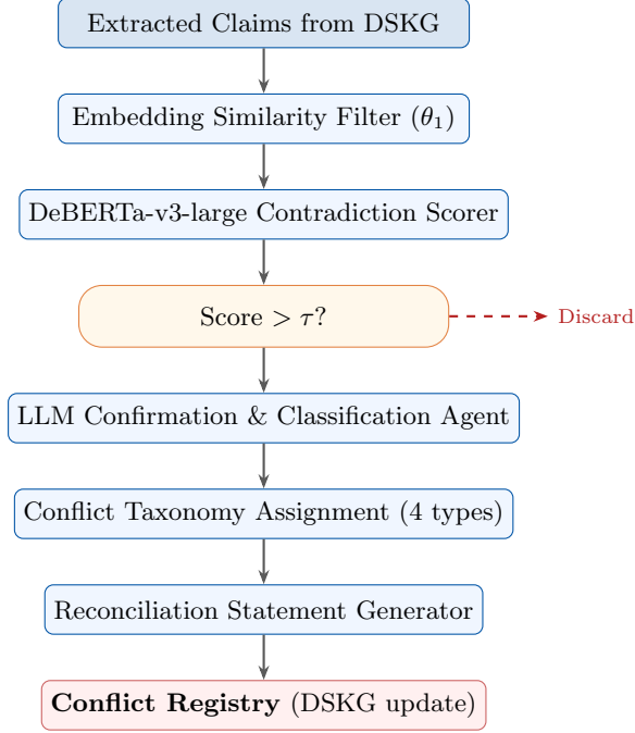
Fig. 2: Two-stage contradiction detection and resolution pipeline. Only claim pairs passing the DeBERTa threshold \tau are forwarded to the LLM classification stage.
