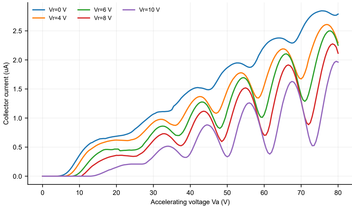
Raw argon Frank-Hertz curves
