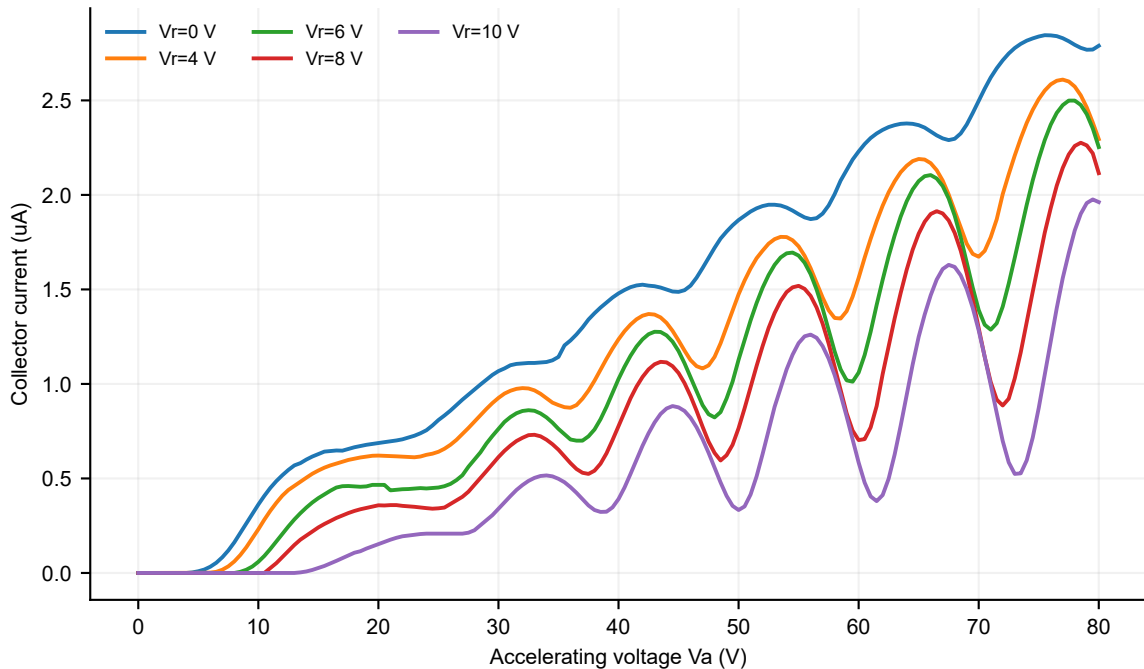
Raw argon Franck-Hertz curves
