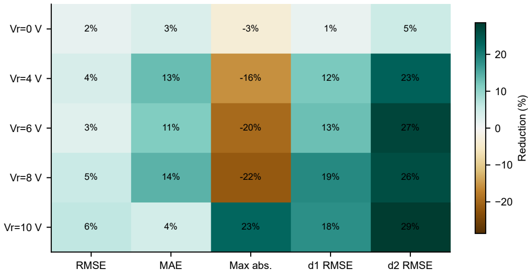
K=4 error reduction relative to K=1 by curve
