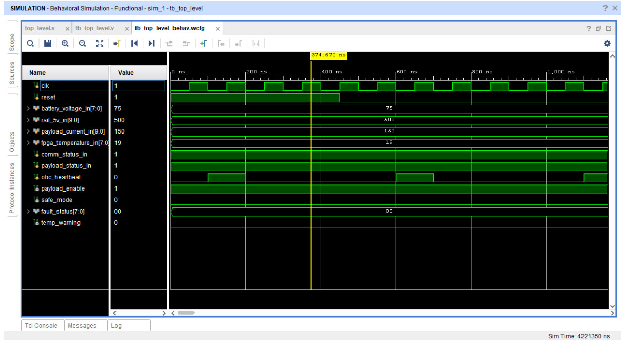
Figure 2: Simulation waveform showing monitored parameters, fault status, and protection outputs.
