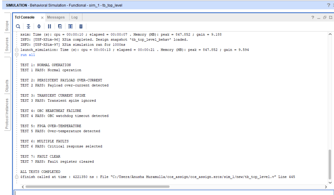
Figure 3: Testbench output showing successful completion of all seven test cases.
