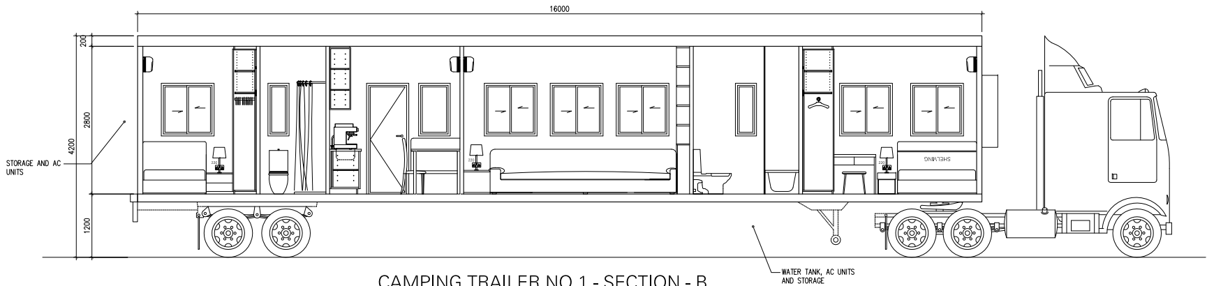
CAMPING TRAILER NO.1 - SECTION - B SCALE - 1:50
