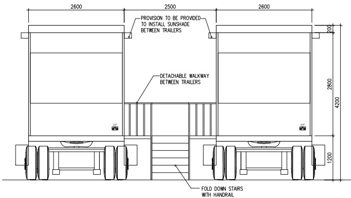
FRONT ELEVATION - 04 SCALE - 1:50
