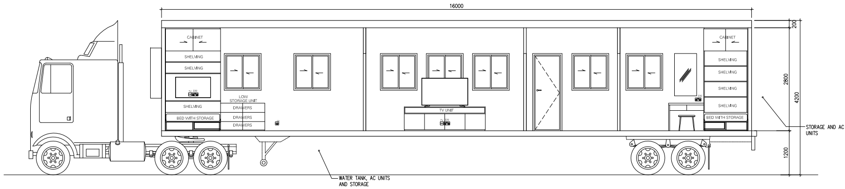
CAMPING TRAILER NO.1 - SECTION - A SCALE - 1:50
