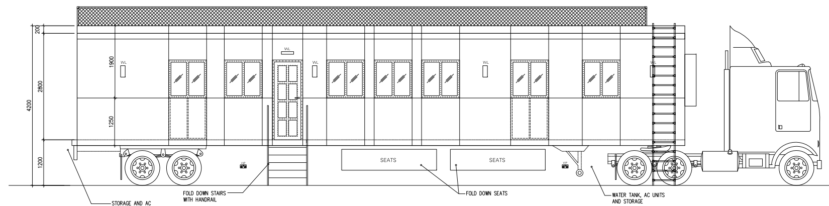
CAMPING TRAILER NO.1 ELEVATION - 02 SCALE - 1:50
