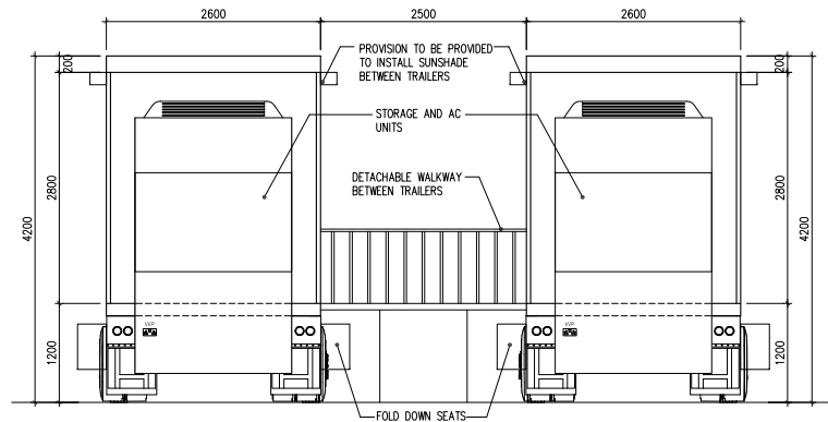
BACK ELEVATION - 03 SCALE - 1:50
