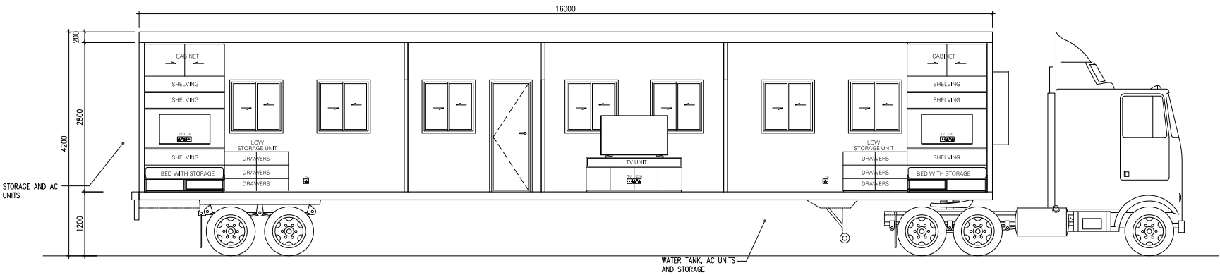
CAMPING TRAILER NO.2 - SECTION - D SCALE - 1:50
