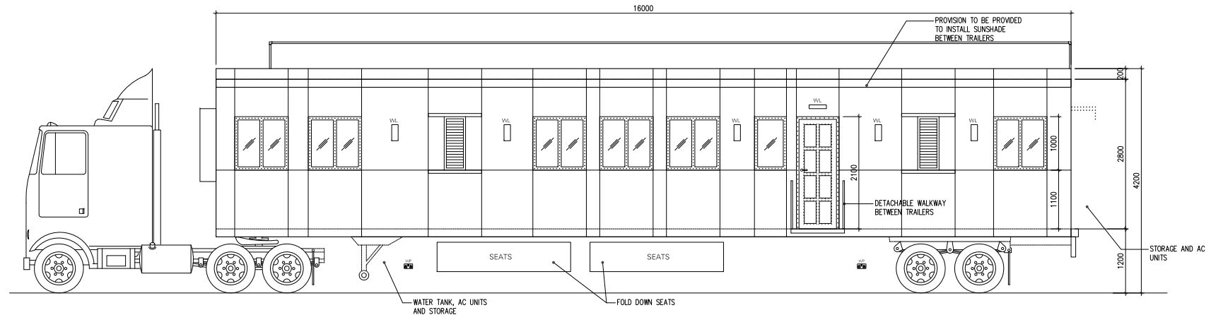
CAMPING TRAILER NO.1 ELEVATION - 01 SCALE - 1:50
