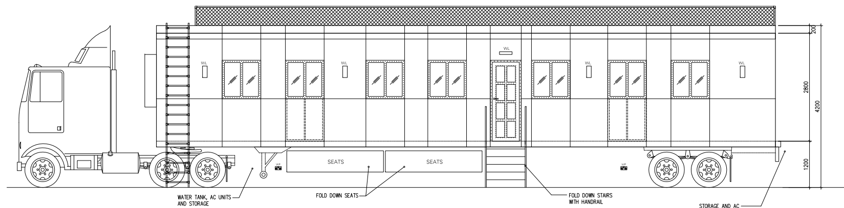
CAMPING TRAILER NO.2 ELEVATION - 06 SCALE - 1:50
