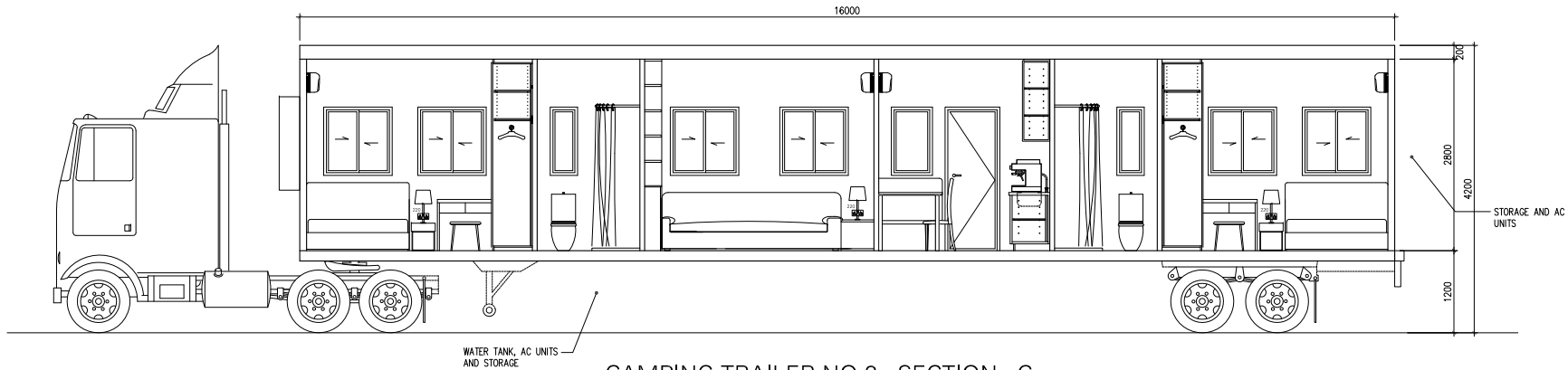
CAMPING TRAILER NO.2 - SECTION - C SCALE - 1:50
