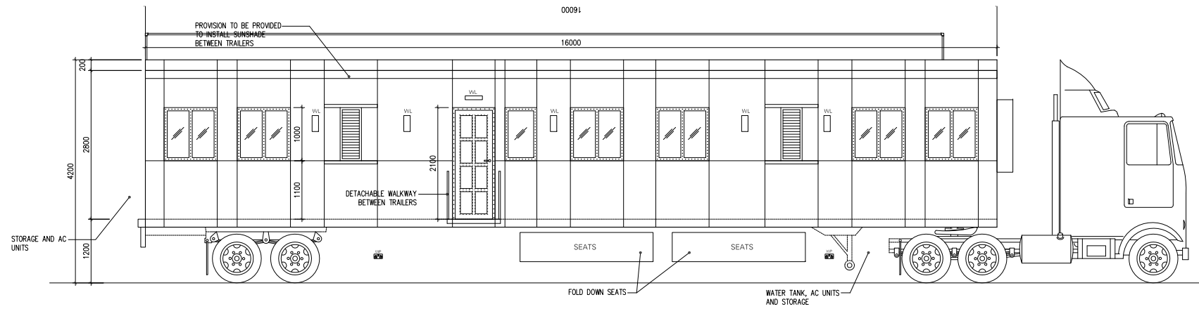
CAMPING TRAILER NO.2 ELEVATION - 05 SCALE - 1:50
