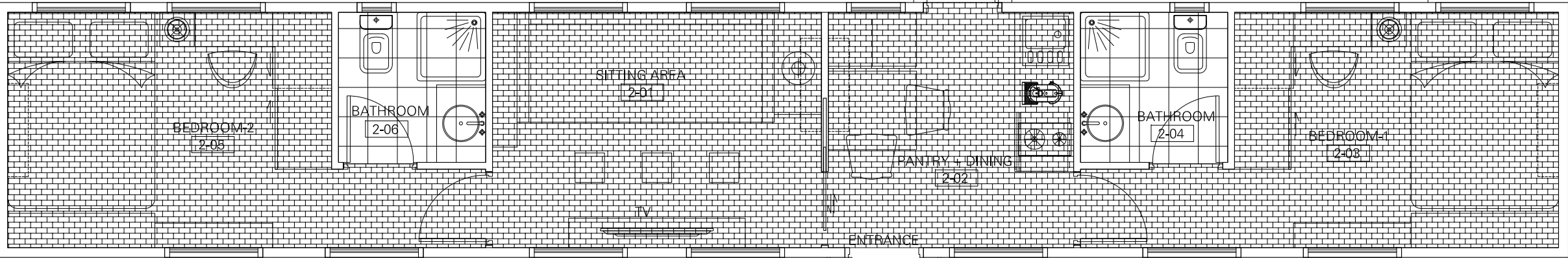
CAMPING TRAILER NO.2 FLOORING LAYOUT
