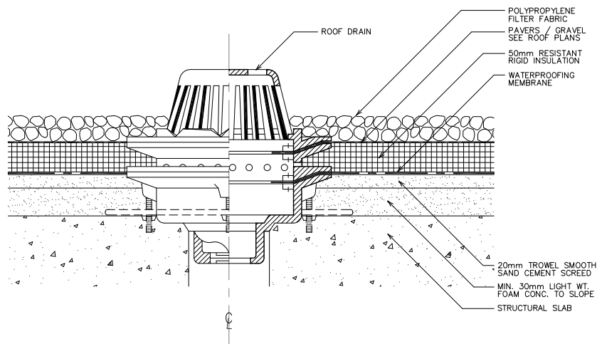
4 TYPICAL ROOFING DETAIL AT ROOF DRAIN A110400 SCALE: 1:5 M.
