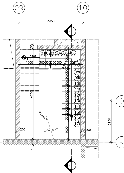
STAIR NO.-4-BASEMENT FLOOR PLAN SCALE : 1/50
