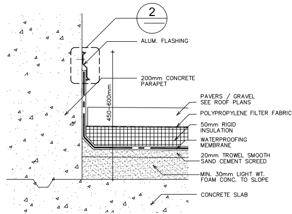
1 TYPICAL ROOFING DETAIL AT PARAPET A110400 SCALE: 1:5 M.
