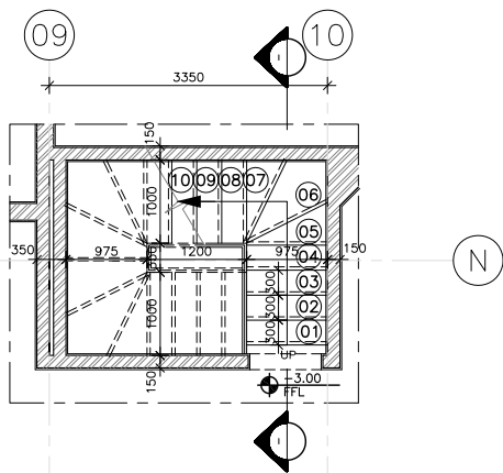
STAIR NO.-3-BASEMENT FLOOR PLAN SCALE : 1/50
