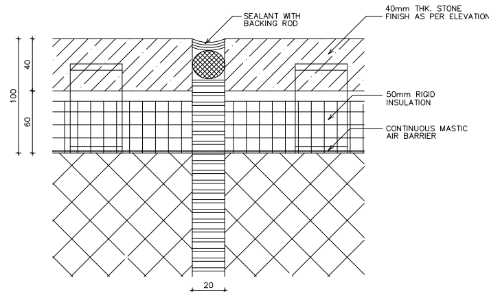
8 EXPANSION JOINT AT EXTERNAL STONE FINISH A110400 SCALE: 1:2 M.
