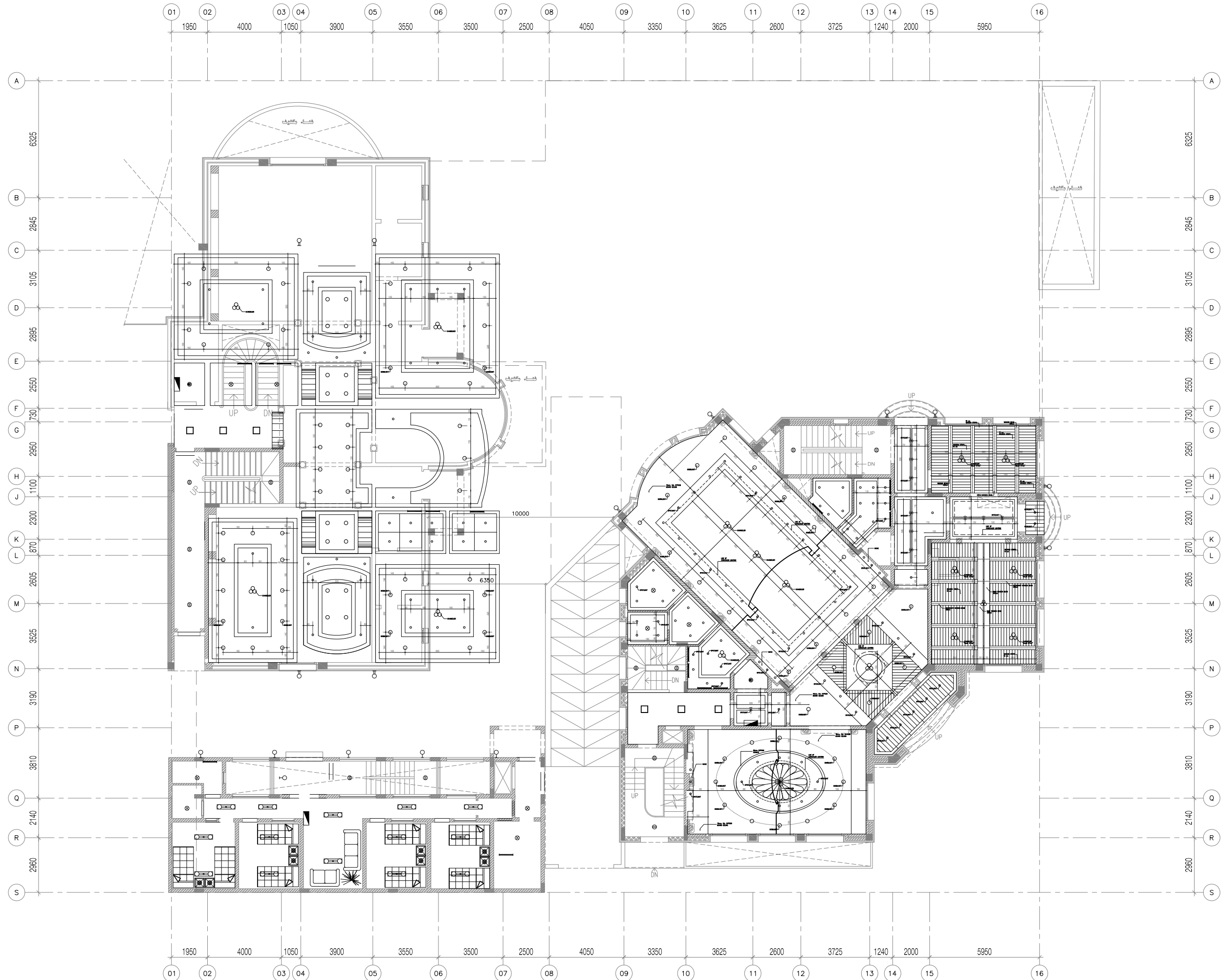
1 GROUND FLOOR PLAN REFLECTED CEILING LAYOUT A060101 SCALE: 1:100 M.
