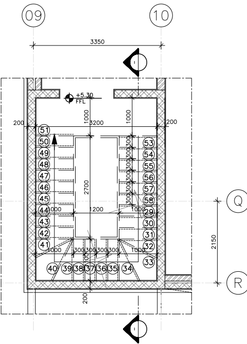
STAIR NO.-4-FIRST FLOOR PLAN SCALE : 1/50
