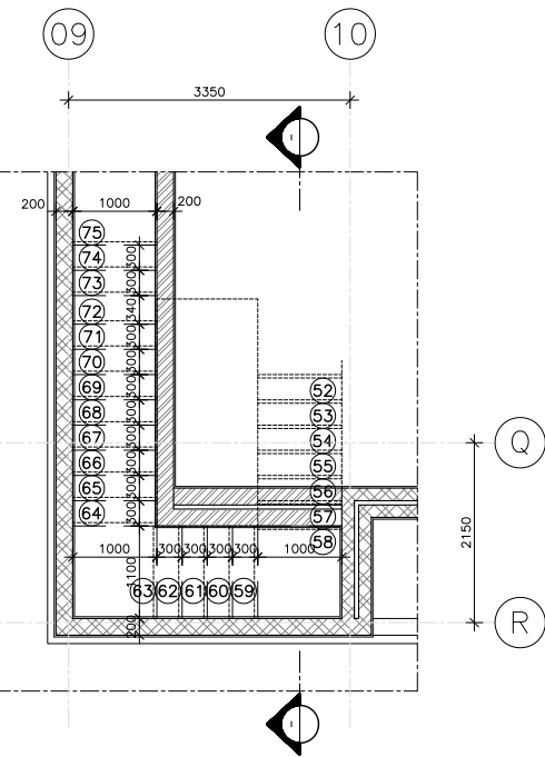
STAIR NO.-4-ROOF FLOOR PLAN SCALE : 1/50
