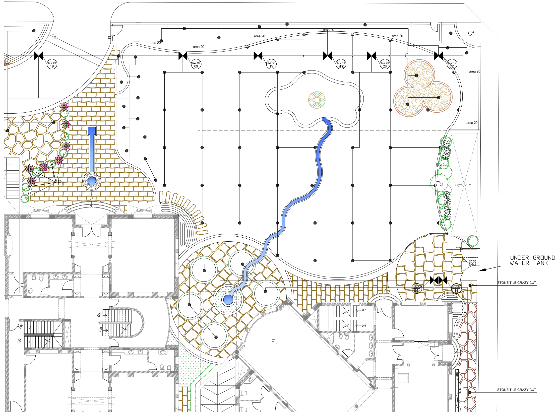
1 LANDSCAPE DIMENSION LAYOUT PART 2/4 A130102 SCALE: 1:100 M.
