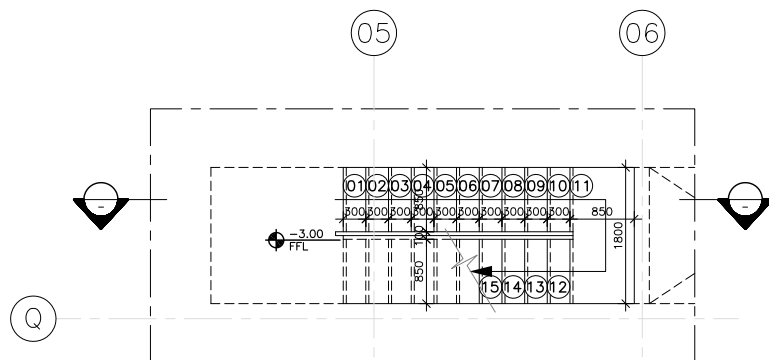
STAIR NO.-6-BASEMENT FLOOR PLAN SCALE : 1/50
