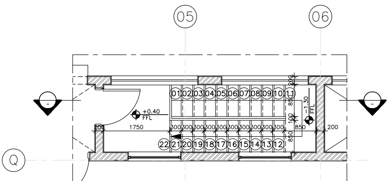
STAIR NO.-6-GROUND FLOOR PLAN SCALE : 1/50
