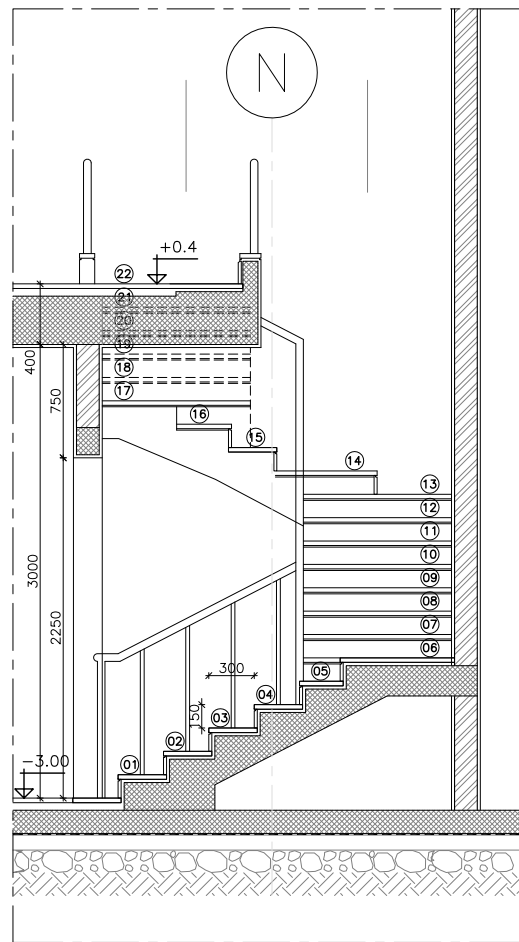
STAIR NO.-3-SECTION A-A SCALE : 1/20
