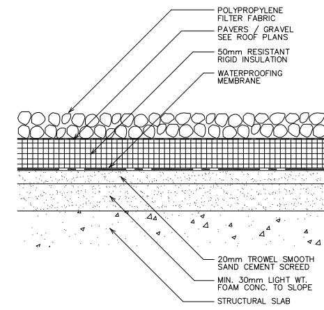
3 TYPICAL ROOFING DETAIL A110400 SCALE: 1:5 M.
