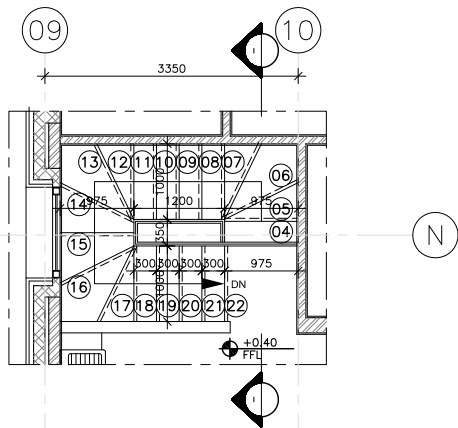
STAIR NO.-3-GROUND FLOOR PLAN SCALE : 1/50
