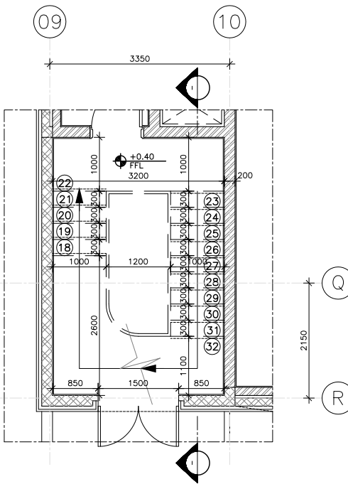
STAIR NO.-4-GROUND FLOOR PLAN SCALE : 1/50
