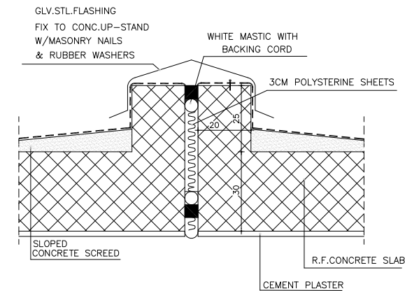
9 EXPANSION JOINT AT ROOF A110400 SCALE: 1:10 M.
