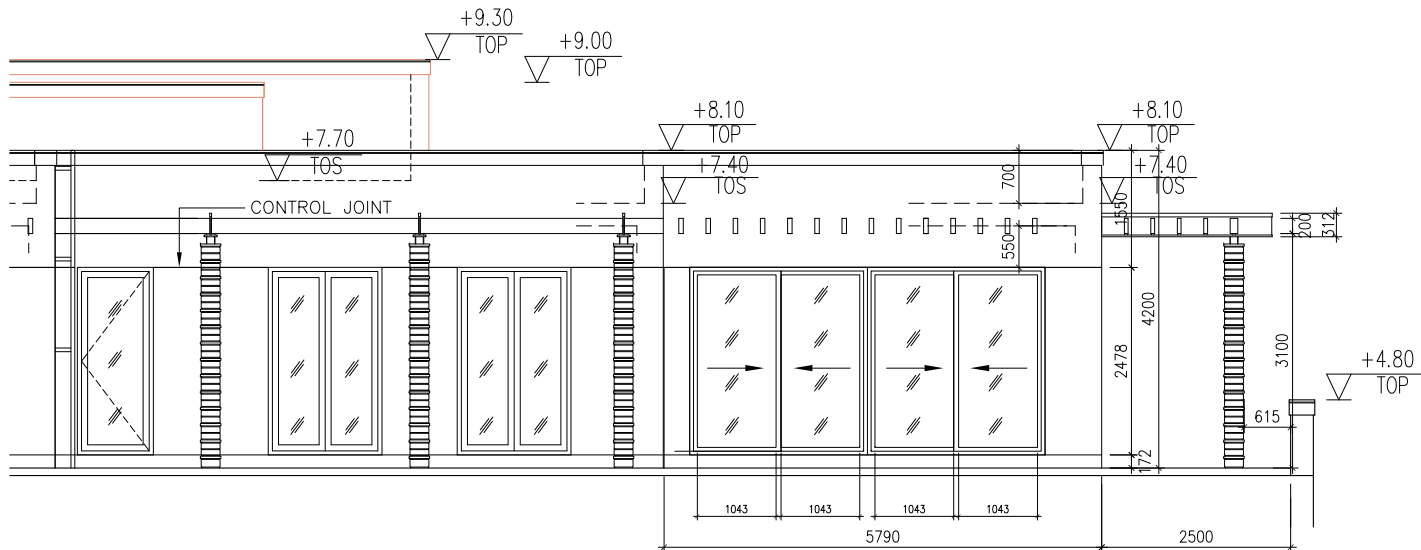
SOUTH ELEVATION OPTION-3
