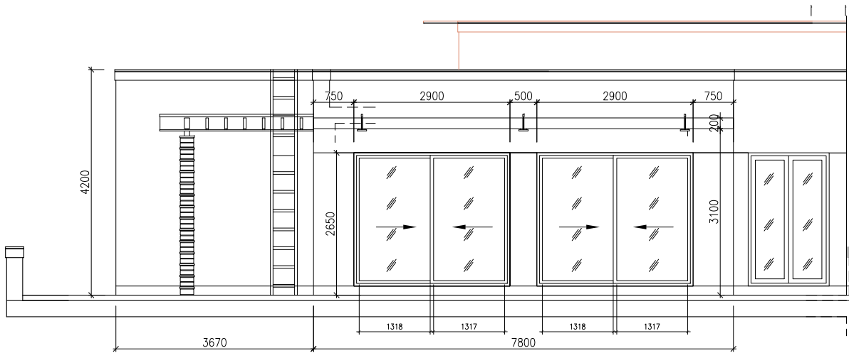
EAST ELEVATION (OPTION-3)
