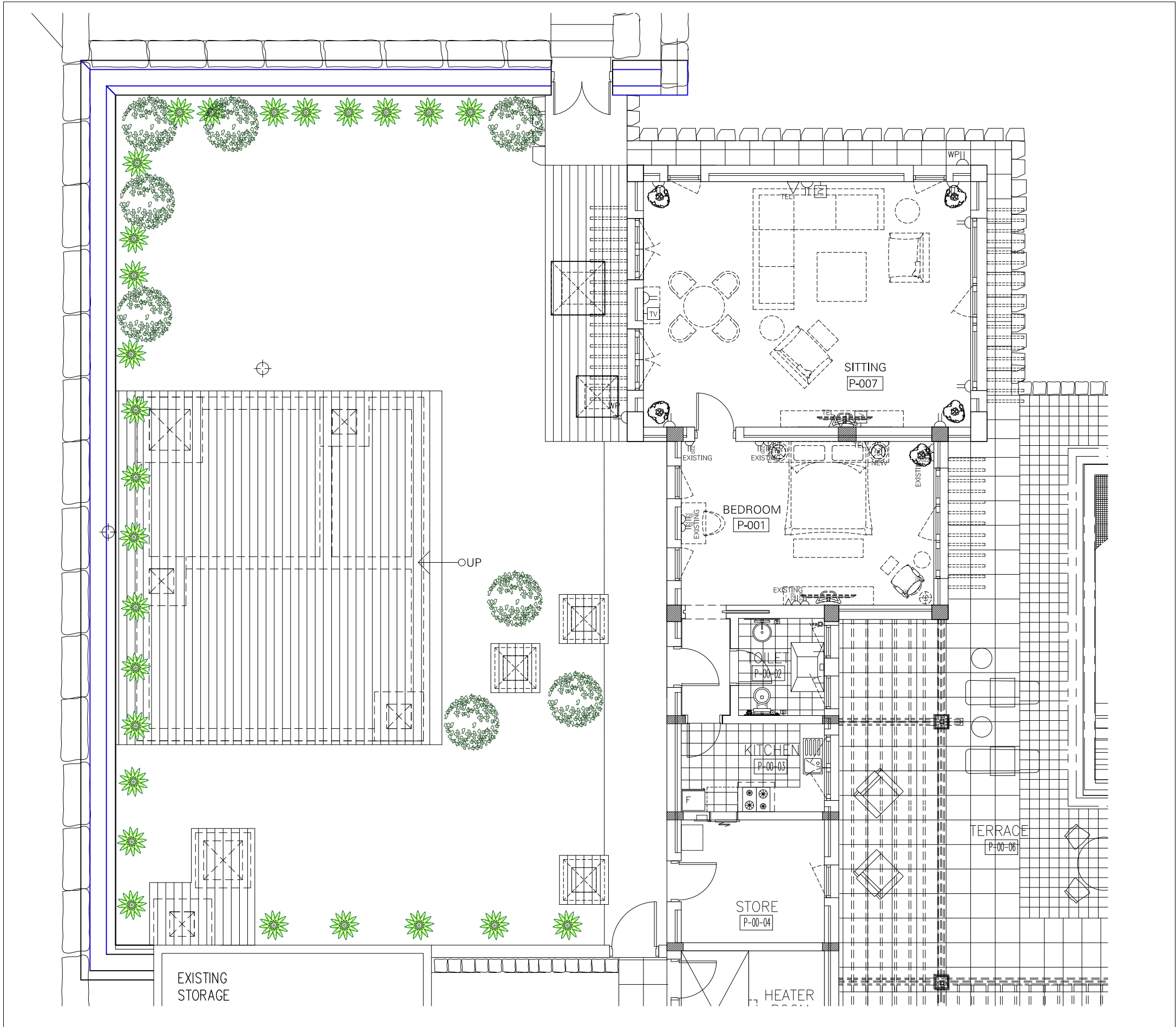
POWER + COMMUNICATION LAYOUT SCALE 1:50
