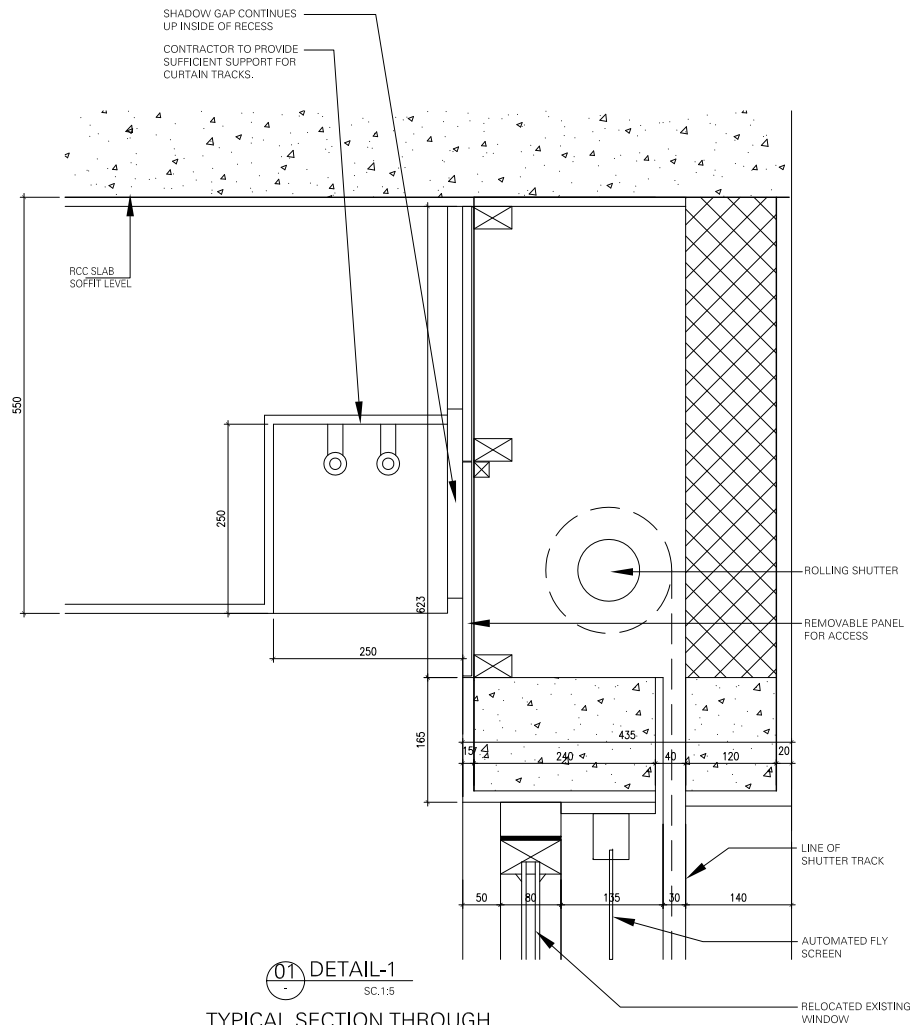
TYPICAL SECTION THROUGH SHUTTER AND CURTAIN BOX
