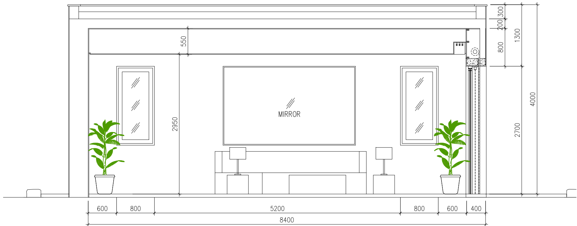
TYPICAL SECTION SC.1:25
