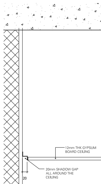
01 DETAIL-2 SC.1:5
