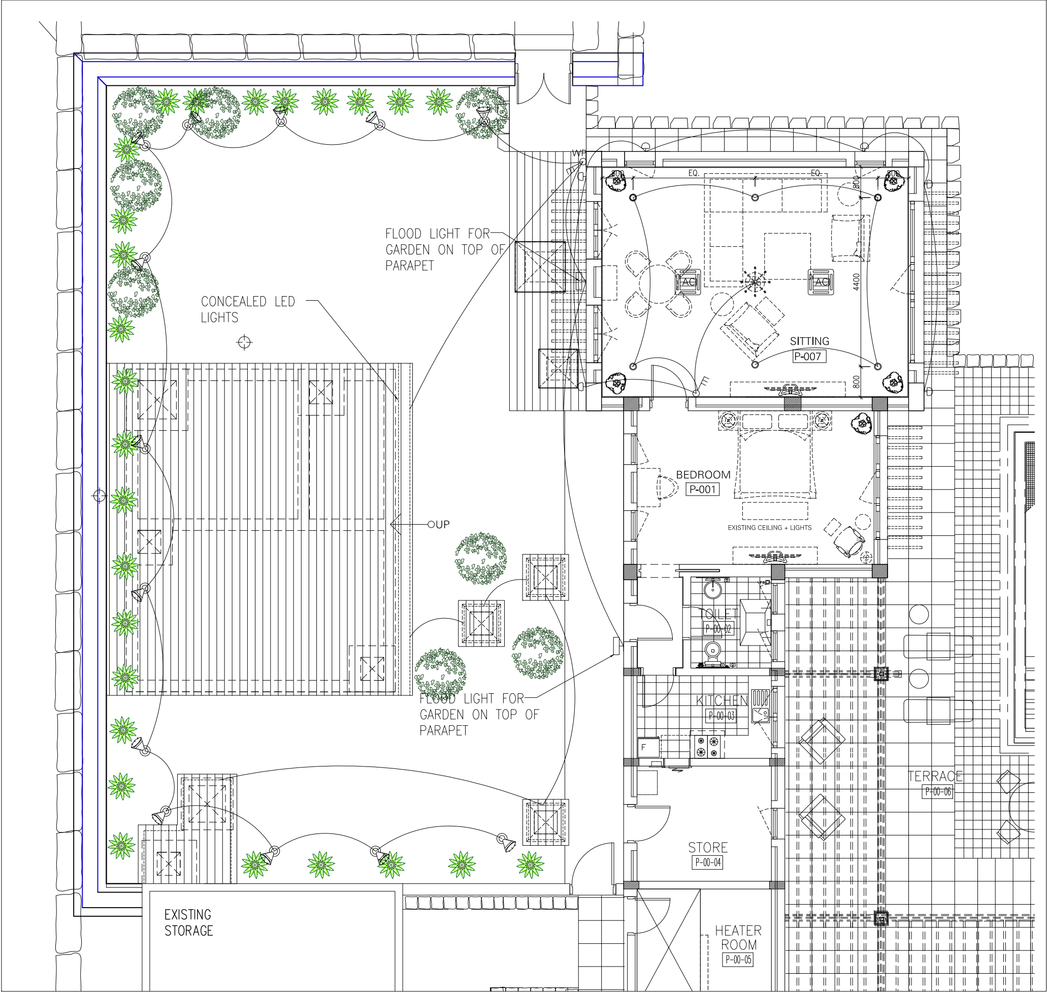
LIGHTING LAYOUT SCALE 1:50
