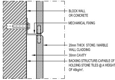
12 STONE / MARBLE WALL CLADDING TYPICAL DETAIL
