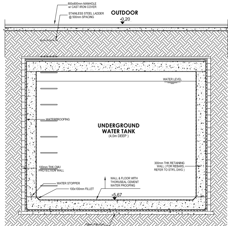
19 UNDERGROUND WATER TANK TYPICAL DETAIL
