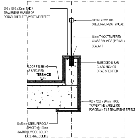
15 GLASS RAILING ARCH'L DETAIL
