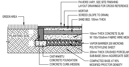
11 DETAIL AT GREEN AREA SECTION TYPICAL DETAIL
