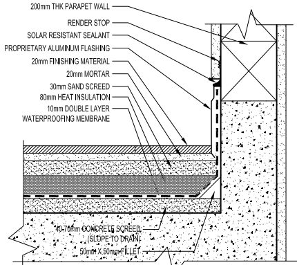
10 PARAPET WALL TYPICAL DETAIL
