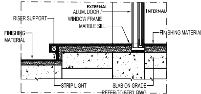
14 GROUND FLOOR WINDOW STEP ARCH'L DETAIL
