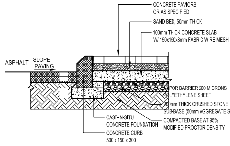
09 SIDEWALK SECTION DETAIL TYPICAL DETAIL
