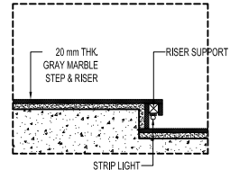
13 OUTDOOR STEP ARCH'L DETAIL
