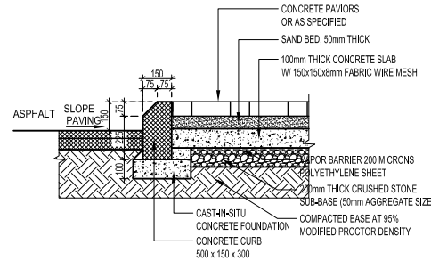
SIDEWALK SECTION DETAIL
