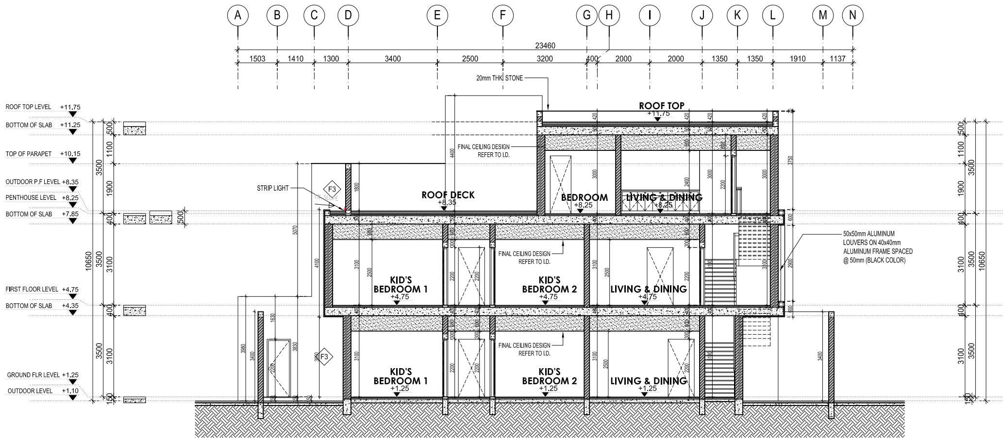
S1 CROSS SECTION AR-07 SCALE: 1:100
