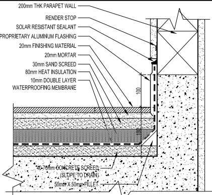
PARAPET WALL TYPICAL DETAIL
