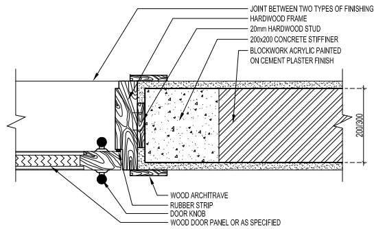
INTERNAL DOOR TYPICAL DETAIL
