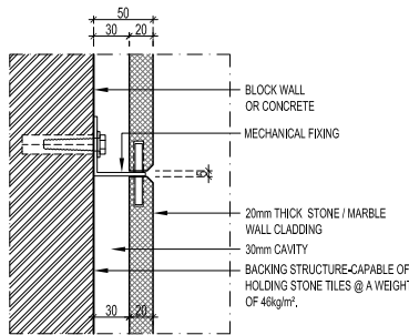
STONE / MARBLE WALL CLADDING TYPICAL DETAIL
