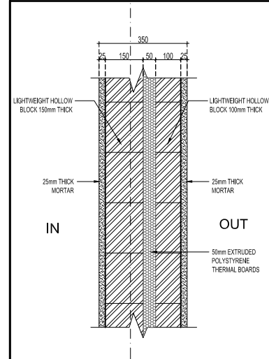
WALL SECTION DETAIL WALL THK = 350mm U VALUE FOR THE WALL=0.382
