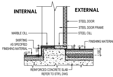
ROOF DOOR THRESHOLD
