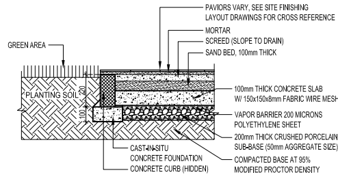
DETAIL AT GREEN AREA SECTION
