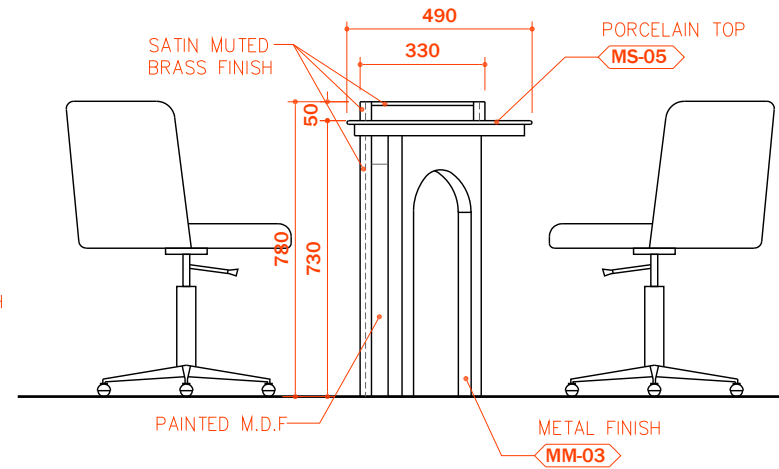
B SIDE ELEVATION SCALE 1:20
