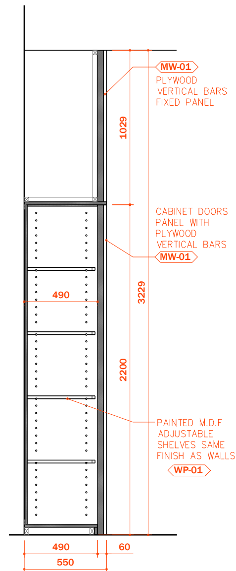
02 SECTION - SCALE 1:25
