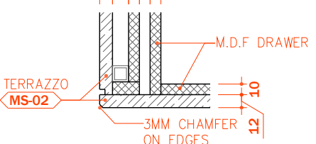
04 SPOT DETAIL SCALE 1:5
