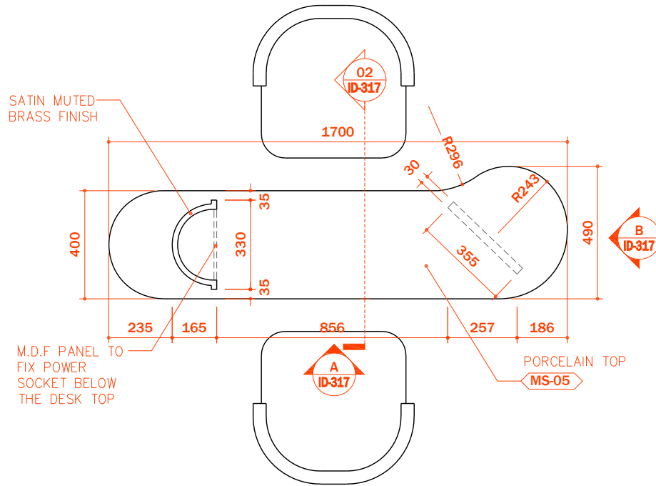
01 MANICURE DESK PLAN SCALE 1:20
