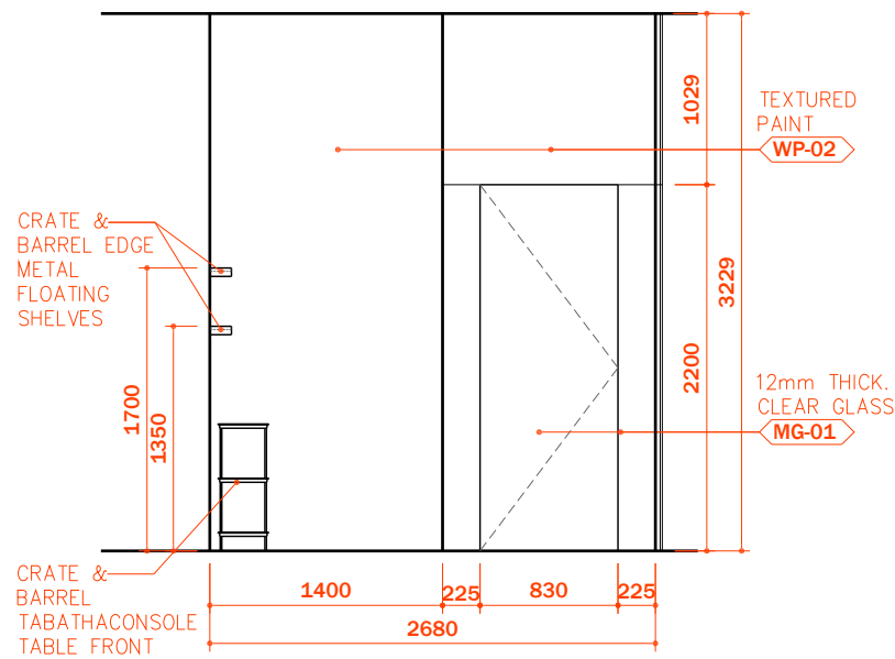
03 ELEVATION
