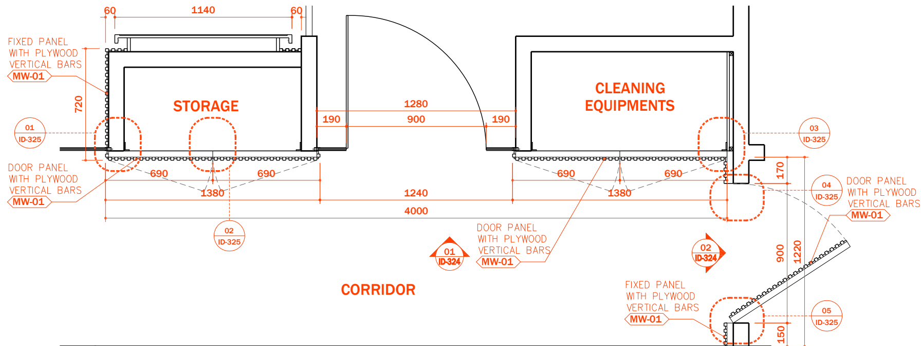
A CORRIDOR STORAGE AND WASHROOM DOOR PLAN SCALE 1:25
