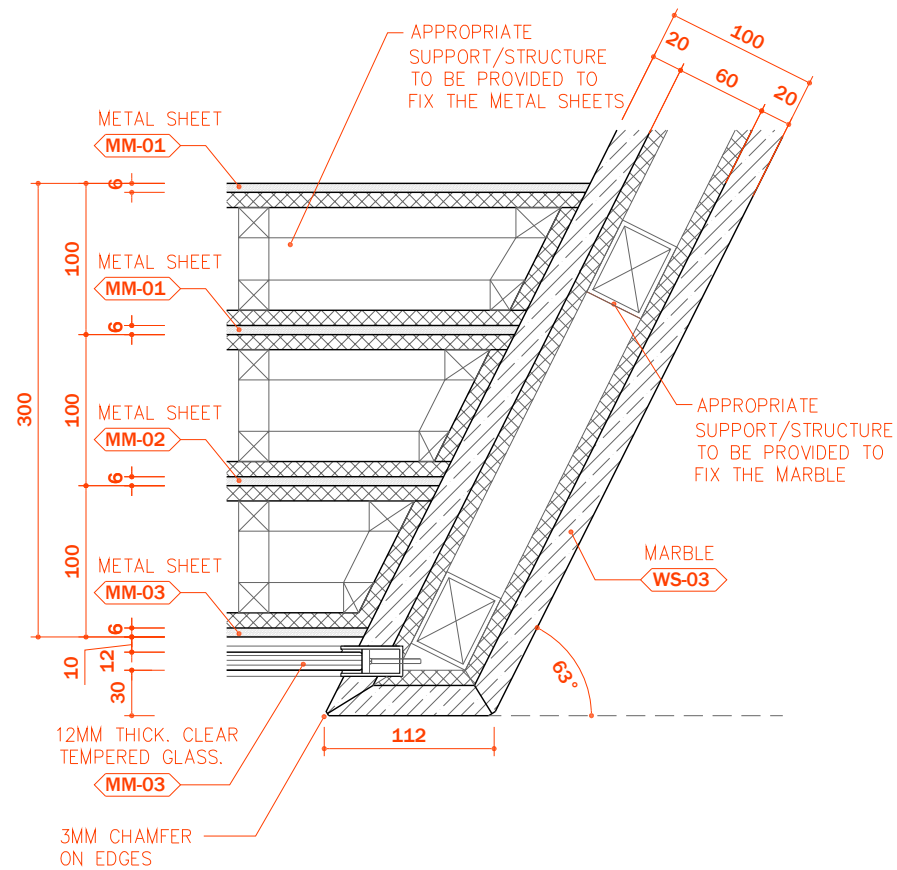
SCALE 1:5
