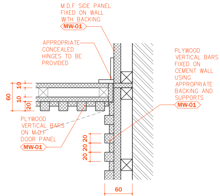
03 SPOT DETAIL SCALE 1:5
