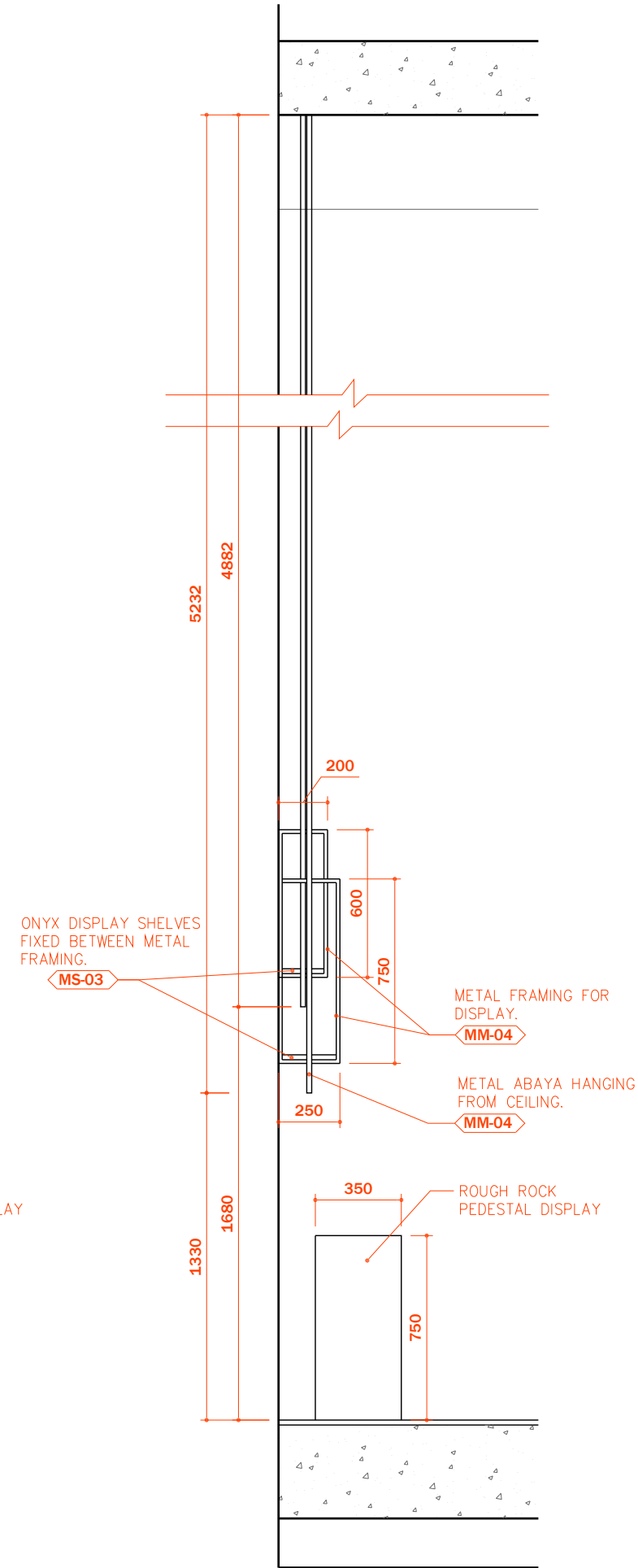
03 SECTION SCALE 1:25
