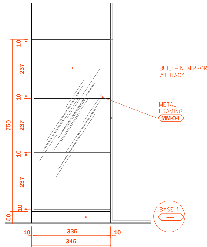
04 SPOT DETAIL SCALE 1:10
