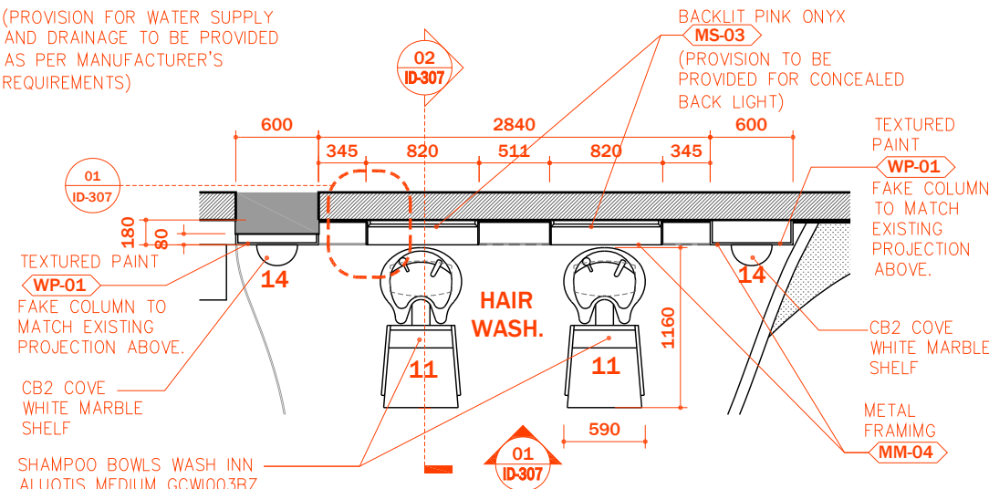
HAIR WASH AREA PLAN SCALE 1:50
