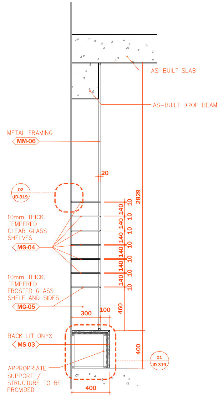
02 SECTION SCALE 1:25
