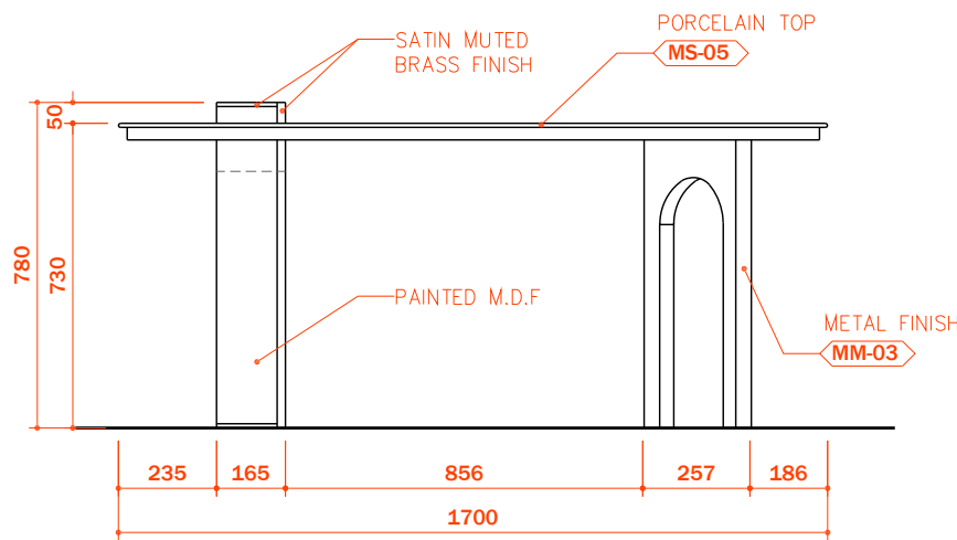
A MANICURE DESK ELEVATION SCALE 1:20
