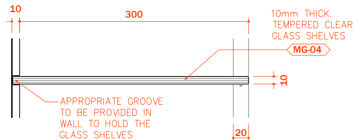
02 SPOT DETAIL SCALE 1:5
