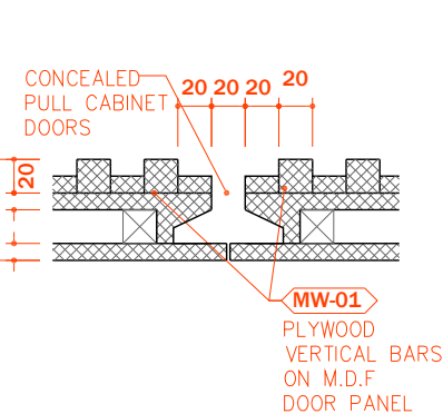
04 SPOT DETAIL SCALE 1:5
