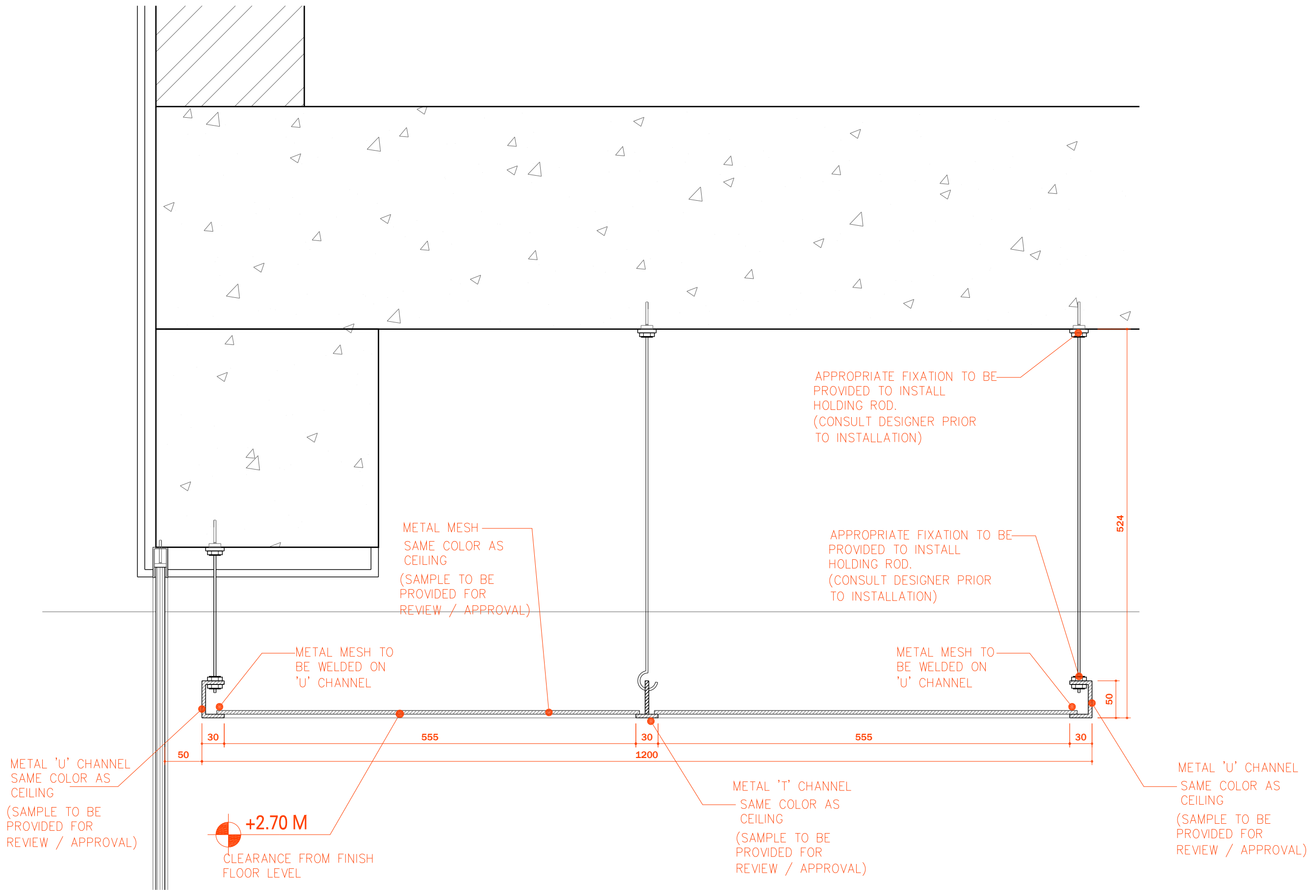
01 METAL MESH CEILING SECTION DETAIL SCALE 1:5
