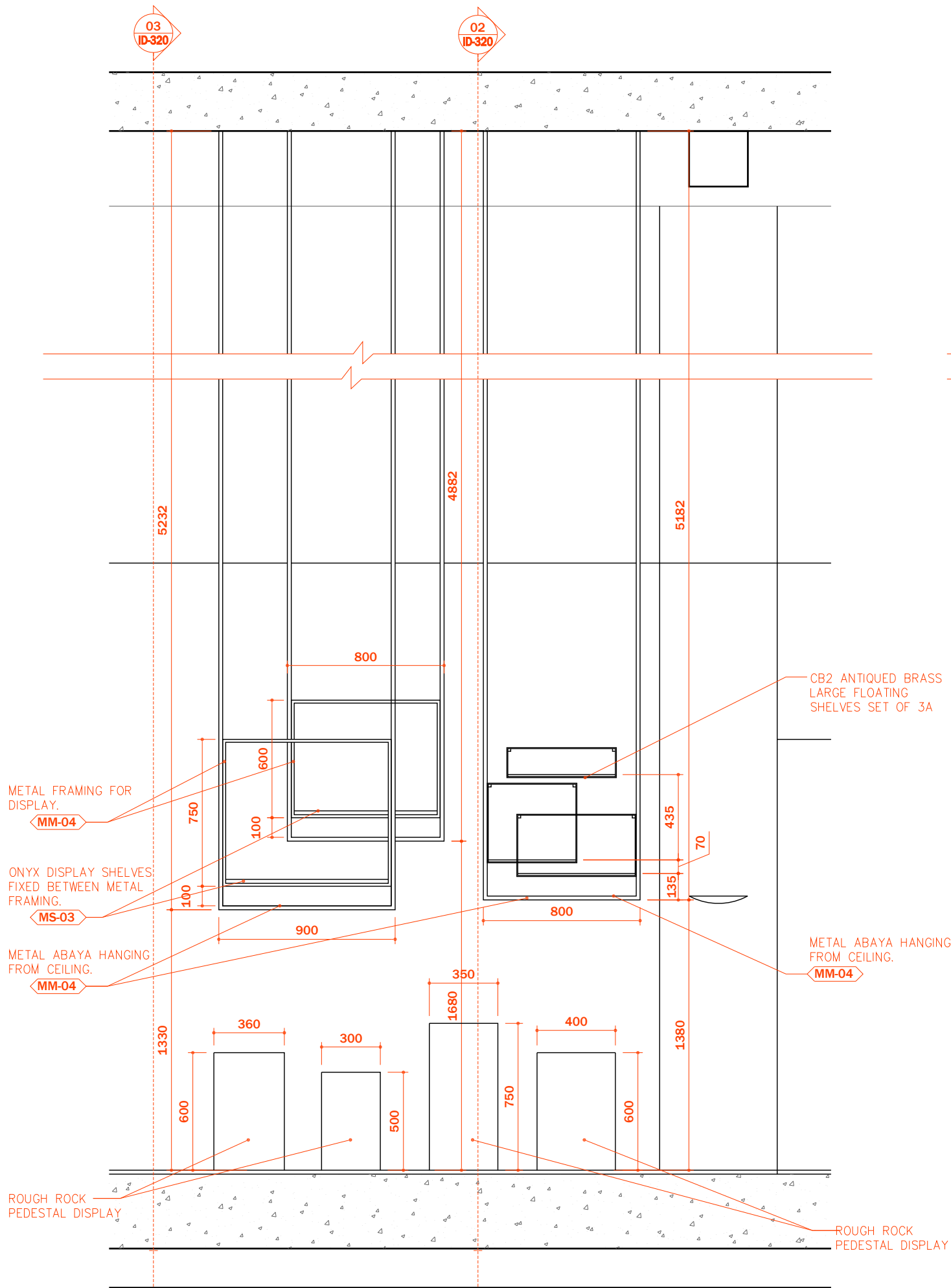
01 CEILING HUNGED DISPLAY + ABAYA HANGING ELEVATION SCALE 1:25
