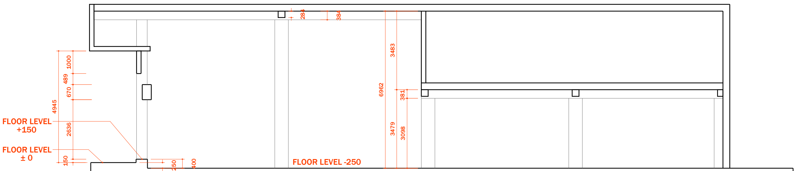
01 AS-BUILT SECTION SCALE 1:100
