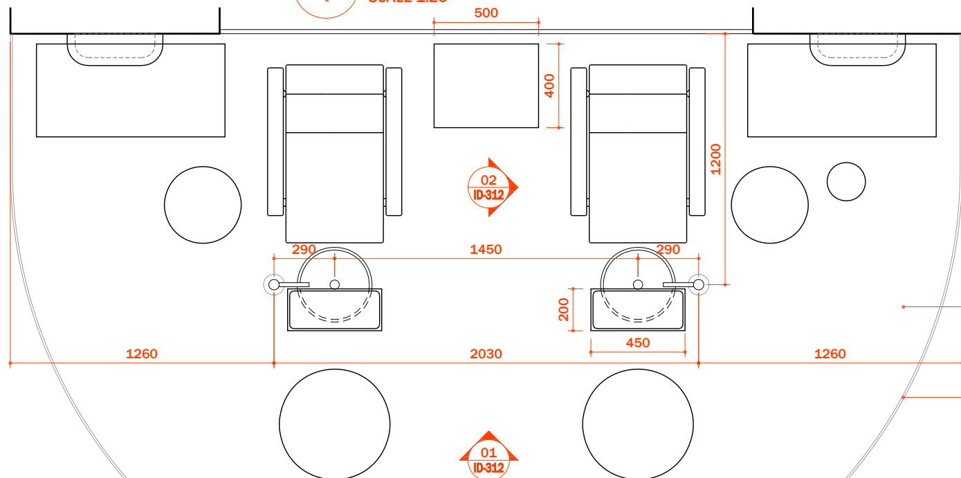
01 PEDICURE STATION PLAN SCALE 1:25
