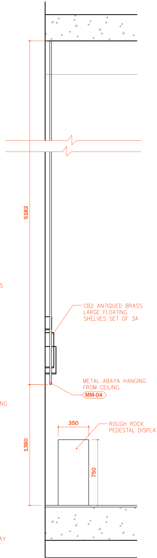
02 SECTION SCALE 1:25
