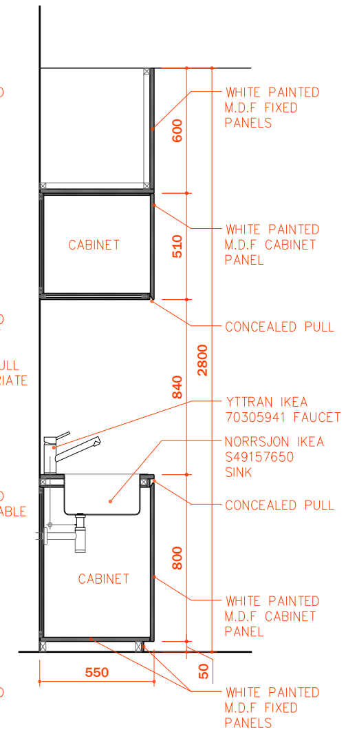
04 SECTION SCALE 1:25
