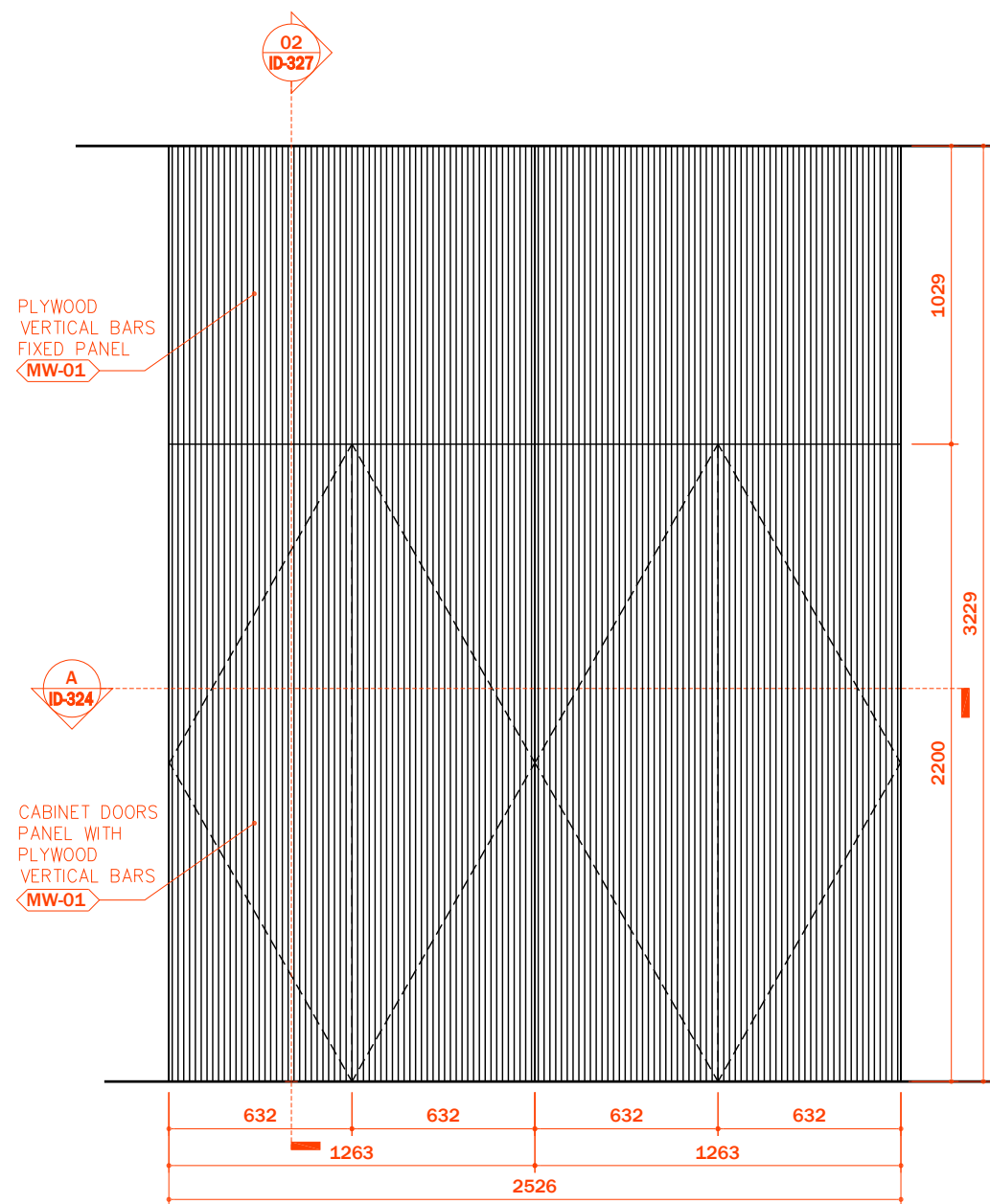
01 ELEVATION SCALE 1:25
