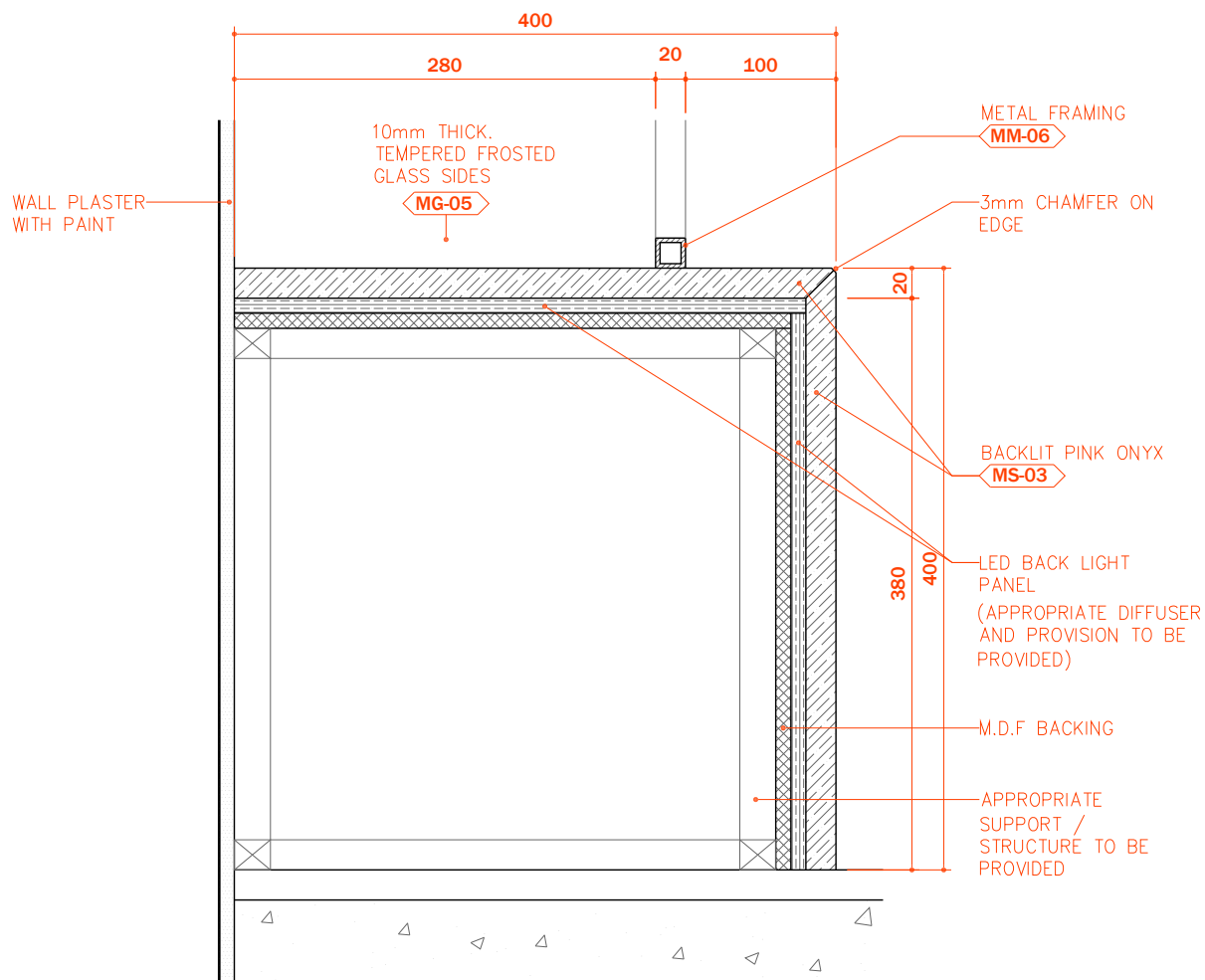
01 SPOT DETAIL SCALE 1:5
