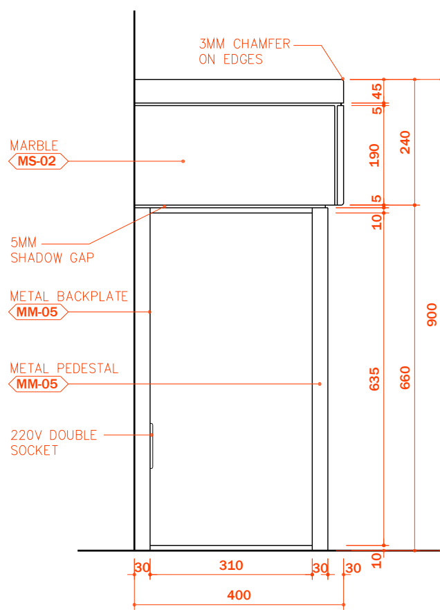
B DRAWER UNIT ELEVATION SCALE 1:10
