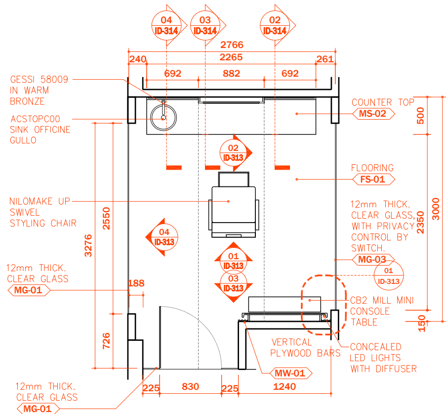
MAKE UP ROOM PLAN
