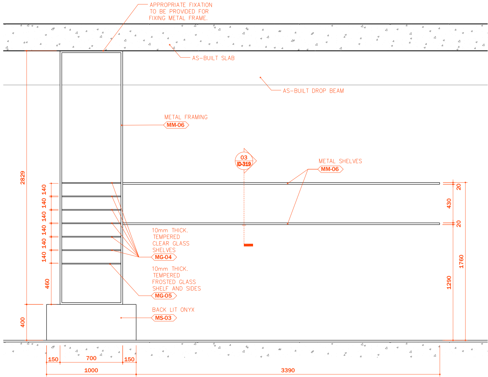
A DISPLAY / SHELVING ELEVATION SCALE 1:25
