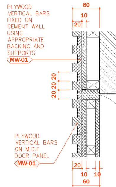
04 SPOT DETAIL SCALE 1:5
