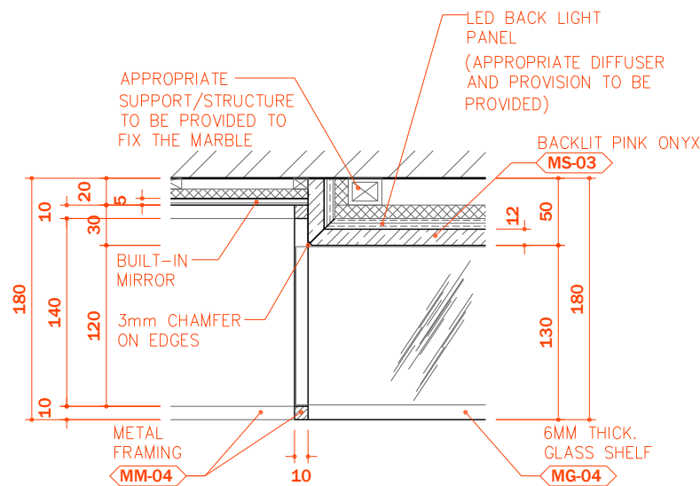
01 SPOT DETAIL SCALE 1:5
