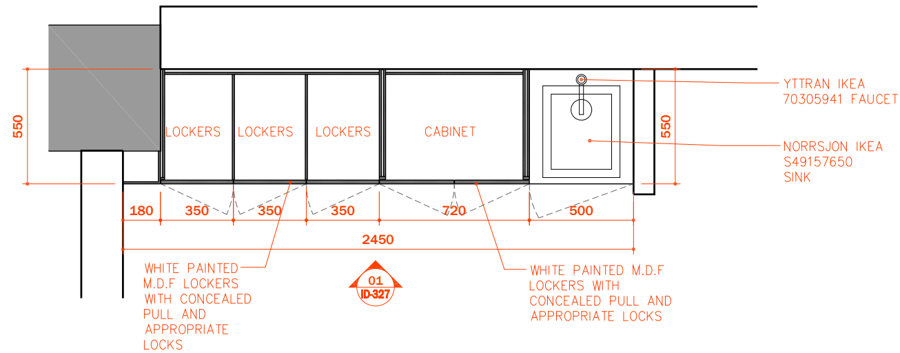
A STAF ROOM BUILT-IN CABINET PLAN SCALE 1:25
