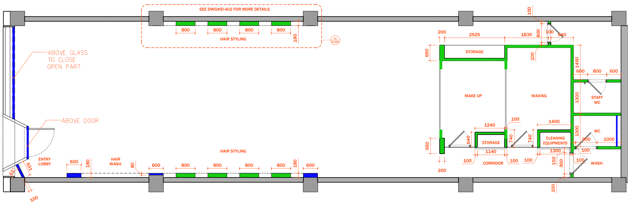
- DRY WALL LAYOUT SCALE 1:75
