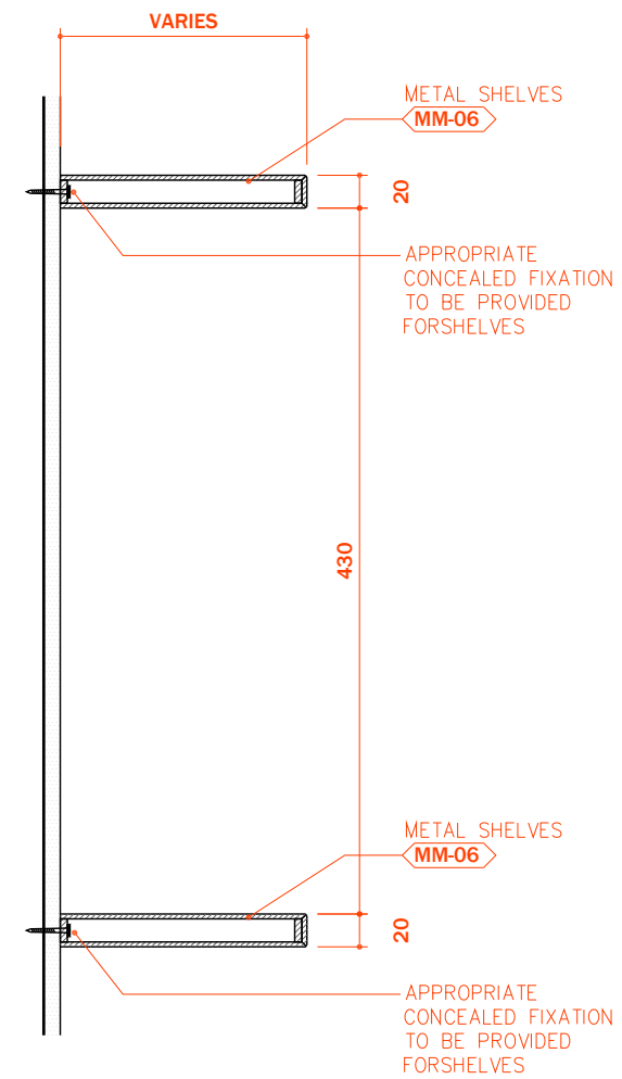
03 SPOT DETAIL SCALE 1:5
