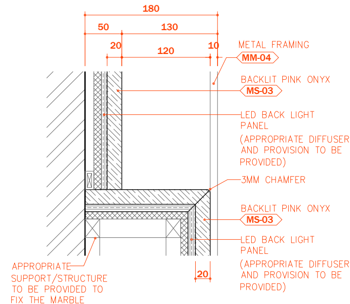
03 SPOT DETAIL SCALE 1:5
