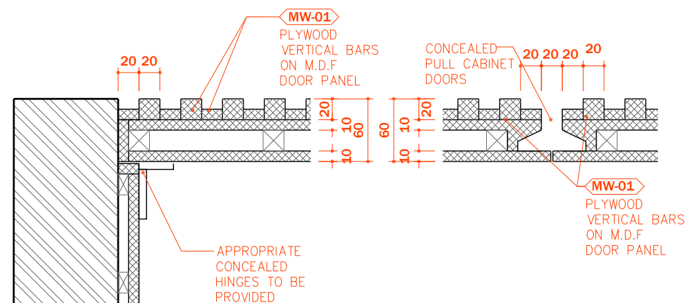
03 SPOT DETAIL SCALE 1:5
