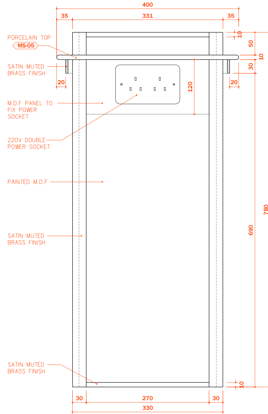
02 SECTION SCALE 1:20
