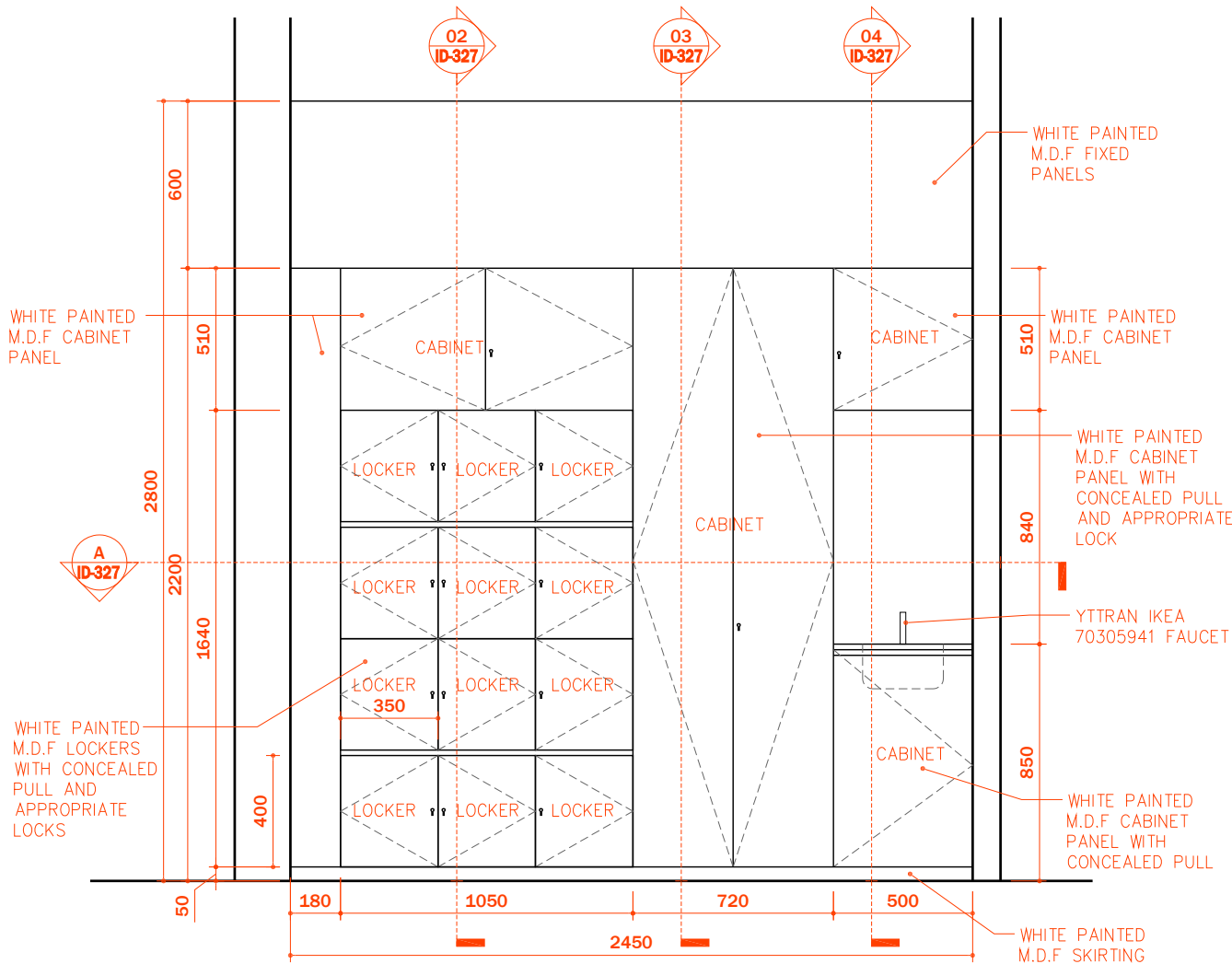
01 STAF ROOM BUILT-IN CABINET ELEVATION SCALE 1:25
