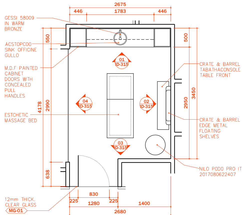
WAXING ROOM PLAN
