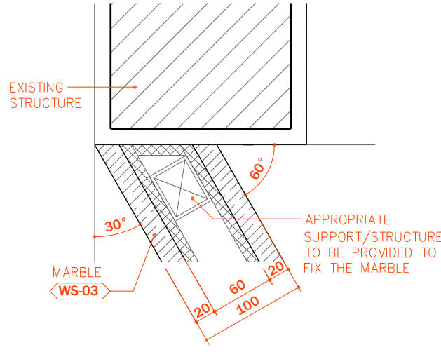
SCALE 1:5
