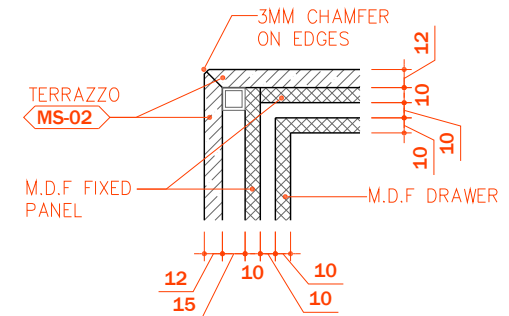
05 SPOT DETAIL SCALE 1:5
