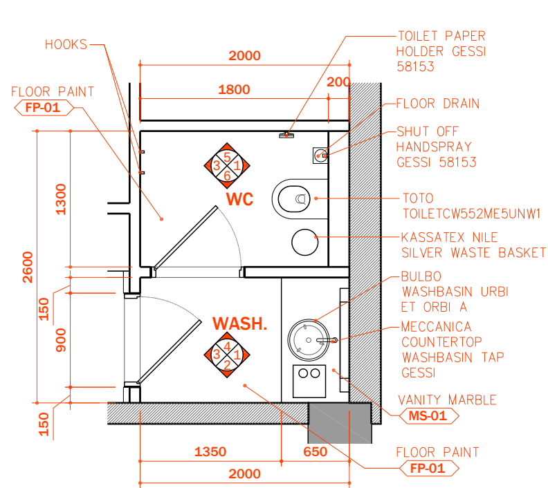
RESTROOM PLAN
