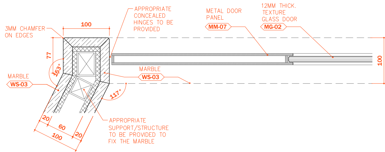
SCALE 1:5
