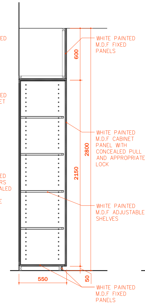
03 SECTION SCALE 1:25
