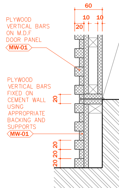
05 SPOT DETAIL SCALE 1:5
