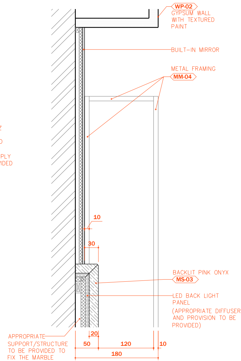
02 SPOT DETAIL SCALE 1:5
