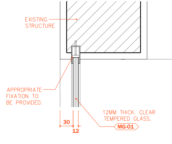
SCALE 1:5
