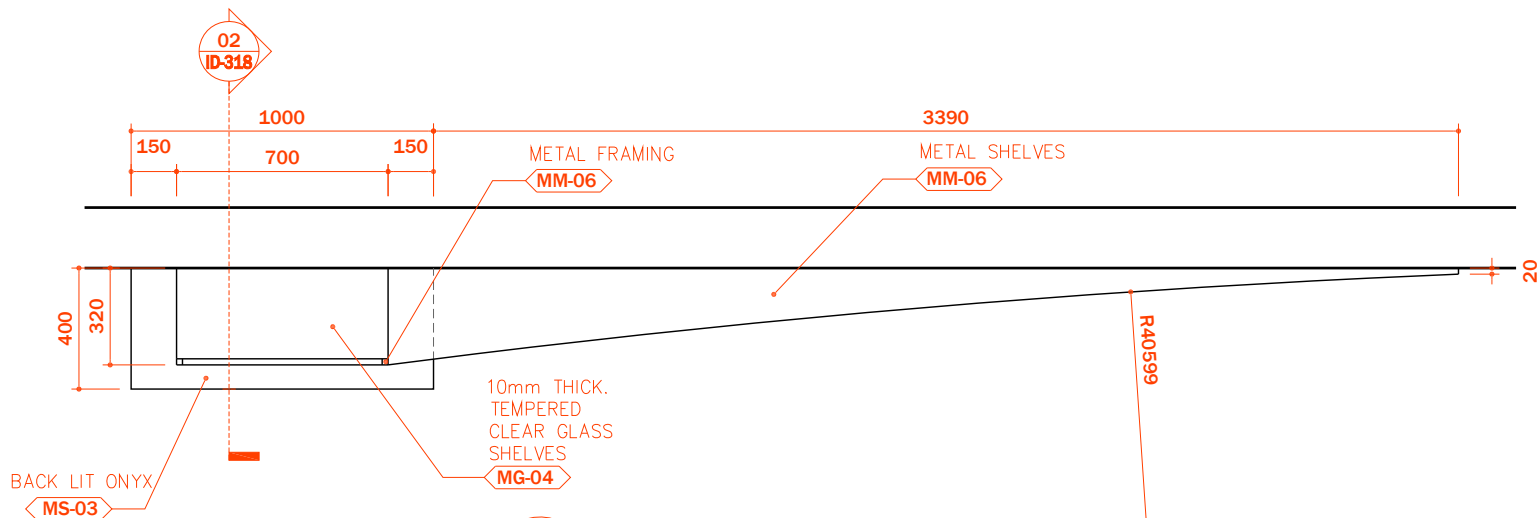
01 DISPLAY / SHELVING PLAN SCALE 1:25
