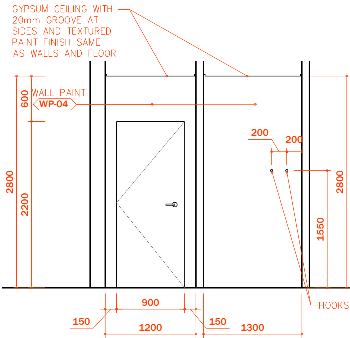
03 ELEVATION
