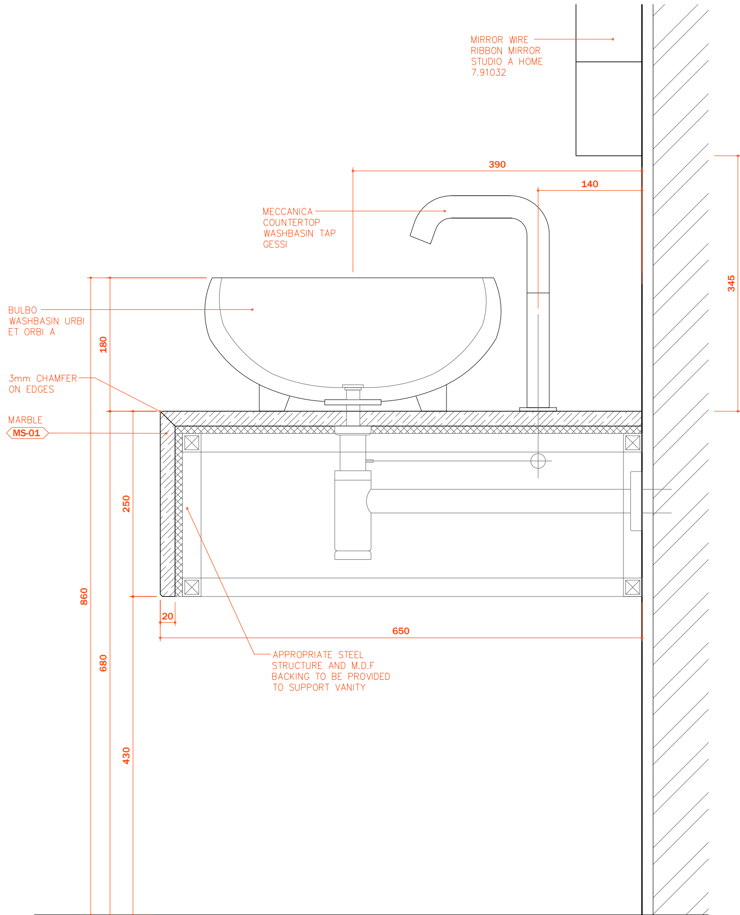
01 VANITY DETAIL SCALE 1:5
