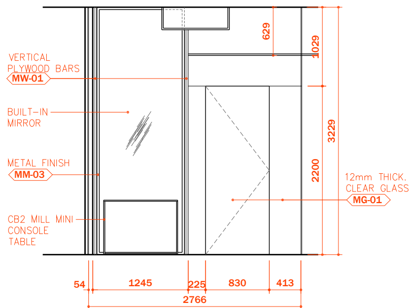
03 ELEVATION
