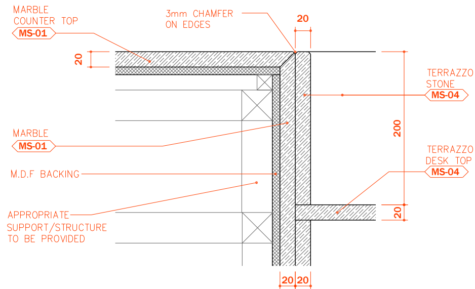
03 COLOR BAR DETAIL SCALE 1:5
