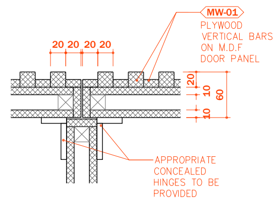
05 SPOT DETAIL SCALE 1:5
