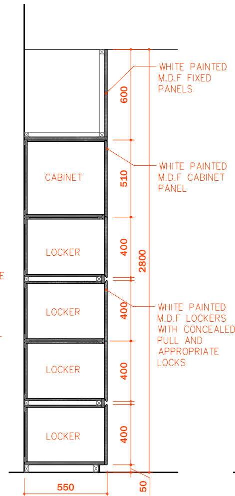
02 SECTION SCALE 1:25
