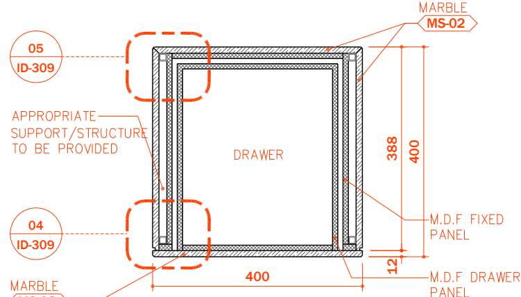
01 SECTION DETAIL SCALE 1:10
