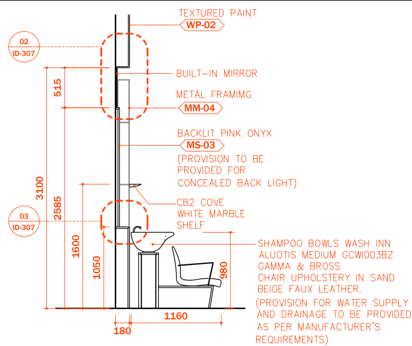
02 SECTION SCALE 1:50
