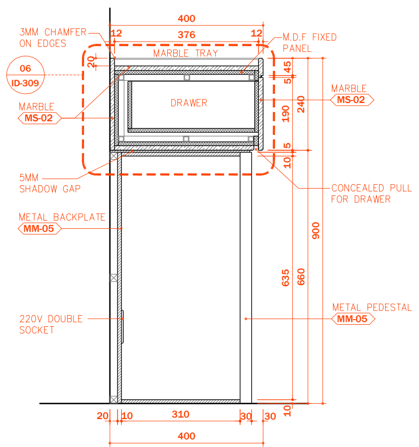
02 SECTION SCALE 1:10
