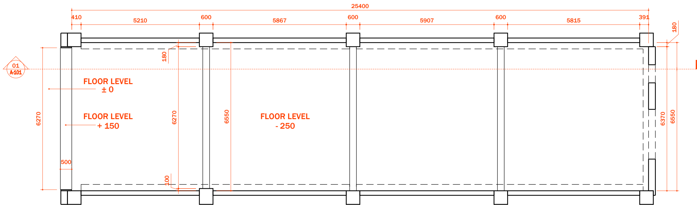
AS-BUILT LAYOUT SCALE 1:100
