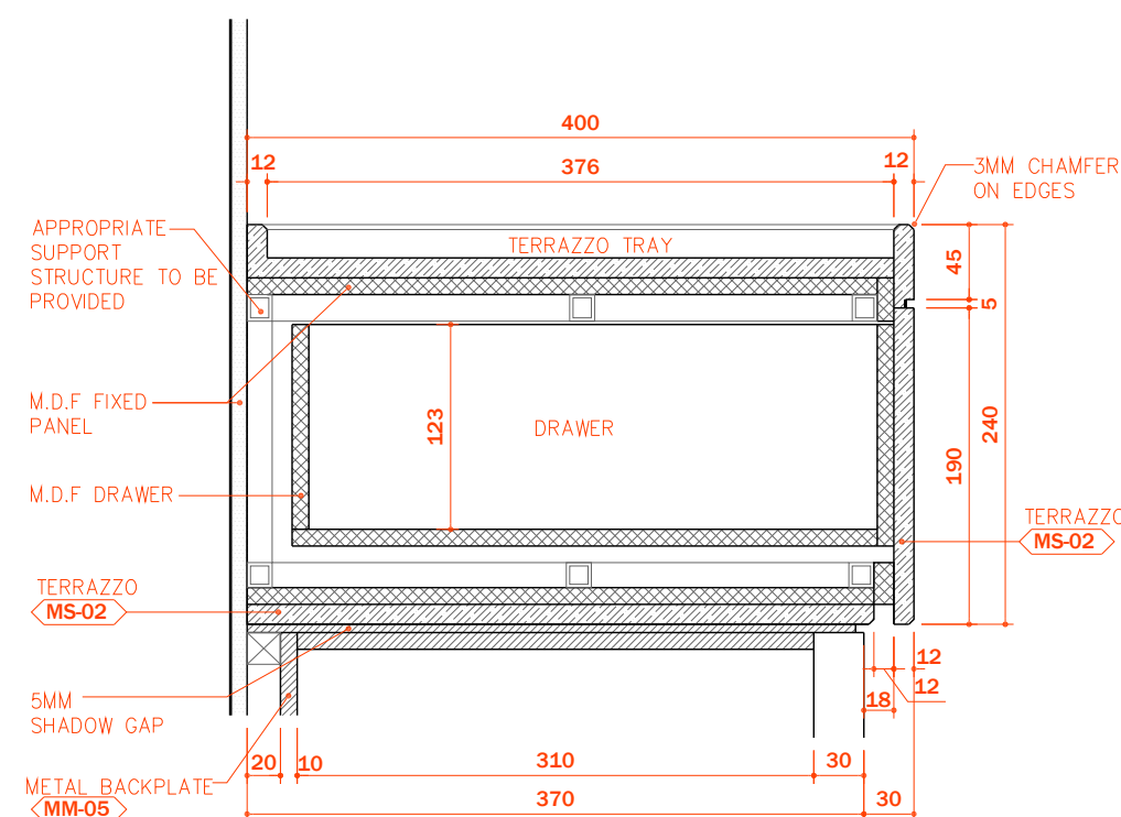
06 SPOT DETAIL SCALE 1:5
