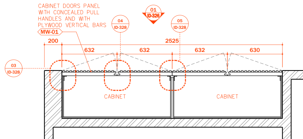
A CORRIDOR CABINET PLAN SCALE 1:25
