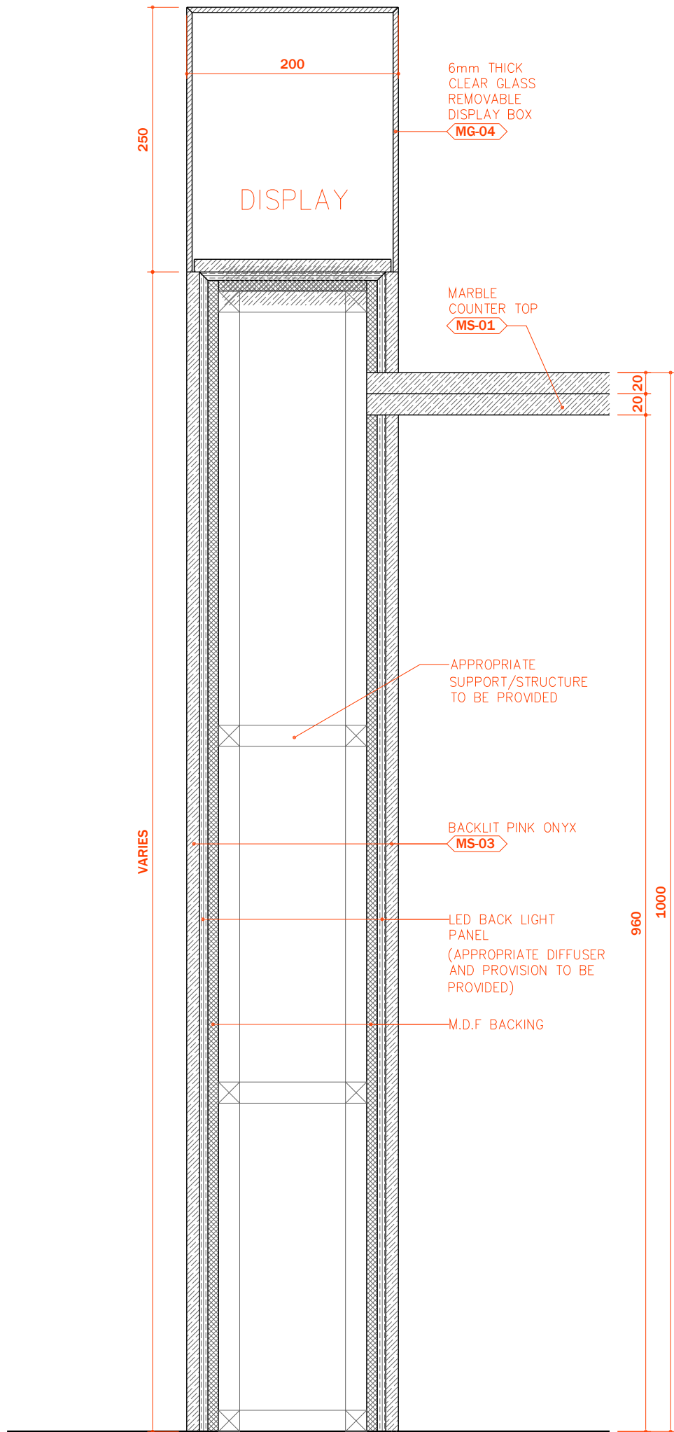
01 DISPLAY BOX DETAIL SCALE 1:5
