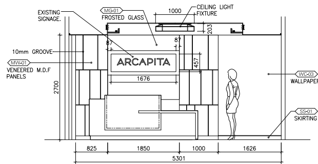
1 ELEVATION SCALE 1:50
