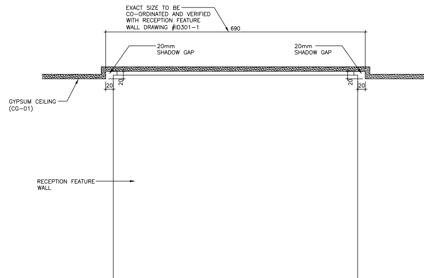
06 DETAIL AT RECEPTION FEATURE WALL SC. 1:5
