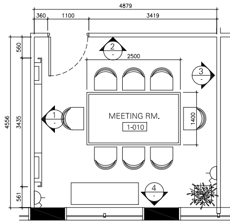
MEETING ROOM (1-010) PLAN SCALE 1:50
