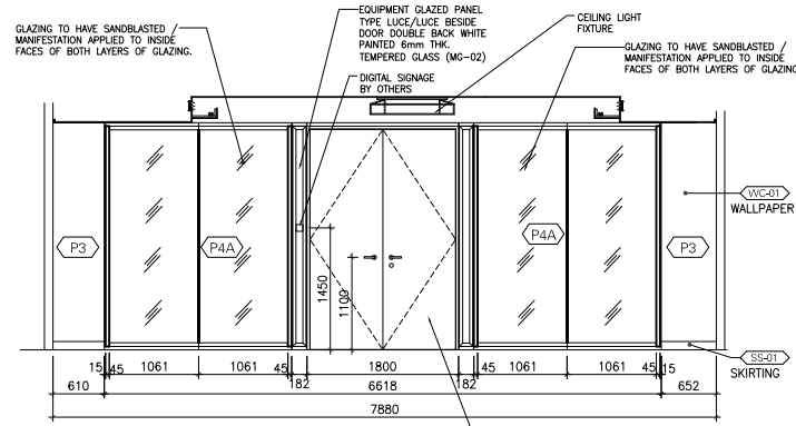
4 ELEVATION SCALE 1:50
