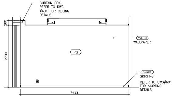
4 ELEVATION SCALE 1:50
