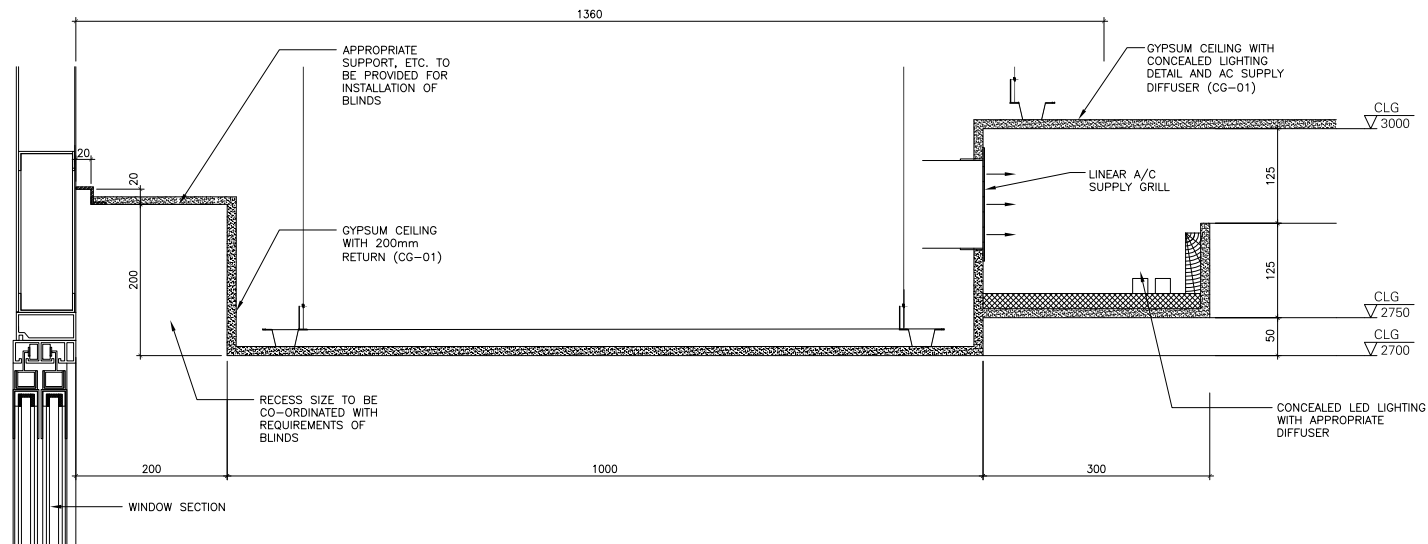
02 TYPICAL GYPSUM CEILING DETAIL WITH CONCEALED LED LIGHT AND CURTAIN BOX @ MEETING ROOMS SC. 1:5
