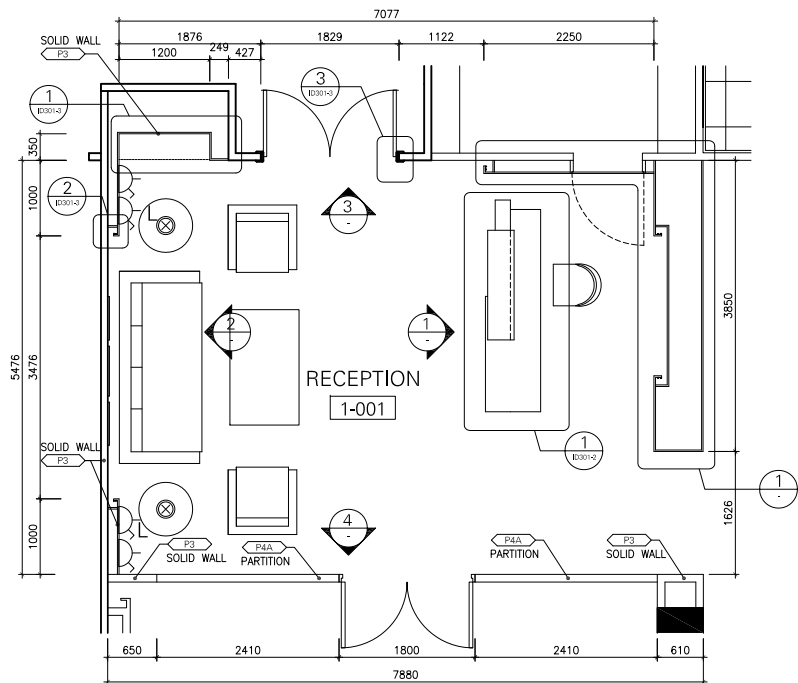
1 RECEPTION PLAN SCALE 1:50
