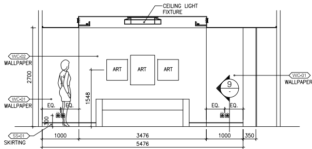
2 ELEVATION SCALE 1:50
