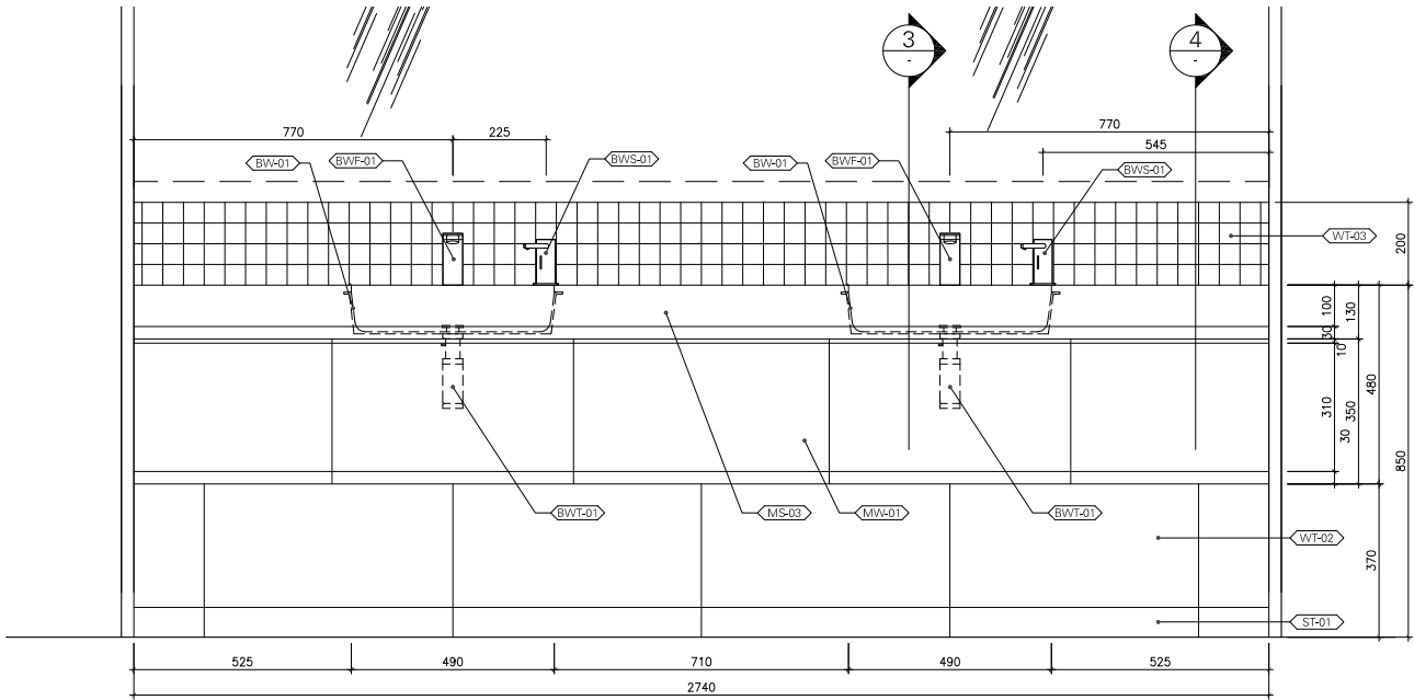
2 VANITY ELEVATION SCALE 1:10
