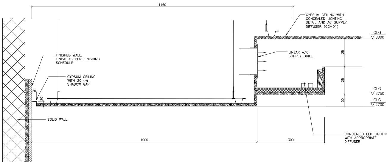
03 TYPICAL GYPSUM CEILING DETAIL WITH CONCEALED LED LIGHT @ RECEPTION SC. 1:5
