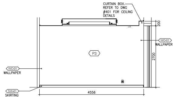
3 ELEVATION SCALE 1:50
