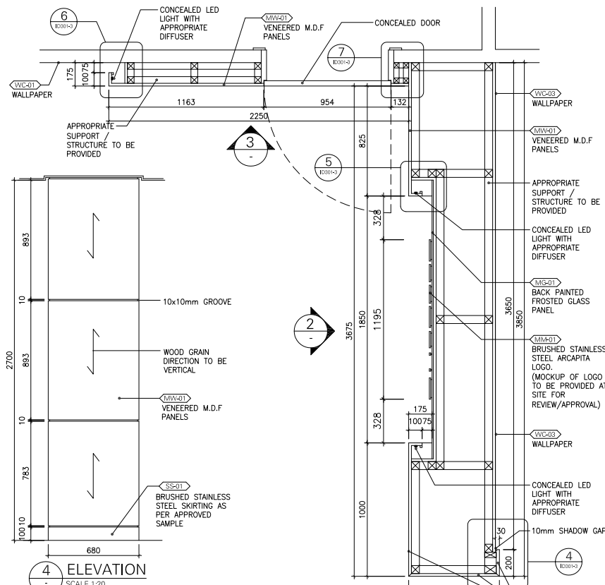
1 FEATURE WALL SECTION PLAN SCALE 1:20
