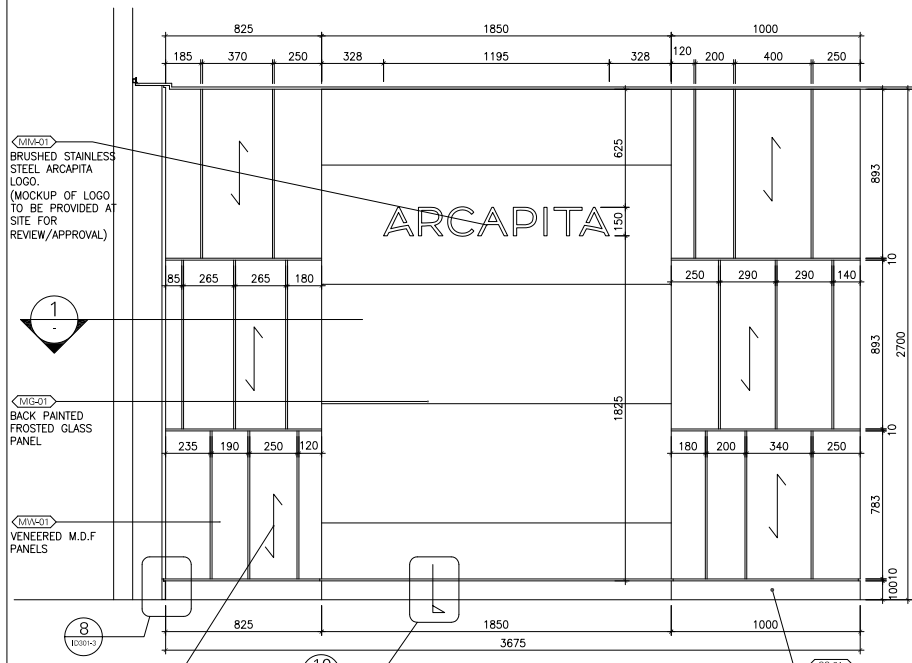
2 ELEVATION SCALE 1:20
