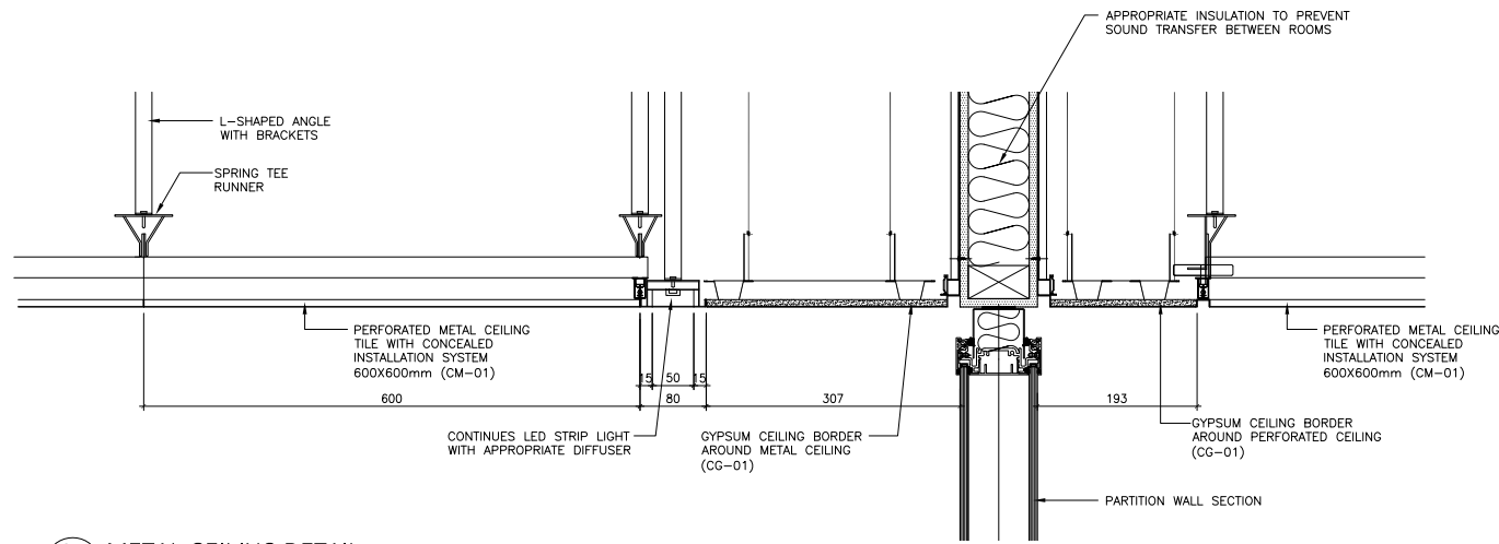
01 METAL CEILING DETAIL SC. 1:5
