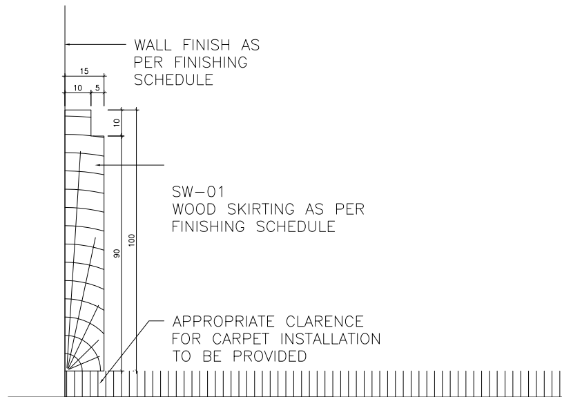
05 TYPICAL WOOD SKIRTING DETAIL (SW-01) SC: 1:1 ALL AREAS (EXCEPT RECEPTION, KITCHENETTE AND RESTROOM)
