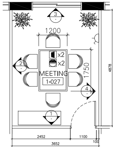
MEETING ROOM (1-027) PLAN SCALE 1:50
