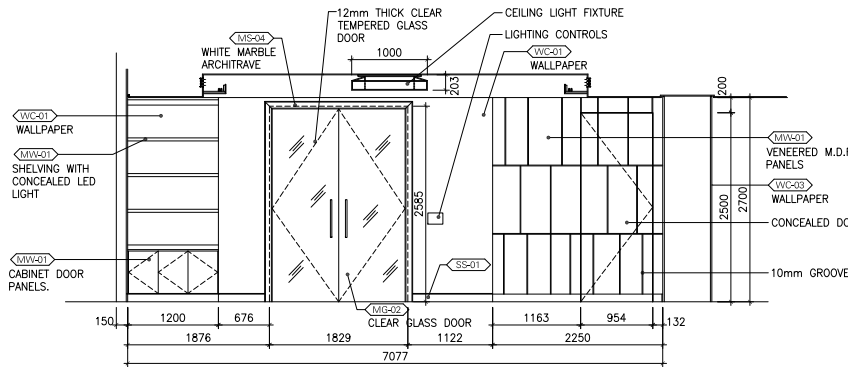
3 ELEVATION SCALE 1:50
