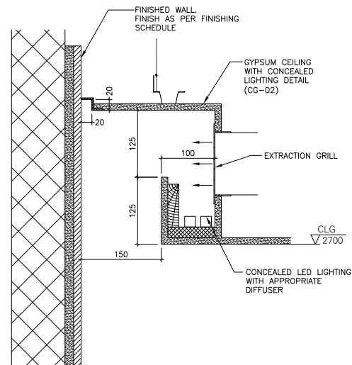
05 CEILING DETAIL WITH CONCEALED LED LIGHTS @ RESTROOM SC. 1:5
