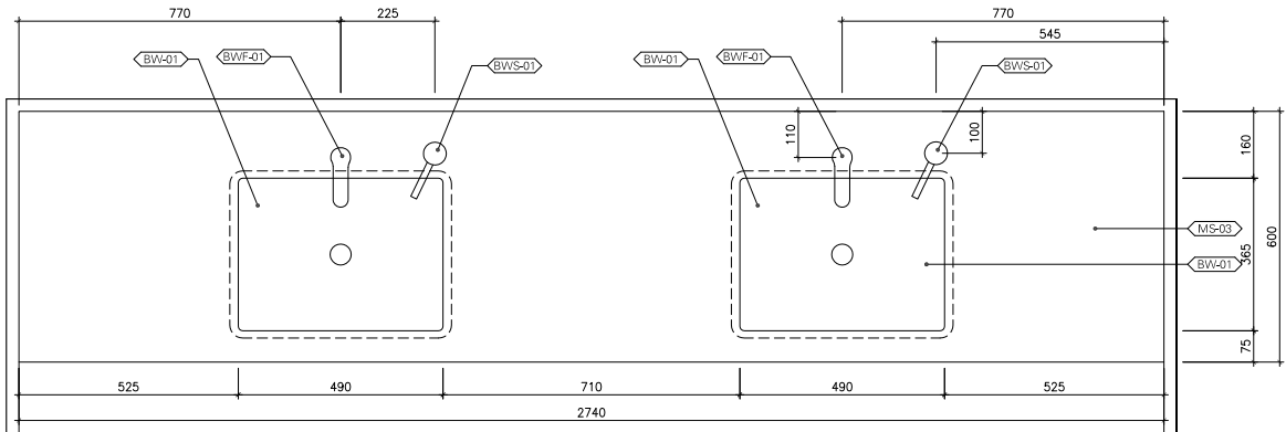
1 VANITY PLAN SCALE 1:10
