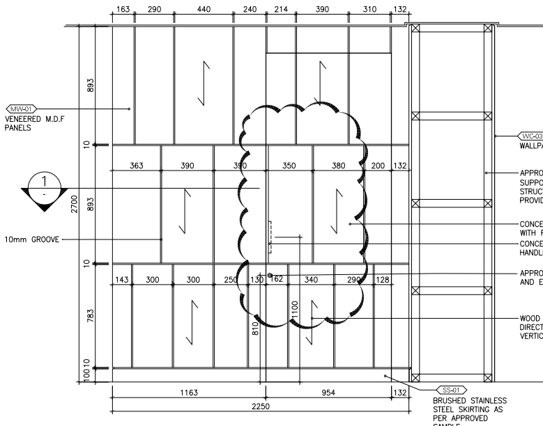
3 ELEVATION SCALE 1:20
