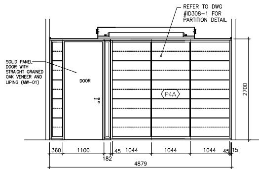
2 ELEVATION SCALE 1:50
