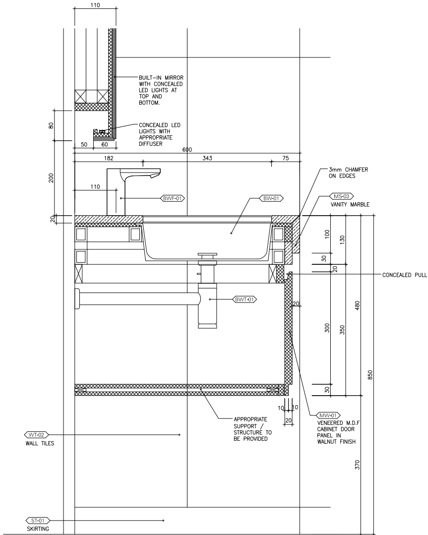
3 VANITY SECTION SCALE 1:5
