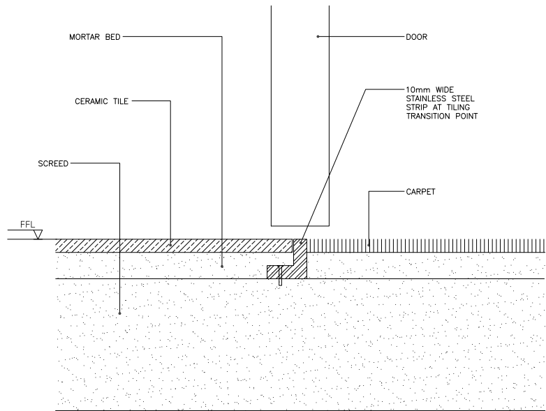
02 FLOOR TRANSITION DETAIL (CERAMIC TILE DETAIL) SC: 1:2
