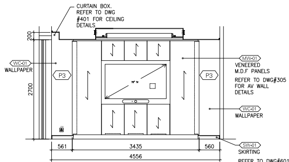
1 ELEVATION SCALE 1:50
