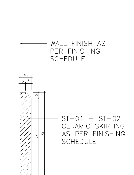
04 TYPICAL CERAMIC SKIRTING DETAIL (ST-01 + ST-02) SC: 1:1 KITCHENETTE (1-028) AND RESTROOM (1-05,1-006)
