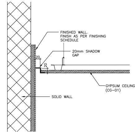
04 TYPICAL GYPSUM FLAT CEILING DETAIL SC. 1:5
