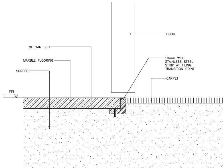
03 FLOOR TRANSITION DETAIL (MARBLE & CARPET DETAIL) SC: 1:2
