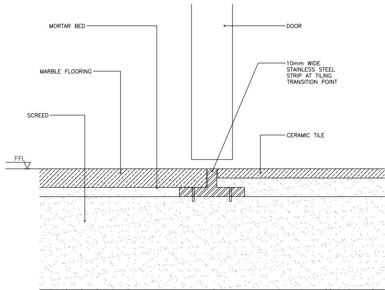
01 FLOOR TRANSITION DETAIL (MARBLE + CERAMIC TILE DETAIL) SC: 1:2
