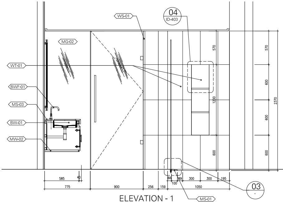
ELEVATION - 1 SCALE 1:20
