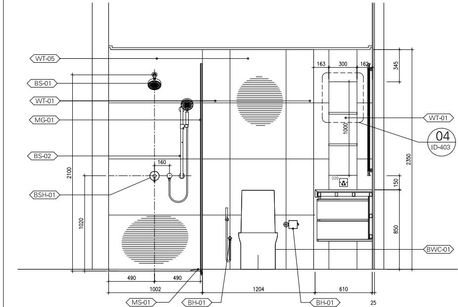
ELEVATION - 3 SCALE 1:20
