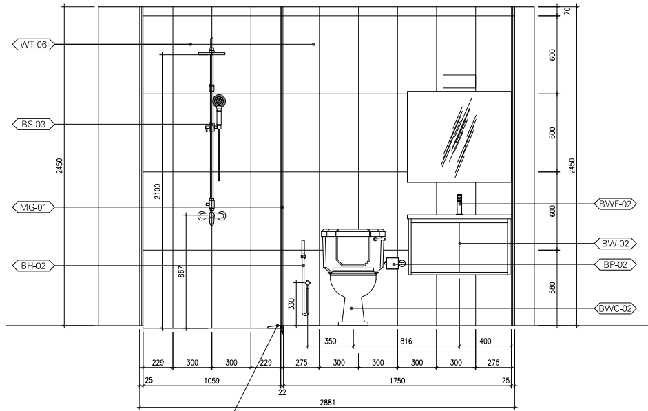
ELEVATION - 1 SCALE 1:20
