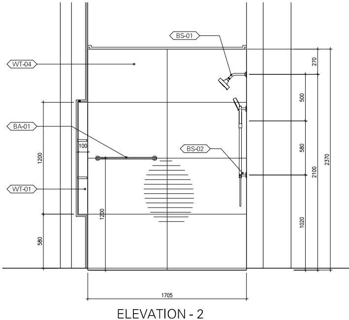
ELEVATION - 2 SCALE 1:20
