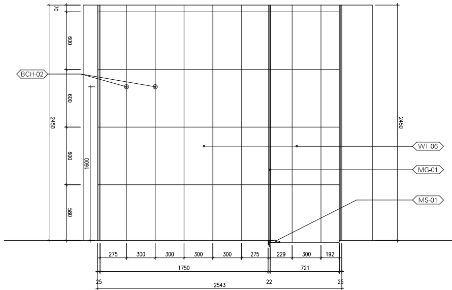
ELEVATION - 3 SCALE 1:20
