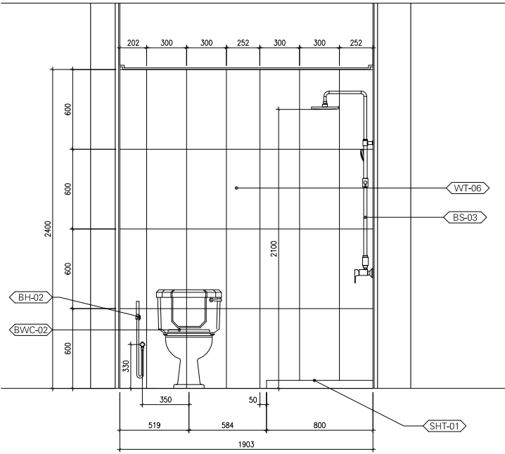
ELEVATION - 3 SCALE 1:20
