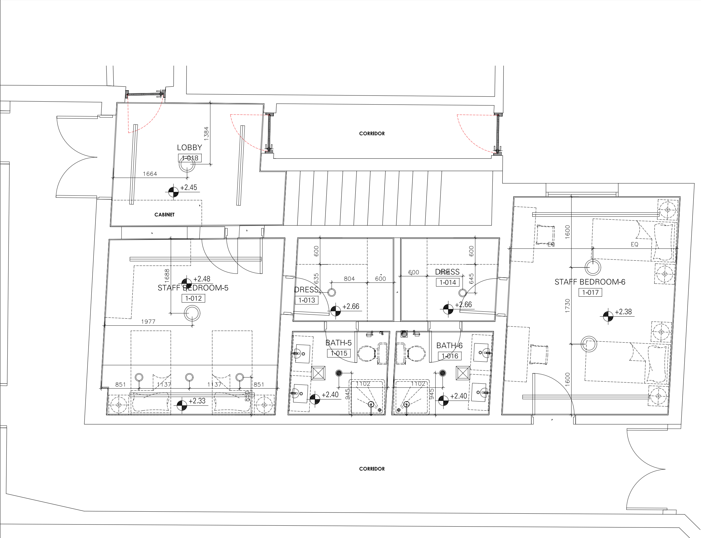
STAFF BEDROOM - 5 & 6 REFLECTED CEILING LAYOUT SCALE 1:25
