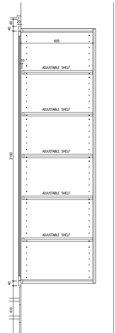
D CABINET SECTION Scale 1:10
