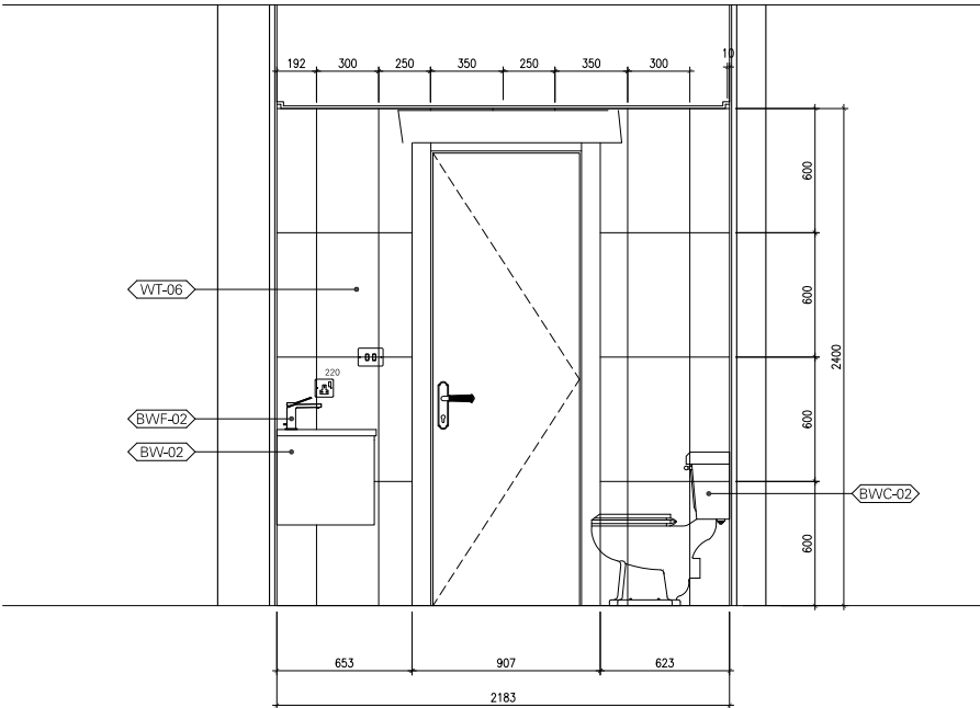
ELEVATION - 4 SCALE 1:20
