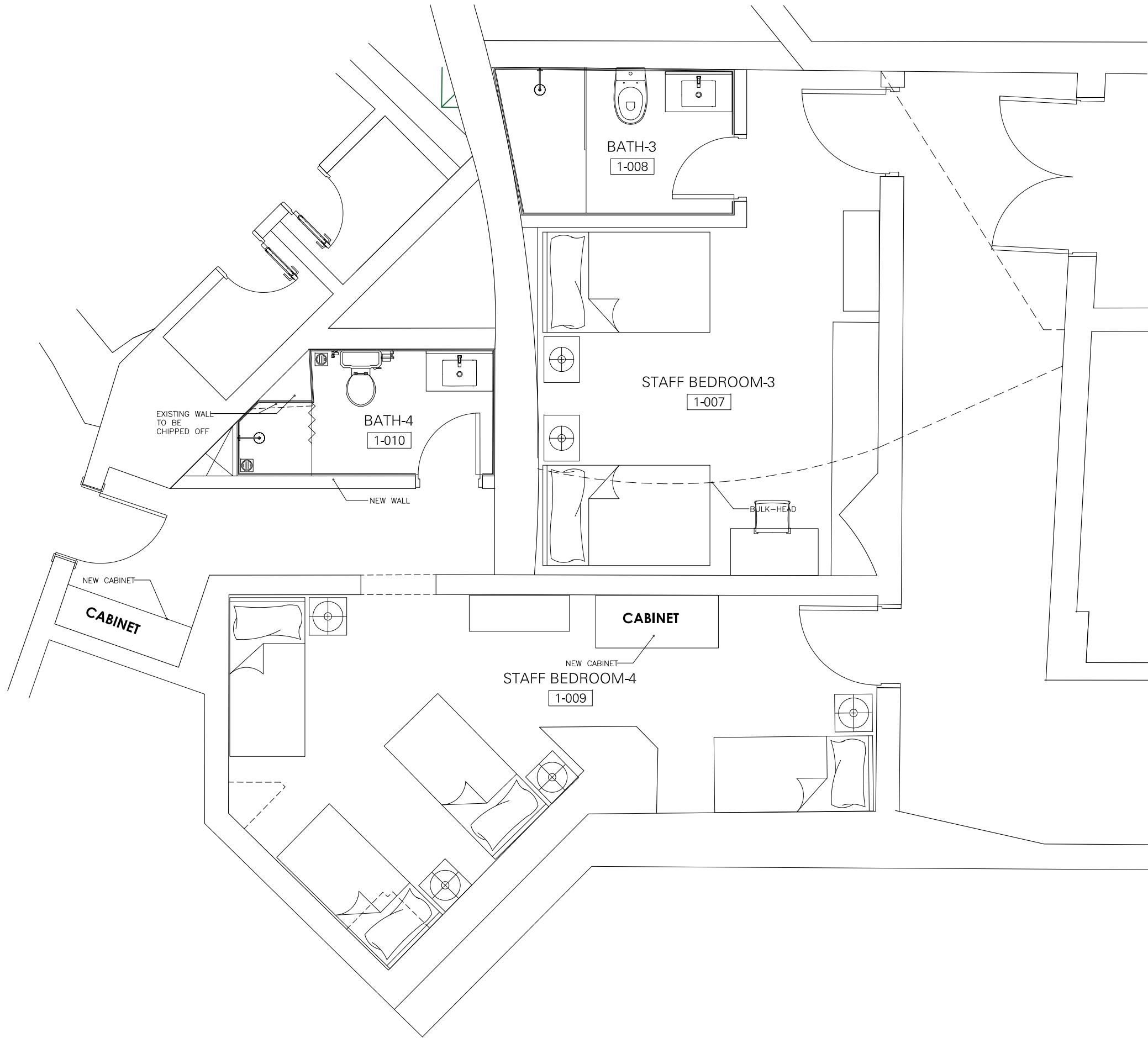
STAFF BEDROOM - 3 & 4 FURNITURE LAYOUT
