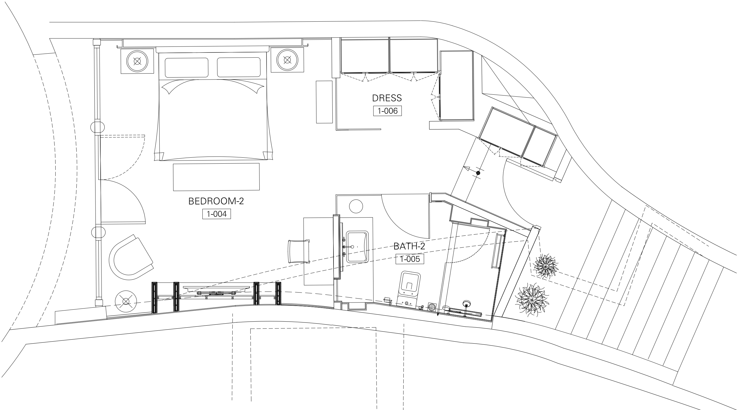
FIRST FLOOR - GUEST BEDROOM - 2 FURNITURE LAYOUT SCALE 1:25
