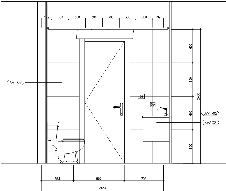
ELEVATION - 1 SCALE 1:20
