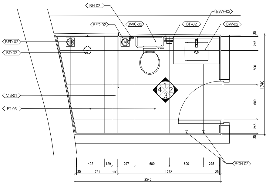
STAFF BATH-3 (1-008) PLAN SCALE 1:20
