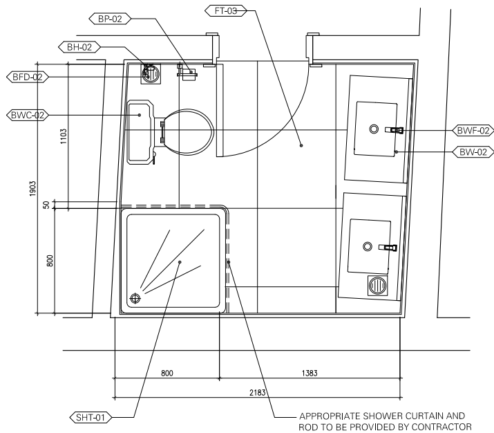
STAFF BATH-6 (1-016) PLAN SCALE 1:20
