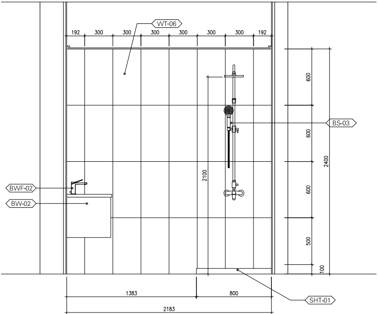
ELEVATION - 3 SCALE 1:20
