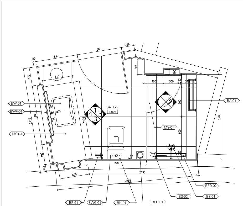
BATHROOM-2 (1-005) PLAN SCALE 1:20
