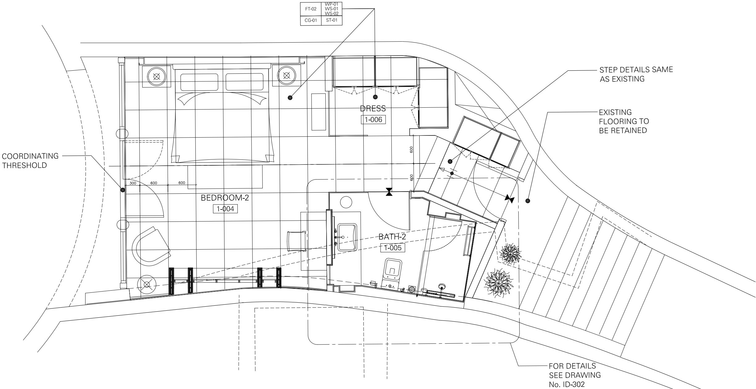
FIRST FLOOR - BEDROOM-2 (1-004) FLOORING LAYOUT SCALE 1:25
