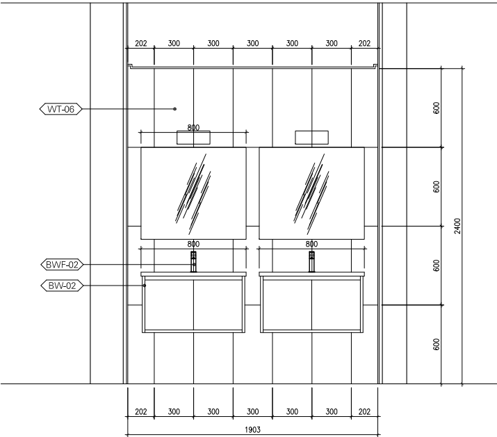
ELEVATION - 4 SCALE 1:20
