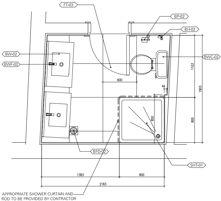
STAFF BATH-5 (1-015) PLAN SCALE 1:20
