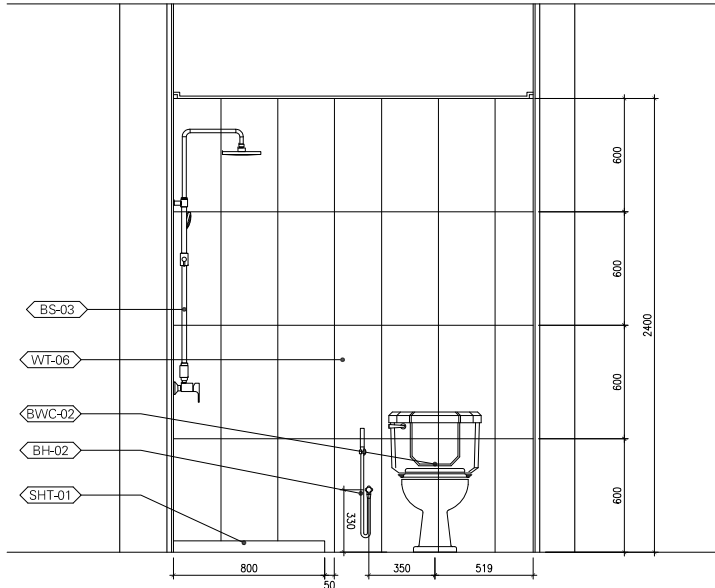
ELEVATION - 4 SCALE 1:20
