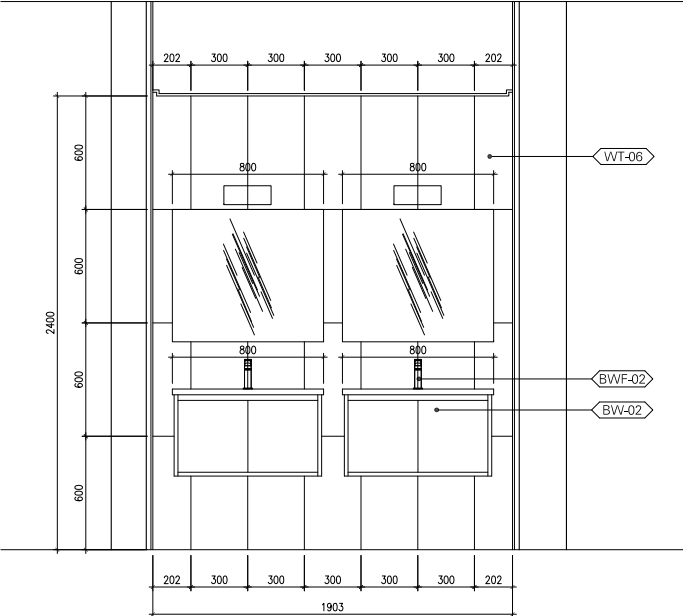
ELEVATION - 2 SCALE 1:20
