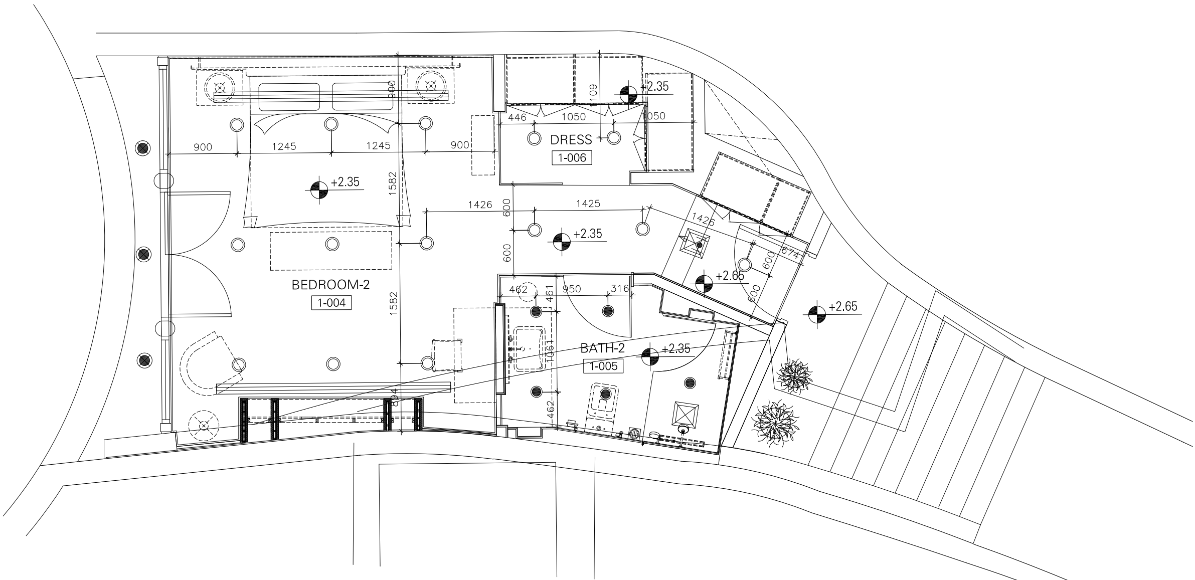
FIRST FLOOR - GUEST BEDROOM - 2 REFLECTED CEILING LAYOUT SCALE 1:25
