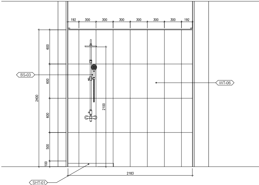
ELEVATION - 2 SCALE 1:20
