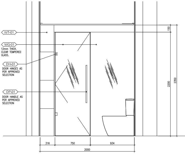
ELEVATION - 5 SCALE 1:20
