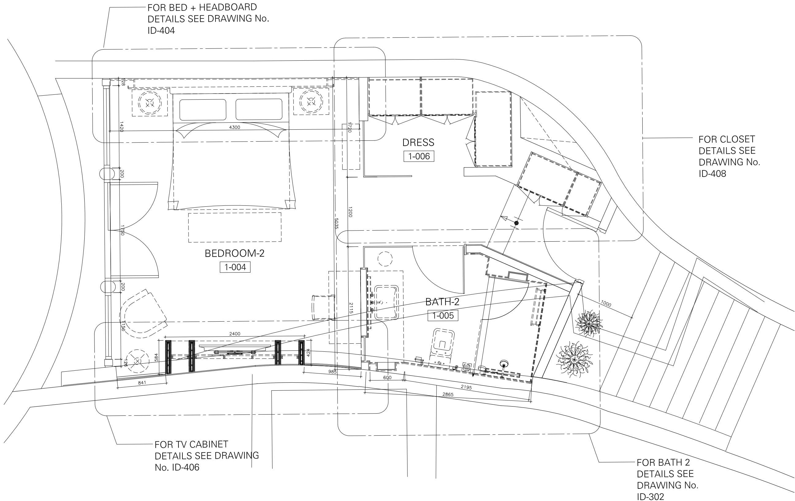
FIRST FLOOR - BEDROOM - 2 (1-004) PLAN SCALE 1:25
