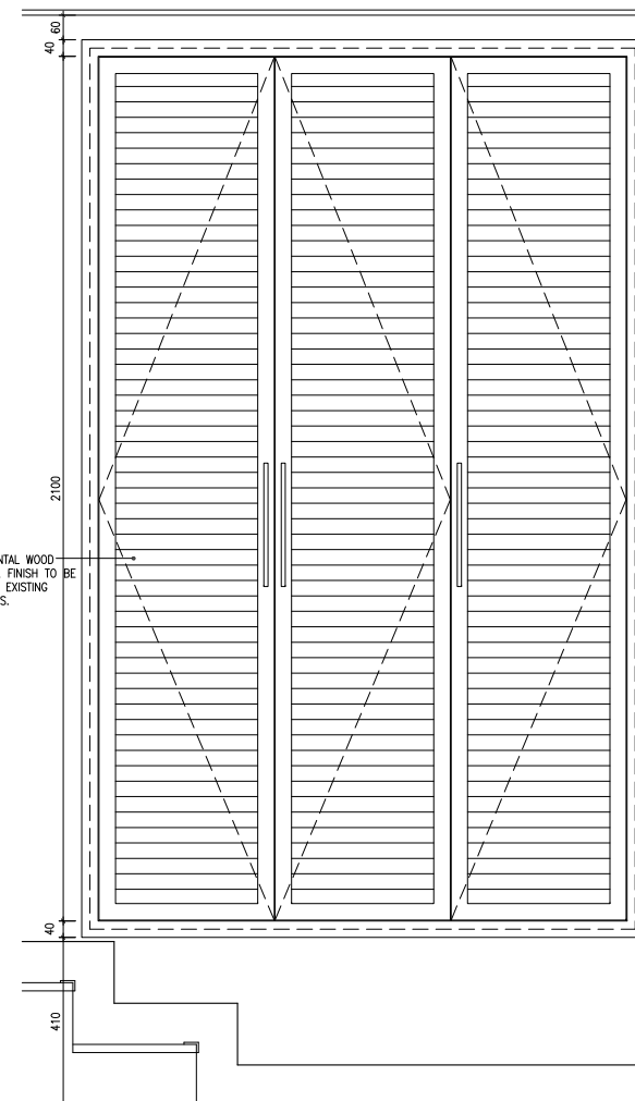
C CABINET ELEVATION - Scale 1:10
