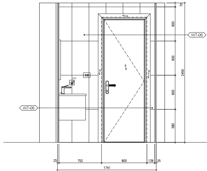
ELEVATION - 2 SCALE 1:20
