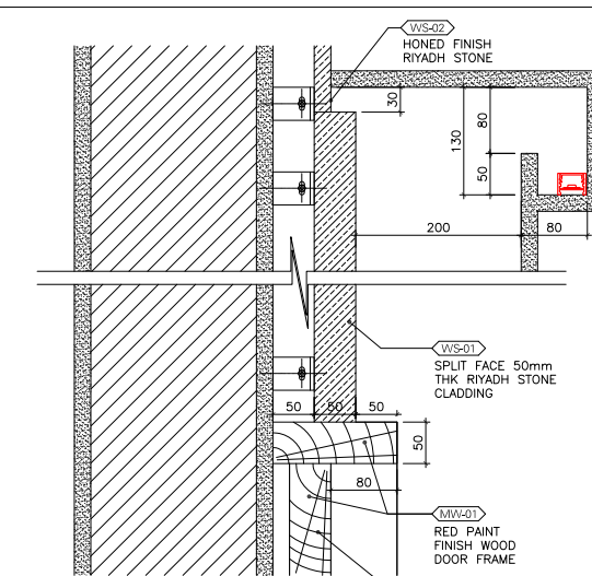
9 DETAIL SCALE 1:5
