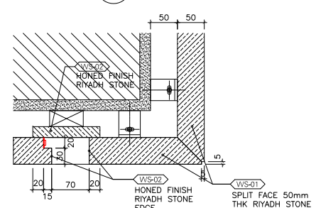
6 DETAIL SCALE 1:5
