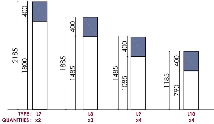
01 FLOOR STANDING - LARGE ELEMENTS WITH DISPLAY CASE - ELEVATIONS Scale 1:20
