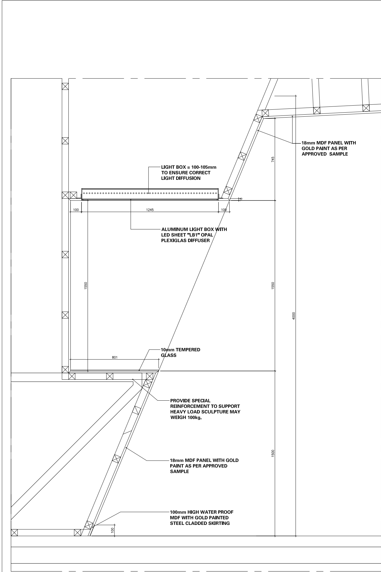
2 SECTION - A SCALE 1:10
