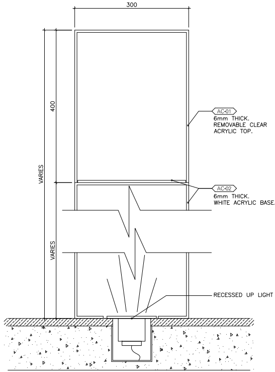
01 TYPICAL FLOOR STANDING PEDESTAL WITH DISPLAY CASE Scale 1:5
