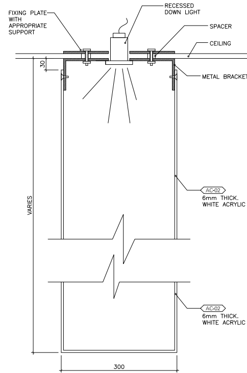
04 TYPICAL LARGE CEILING MOUNTED ELEMENTS Scale 1:5
