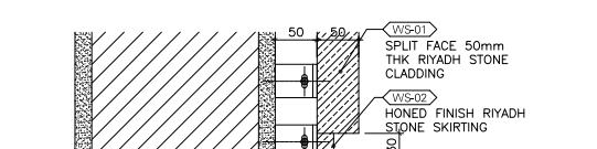
8 DETAIL SCALE 1:5
