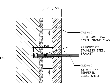
5 DETAIL SCALE 1:5
