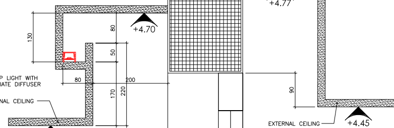
3 CLG DETAIL @ FACADE SCALE 1:5
