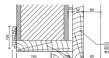
3 DETAIL SCALE 1:5
