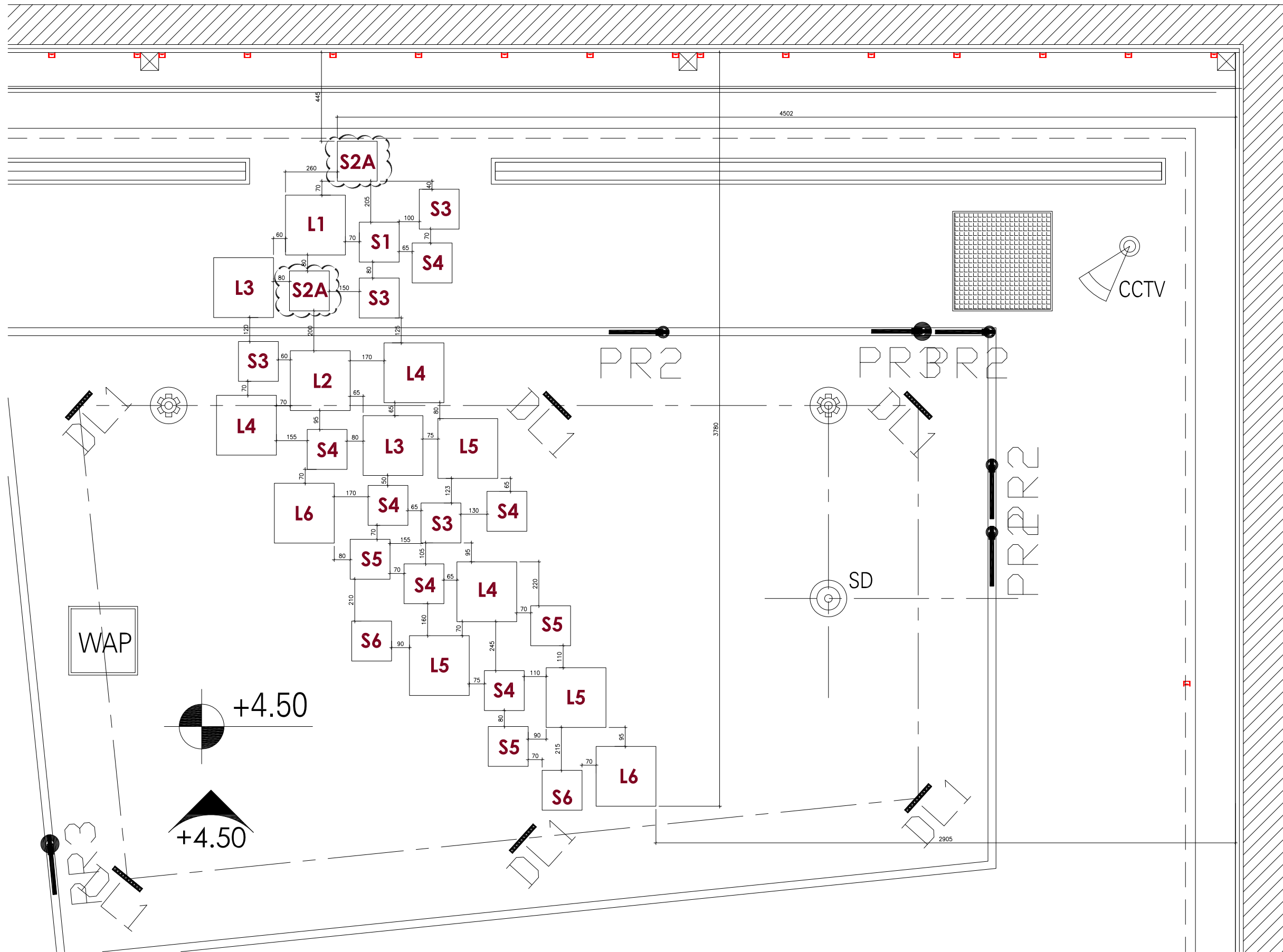
02 CEILING MOUNTED - LIGHTING ELEMENTS KEY PLAN Scale 1:10
