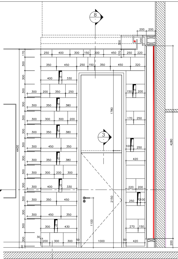
3 ELEVATION - C SCALE 1:20
