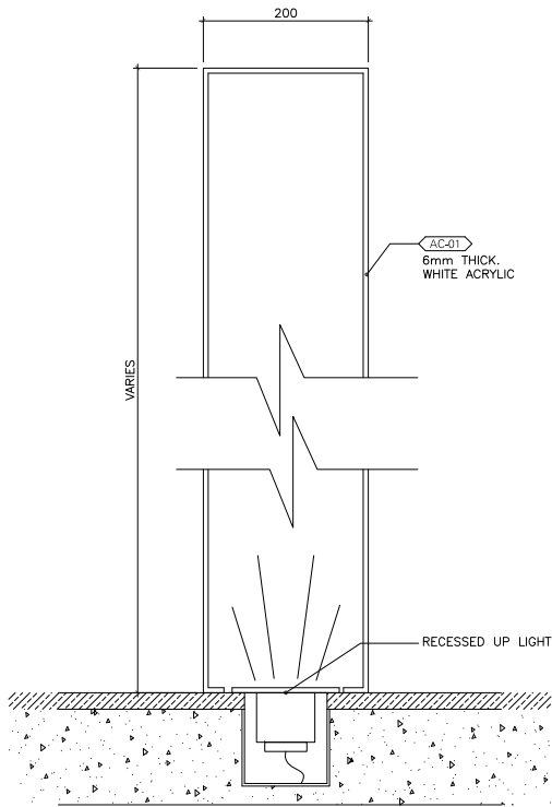
03 TYPICAL FLOOR STANDING PEDESTAL WITHOUT DISPLAY CASE Scale 1:5
