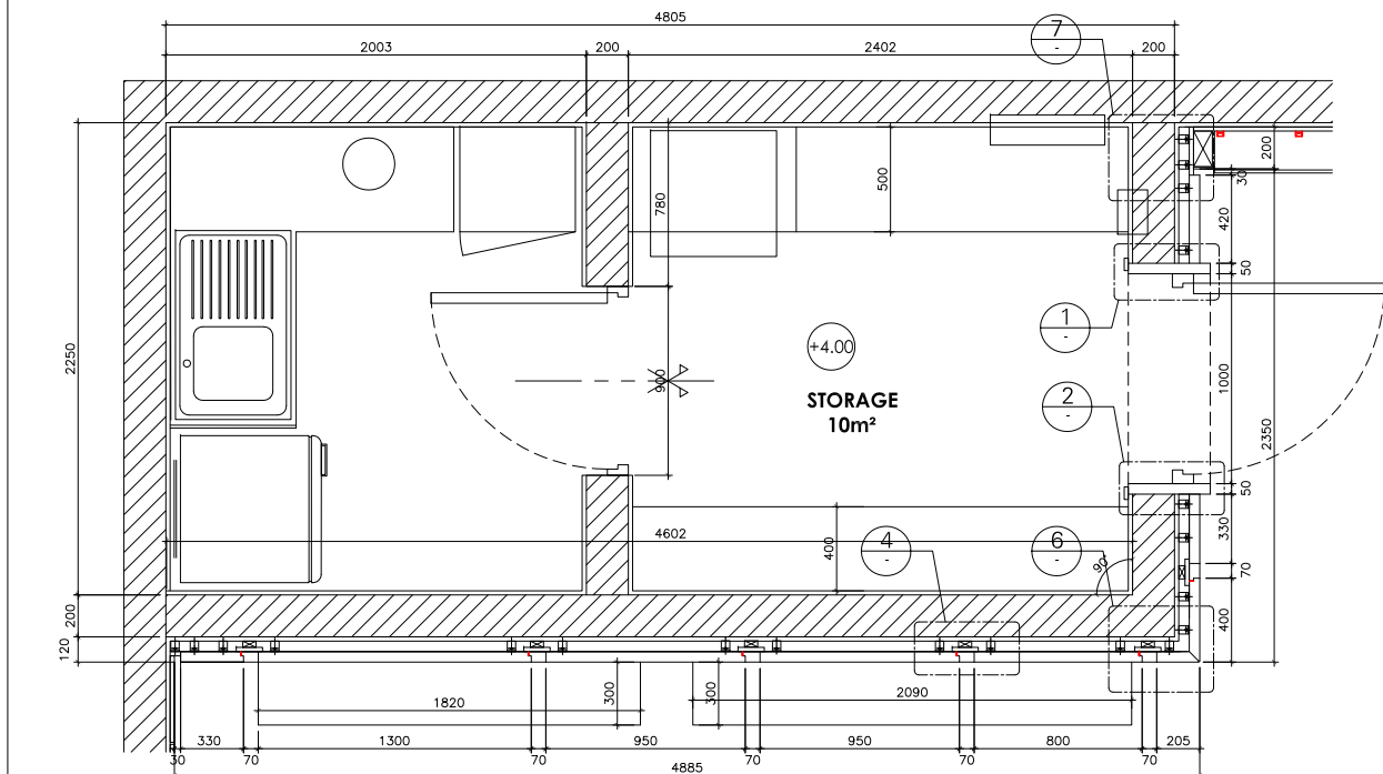
A PLAN SCALE 1:20
