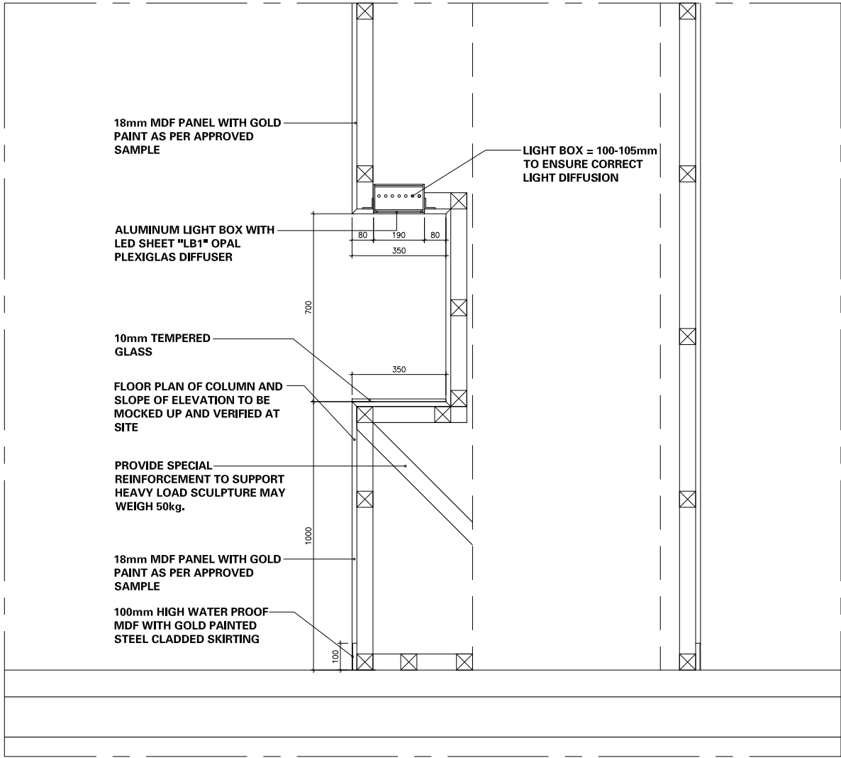
3 SECTION - B SCALE 1:10
