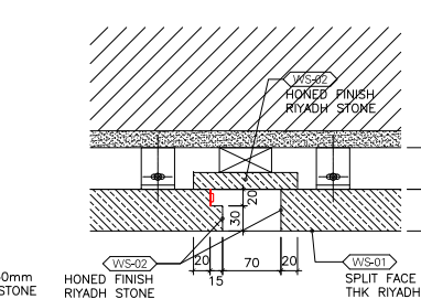
4 DETAIL SCALE 1:5
