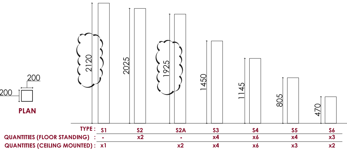
02 FLOOR STANDING + CEILING MOUNTED - SMALL ELEMENT ELEVATIONS Scale 1:20
