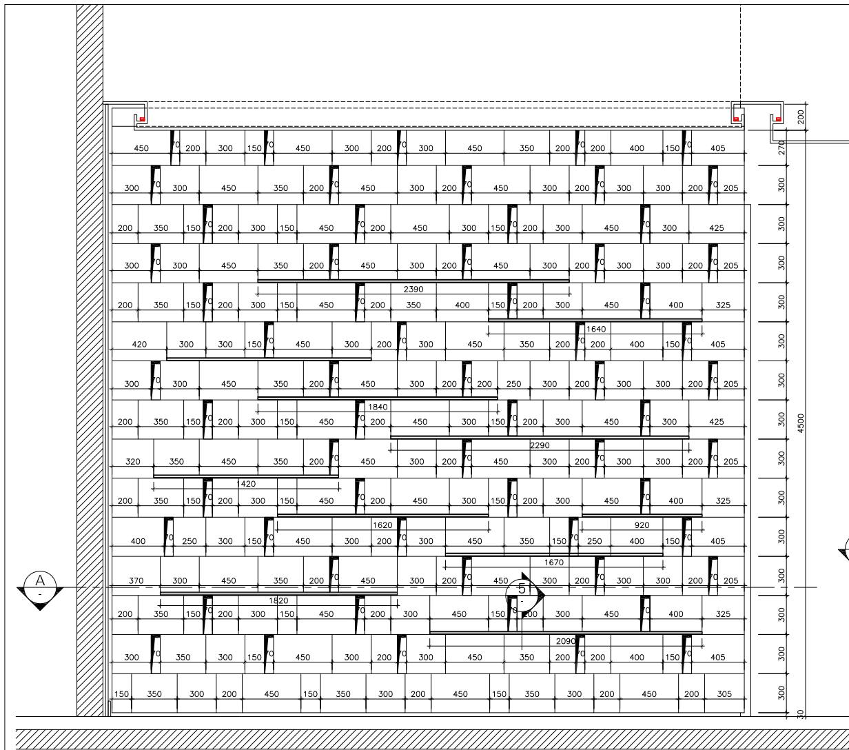
2 ELEVATION - B SCALE 1:20
