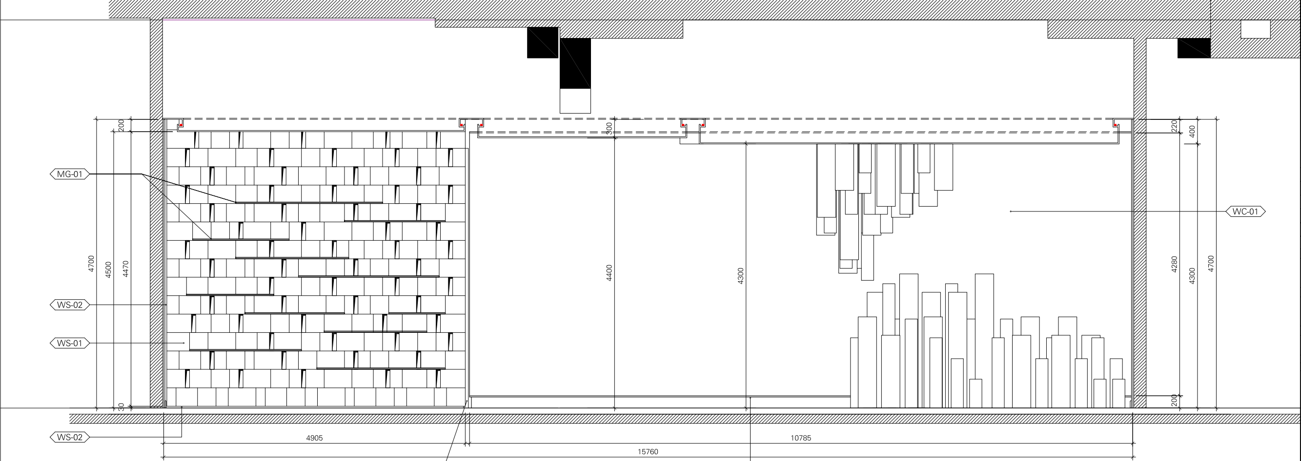
2 ELEVATION - B SCALE 1:30
