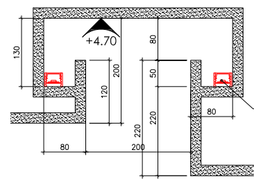
2 TYPICAL CLG DETAIL SCALE 1:5
