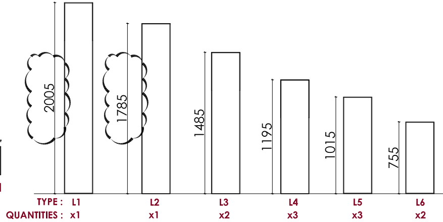
01 CEILING MOUNTED - LARGE ELEMENTS WITHOUT DISPLAY CASE - ELEVATIONS Scale 1:20
