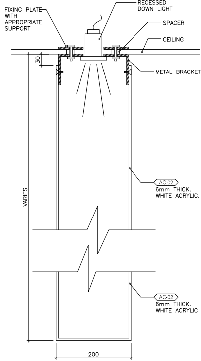
02 TYPICAL SMALL CEILING MOUNTED ELEMENTS Scale 1:5
