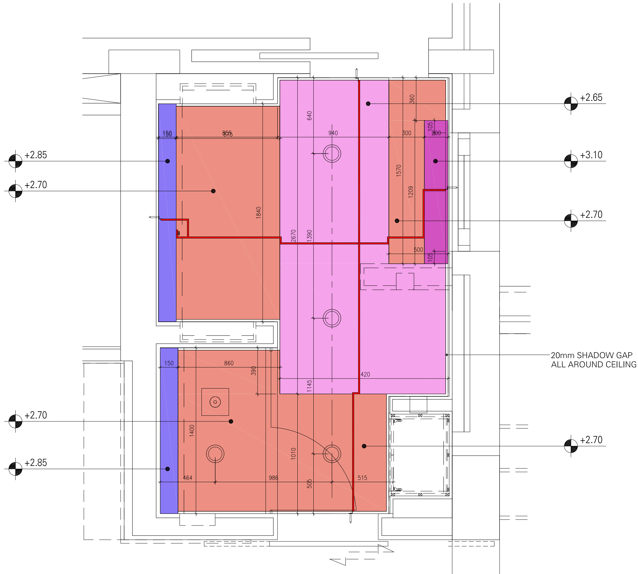
BATH (01-06) CEILING LAYOUT SCALE 1:10
