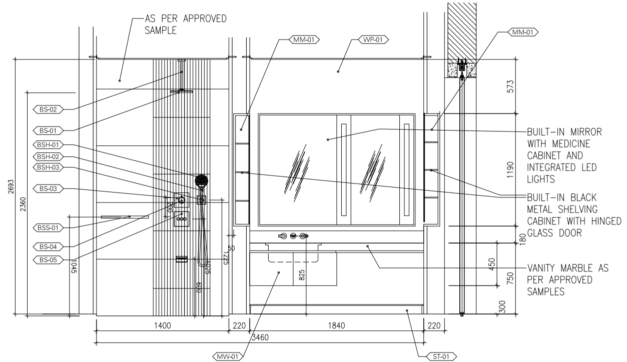
ELEVATION - 01 SCALE 1:25
