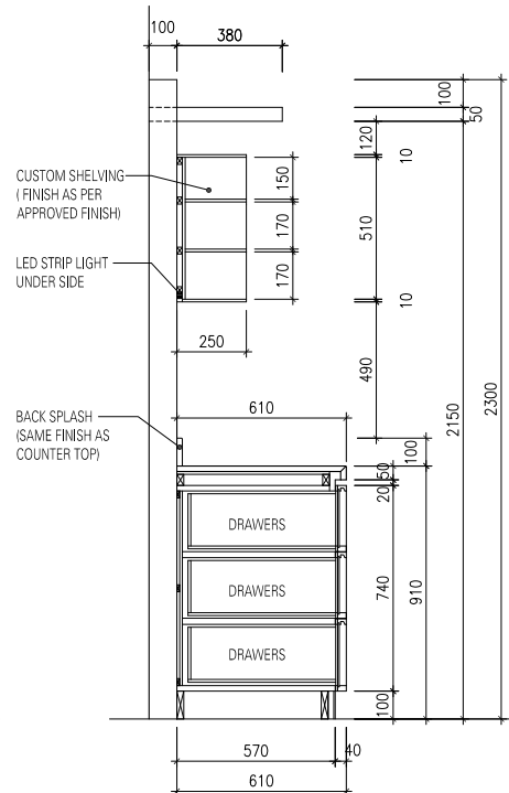
SECTION-2
