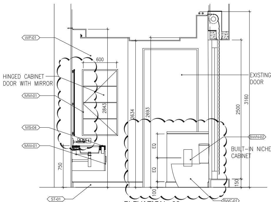
ELEVATION - 02 SCALE 1:25
