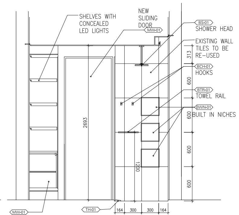
ELEVATION - 04 SCALE 1:25
