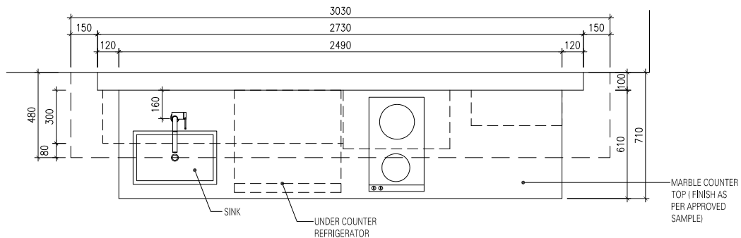
KITCHENETTE PLAN
