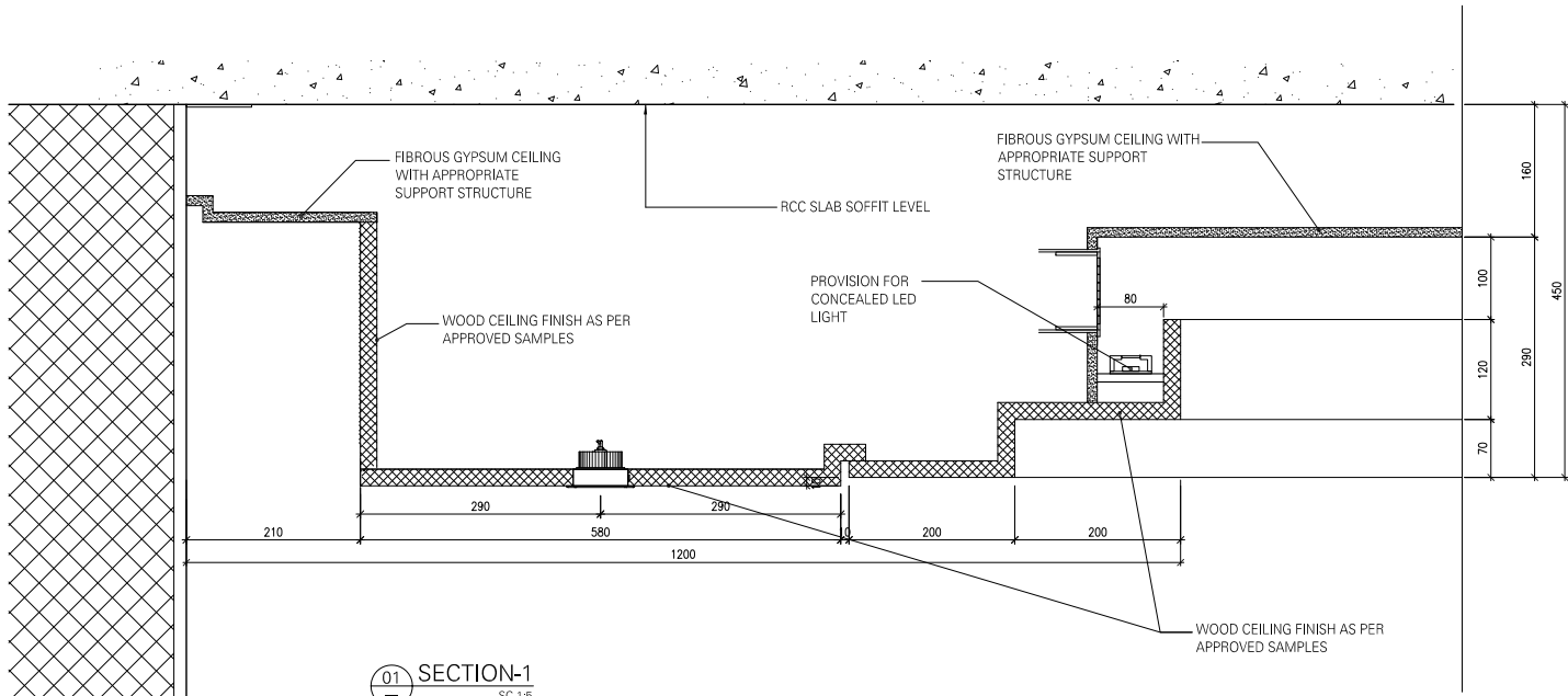
TYPICAL CEILING SECTION AT SALON (01-05B)
