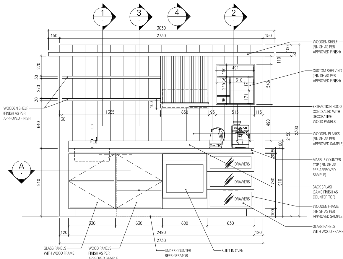
KITCHENETTE ELEVATION
