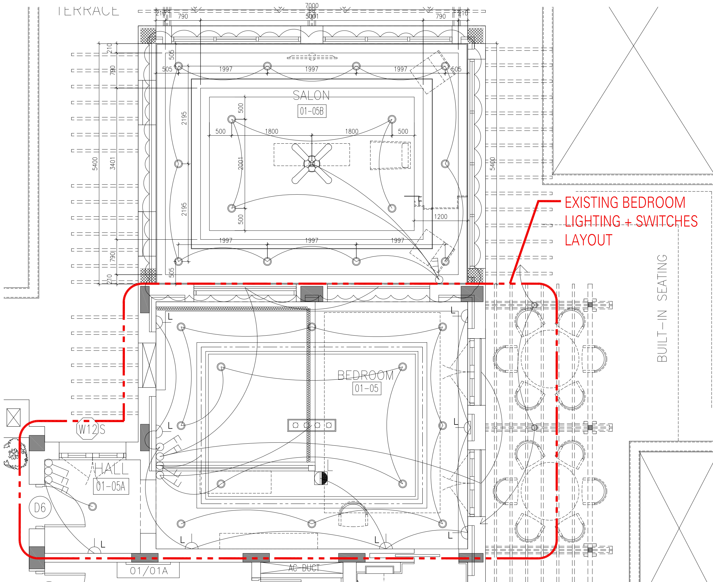
BEDROOM + SALON LIGHTING LAYOUT
