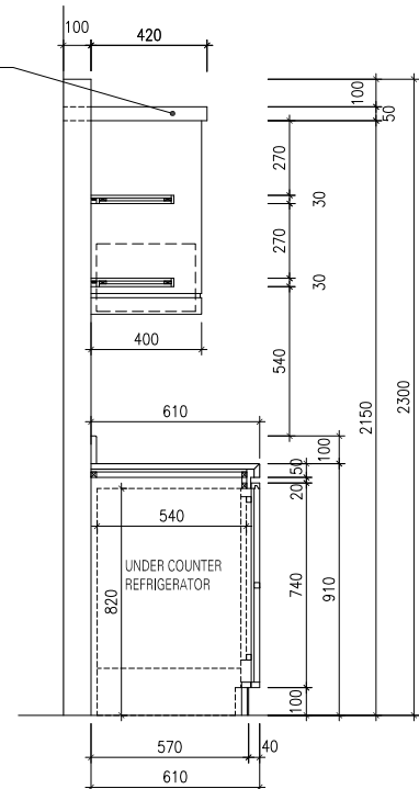
SECTION-1
