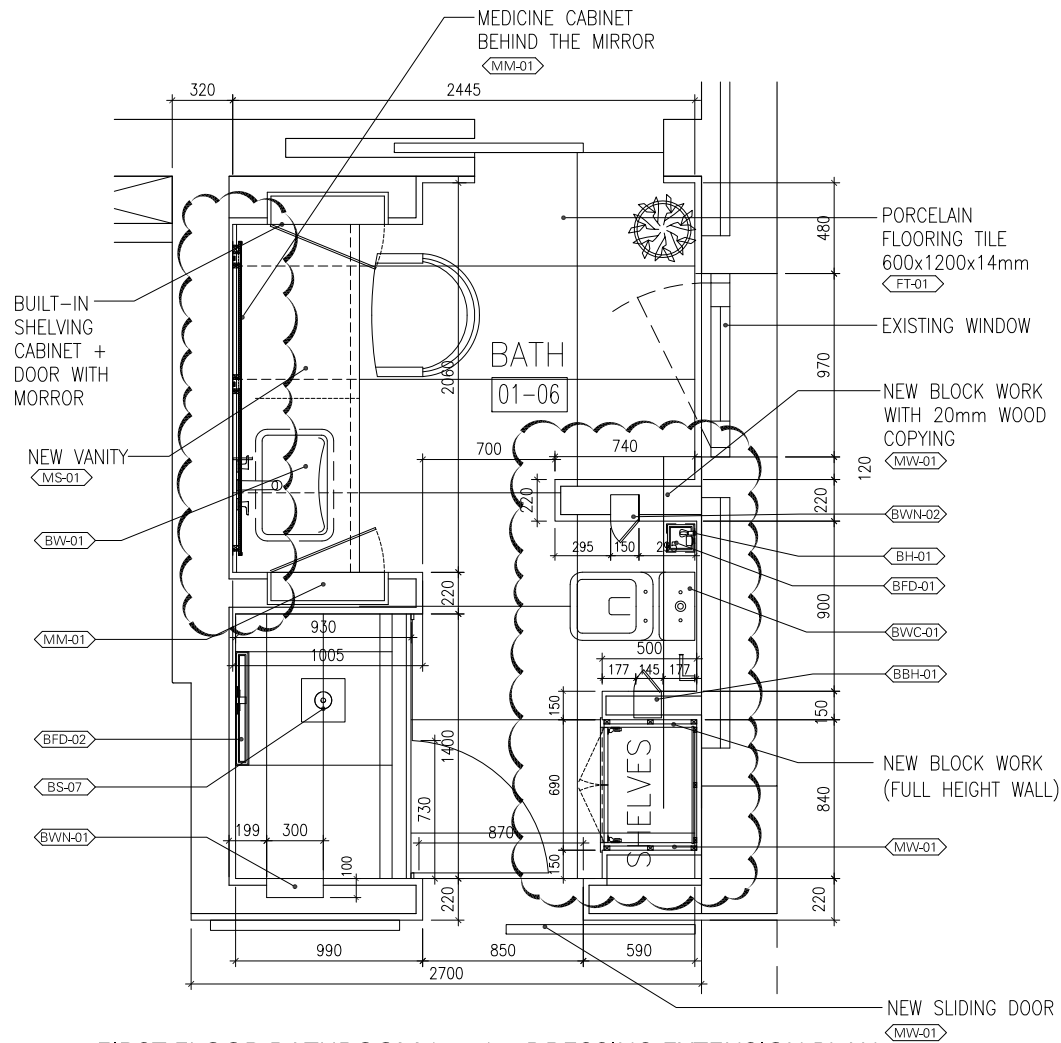
FIRST FLOOR BATHROOM (1-06) + DRESSING EXTENSION PLAN SCALE 1:25
