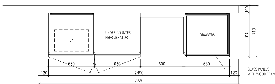
PLAN SECTION - A
