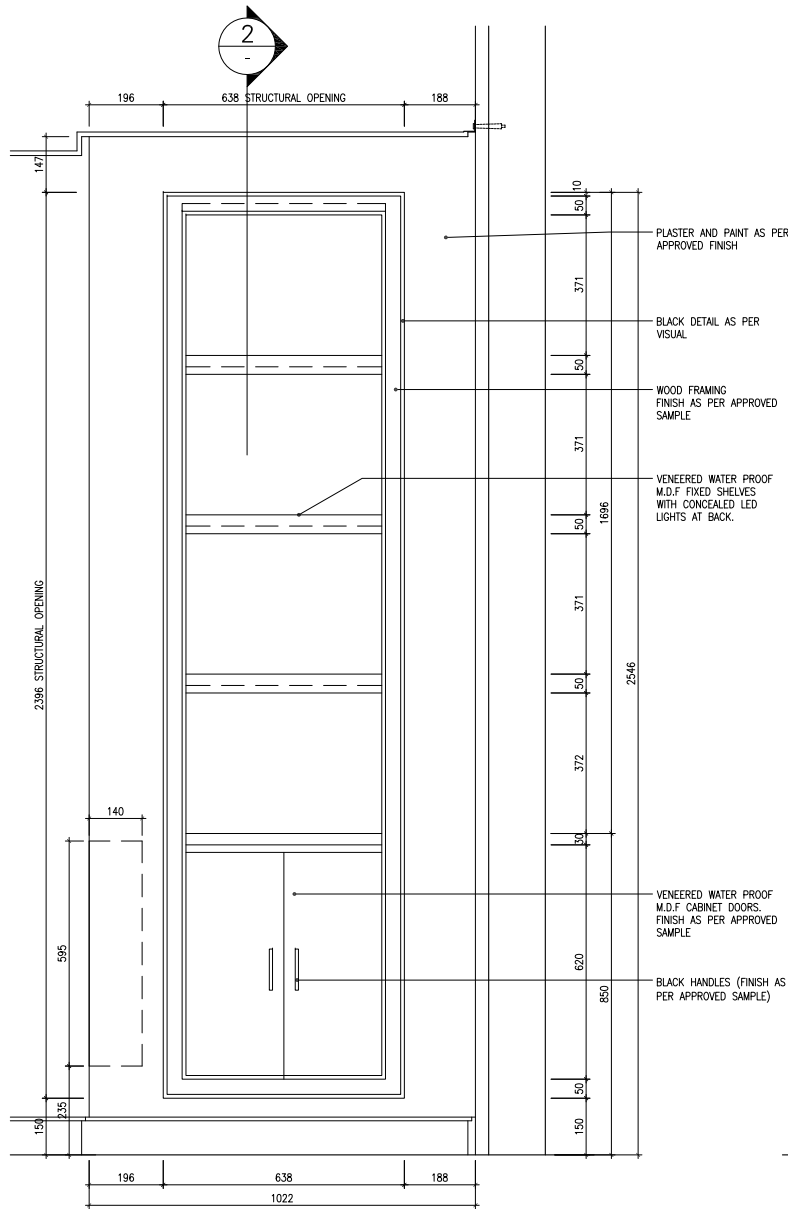
SHELVING + STORAGE UNIT ELEVATION SCALE 1:10
