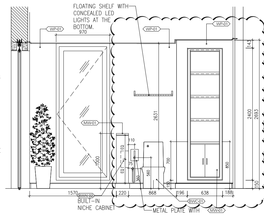
ELEVATION - 03 SCALE 1:25
