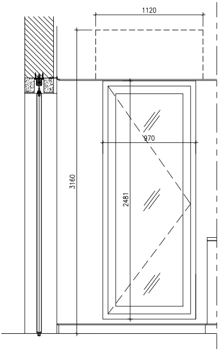
BATHROOM WINDOW ELEVATION
