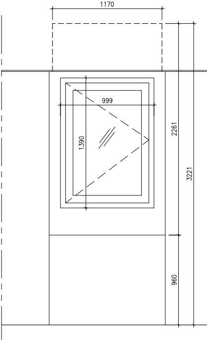
DRESSING WINDOW ELEVATION
