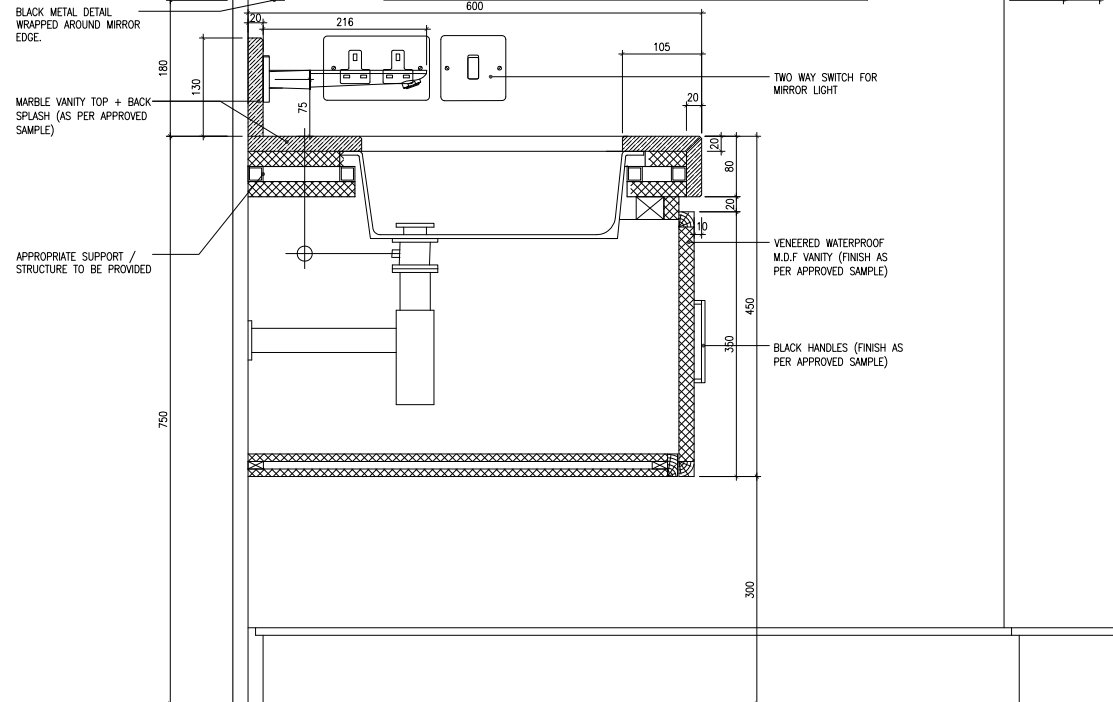
02 VANITY SECTION
