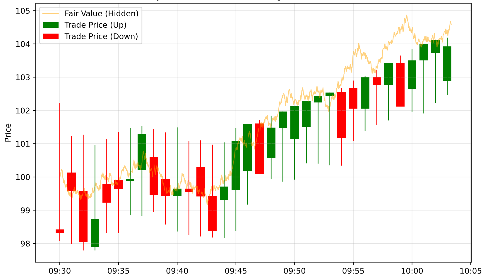
Day 7: Noise Traders Tracking Brownian Motion
