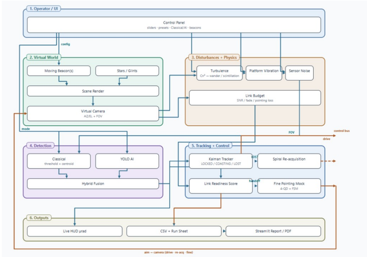
Figure 1: BeamLock real-time PAT architecture. Forward path: scene → disturbances/physics → detection → tracking/control → outputs. Feedback path: Kalman / re-acquisition / fine mock drives the virtual camera AZ/EL plant. ( Note: the live default re-acquisition pattern is raster ; spiral generation remains in code for literature comparison.)
