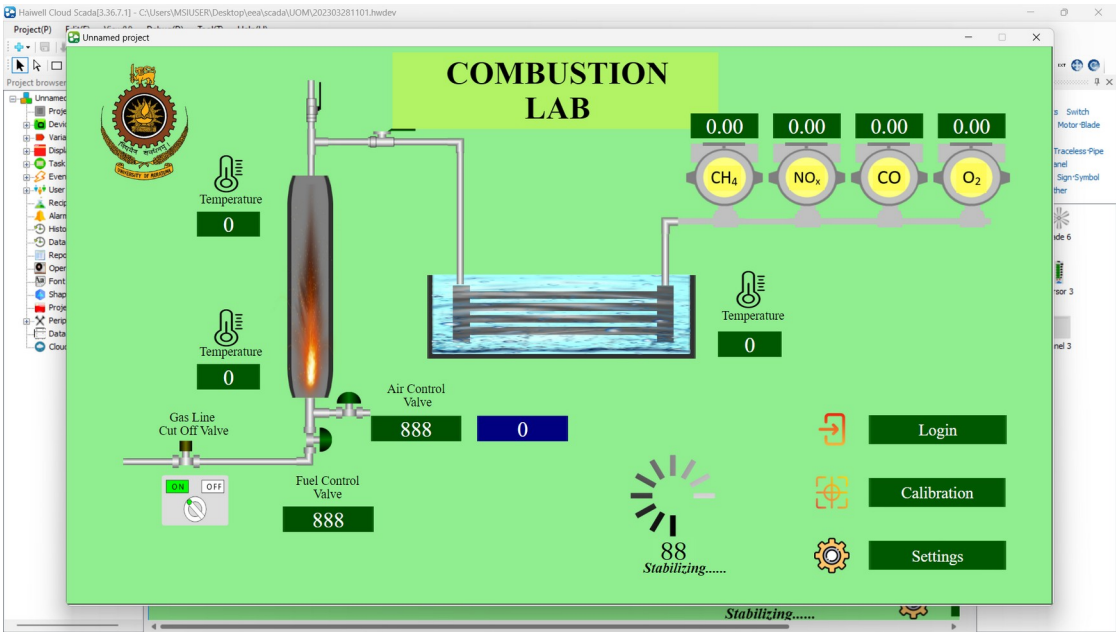
Haiwell SCADA user interface — customised GUI
