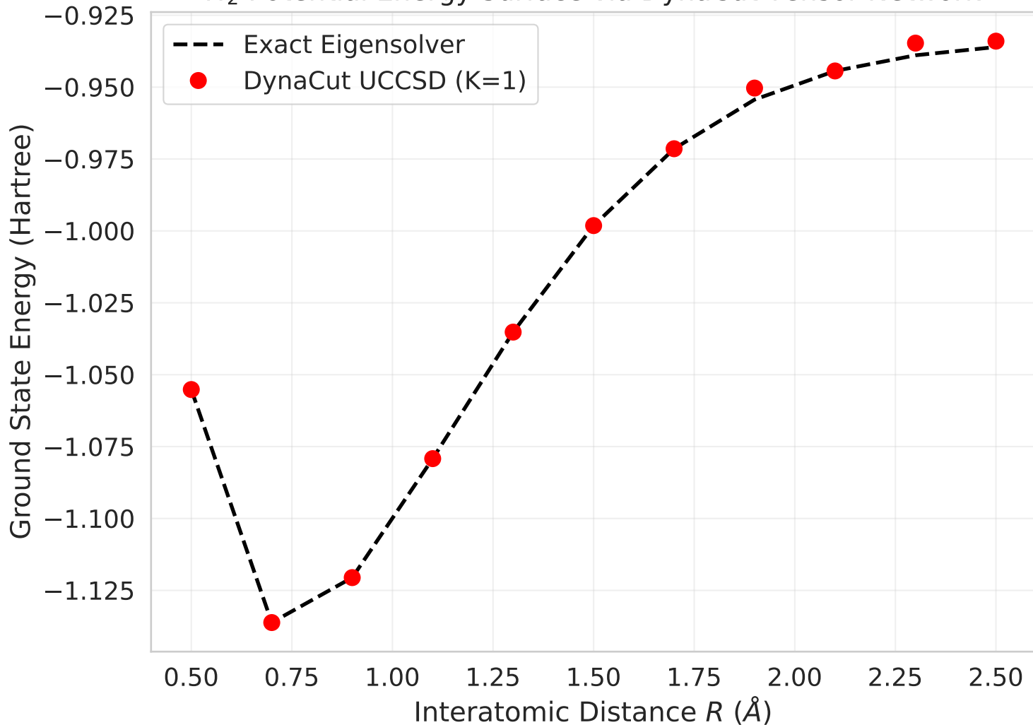
H_2 Potential Energy Surface via DynaCut Tensor Network
