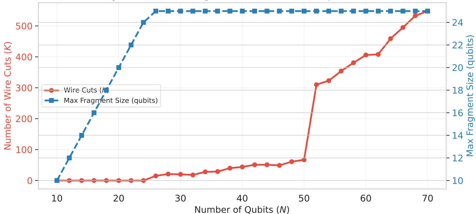
DynaCut Partitioning Profile on Dense SBM ( p_{out} = 0.10 )
