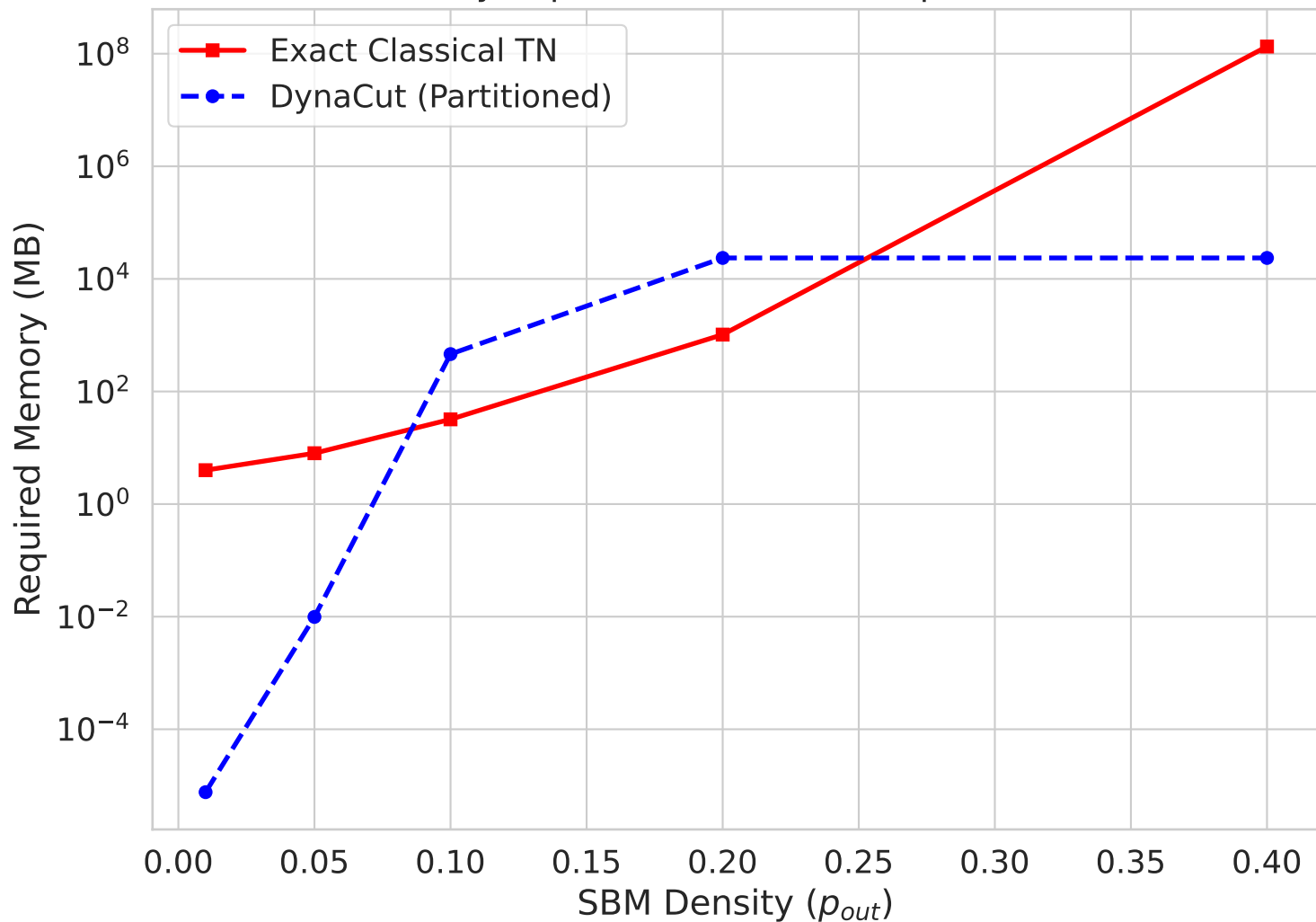
Memory Explosion on Dense Graphs (N=20)
