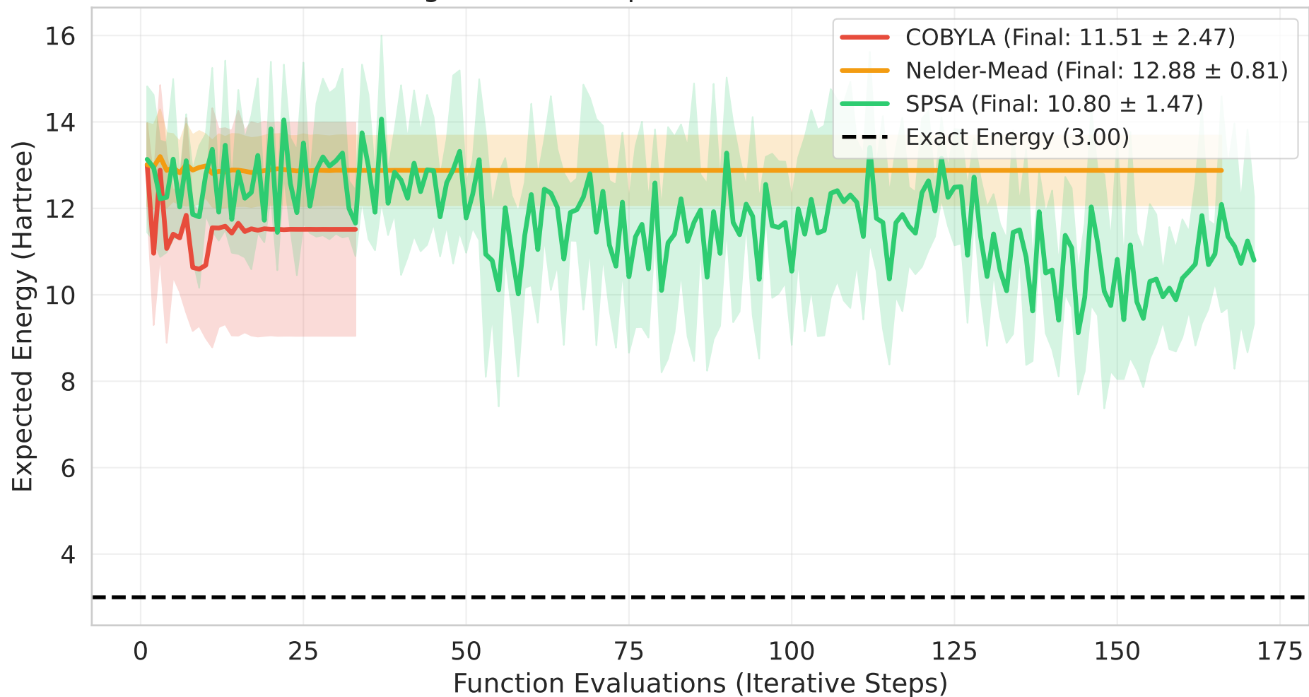
VQE Optimizer Comparison Under HPC-Scale QPD Sampling Noise (N=16) Average over 5 independent random initializations
