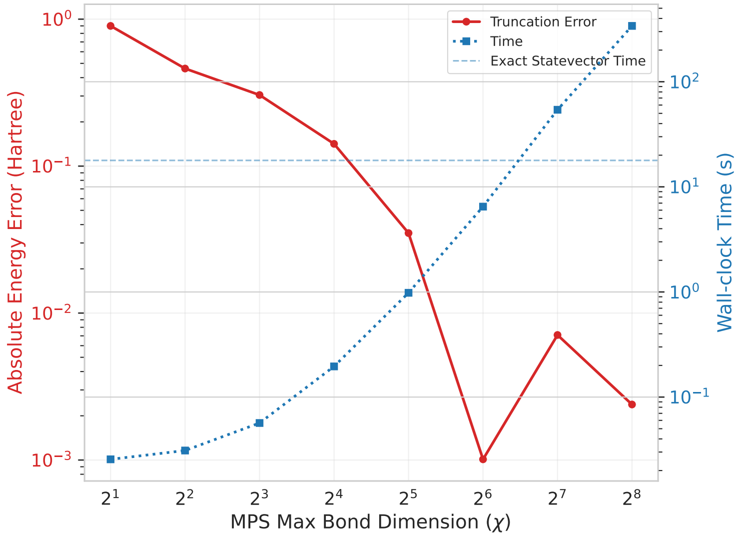
Tensor Network Pareto Frontier: Precision vs. Time (N=26 Dense SBM)
