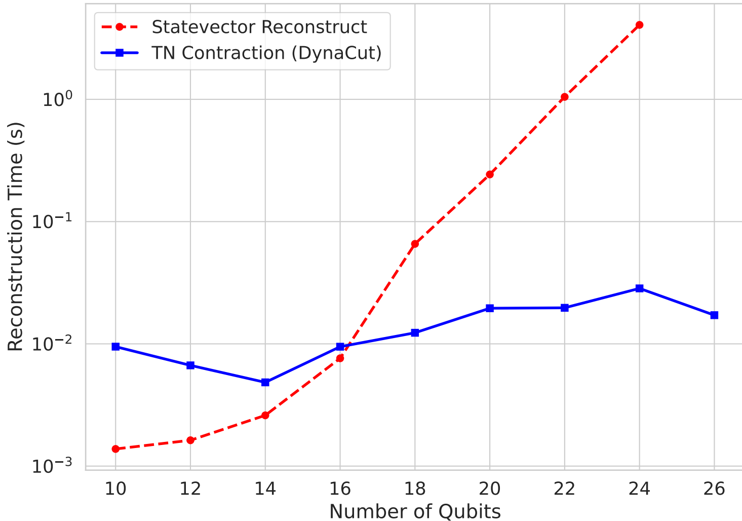
Tensor Network vs Standard Reconstruction
