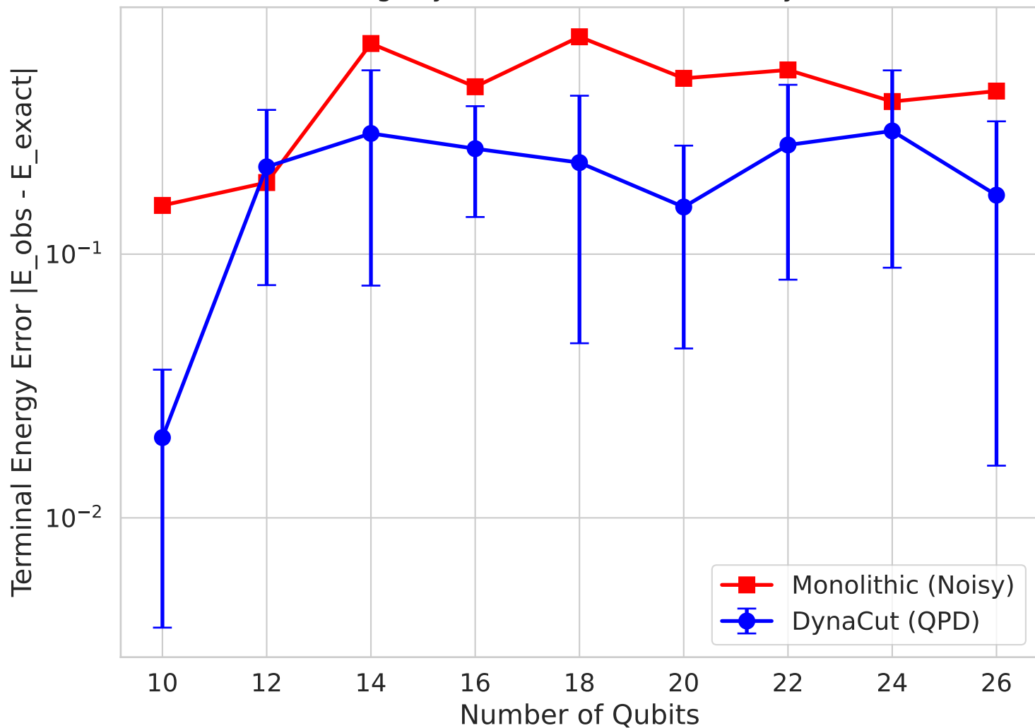
Error Scaling: DynaCut vs Monolithic Noisy Execution
