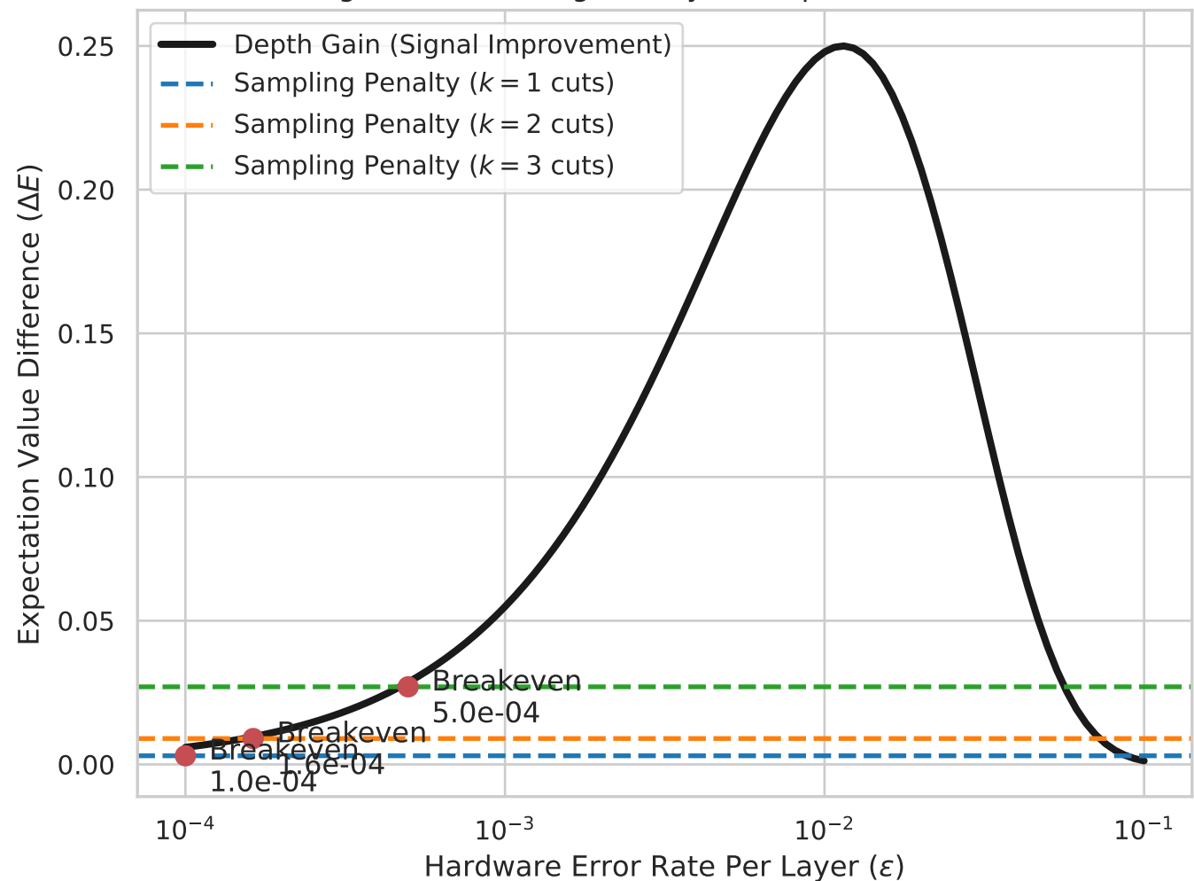
Entanglement Severing Penalty vs. Depth Reduction Gain
