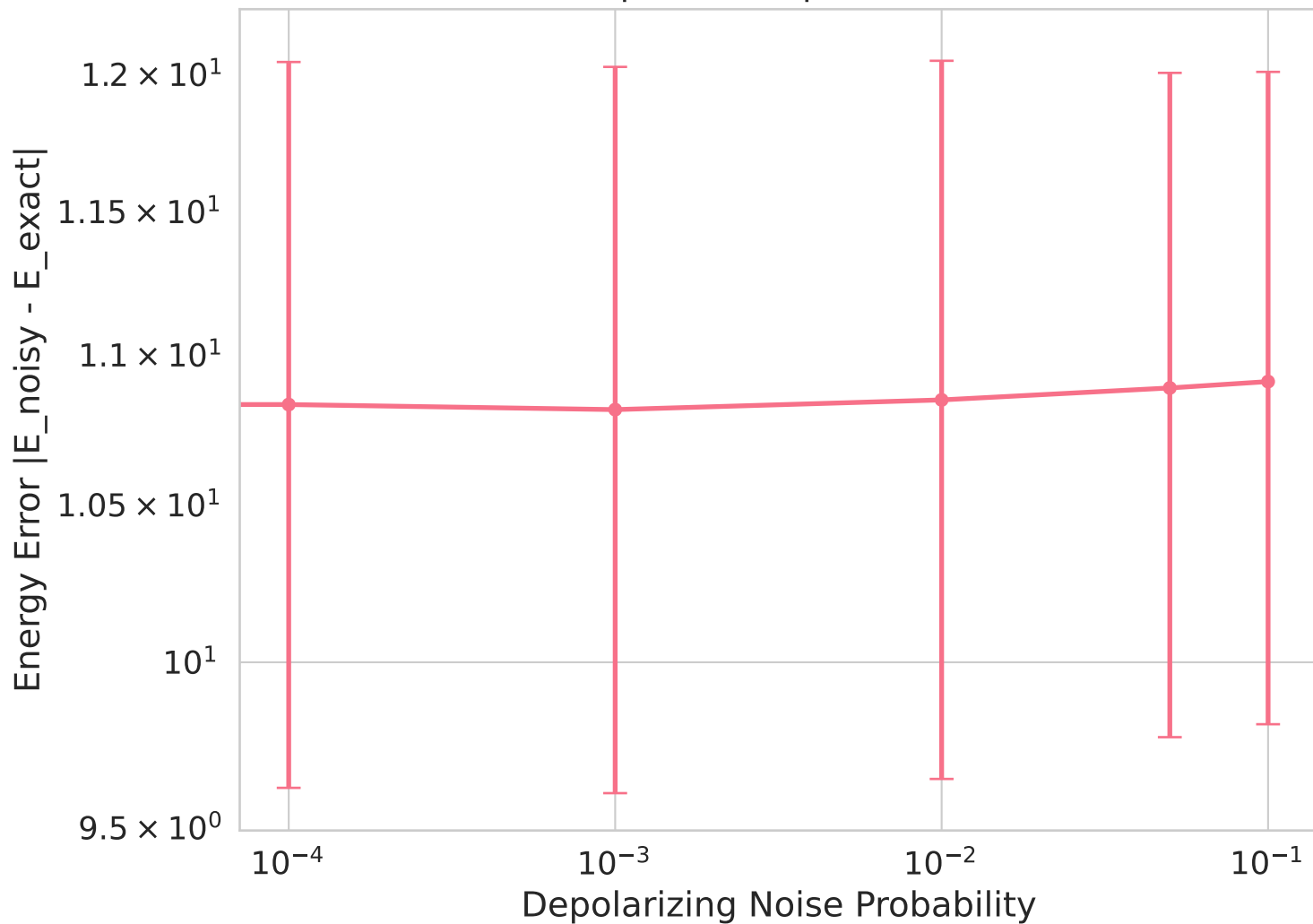
Noise Impact on Expectation Values
