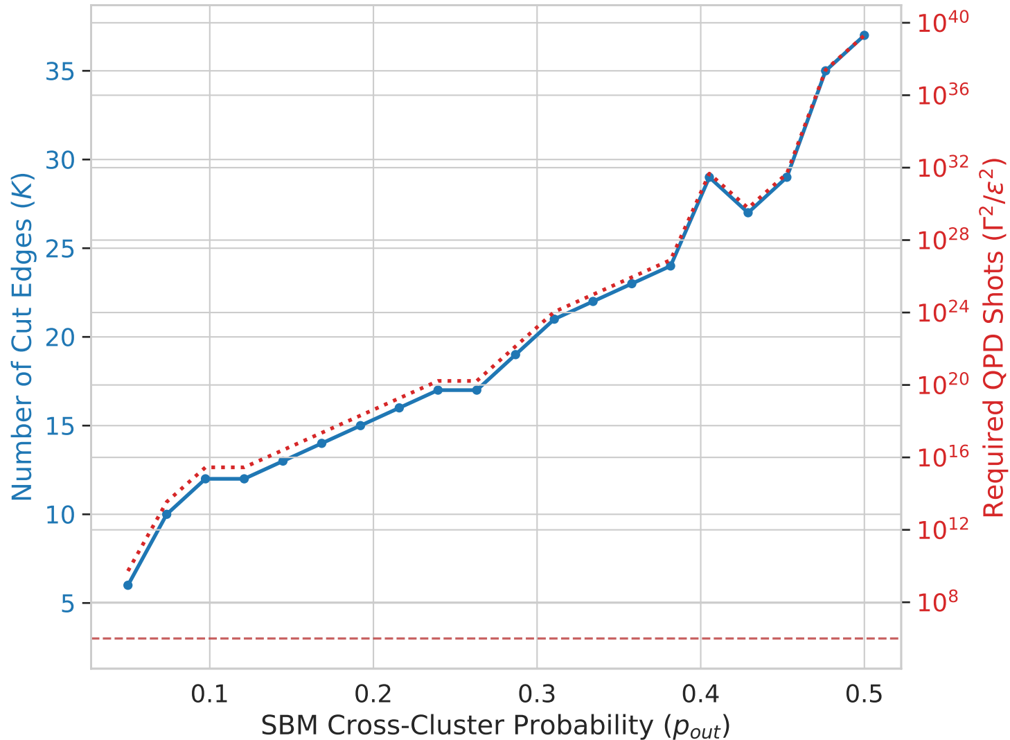
Topology Stress Test: QPD Overhead vs Graph Density
