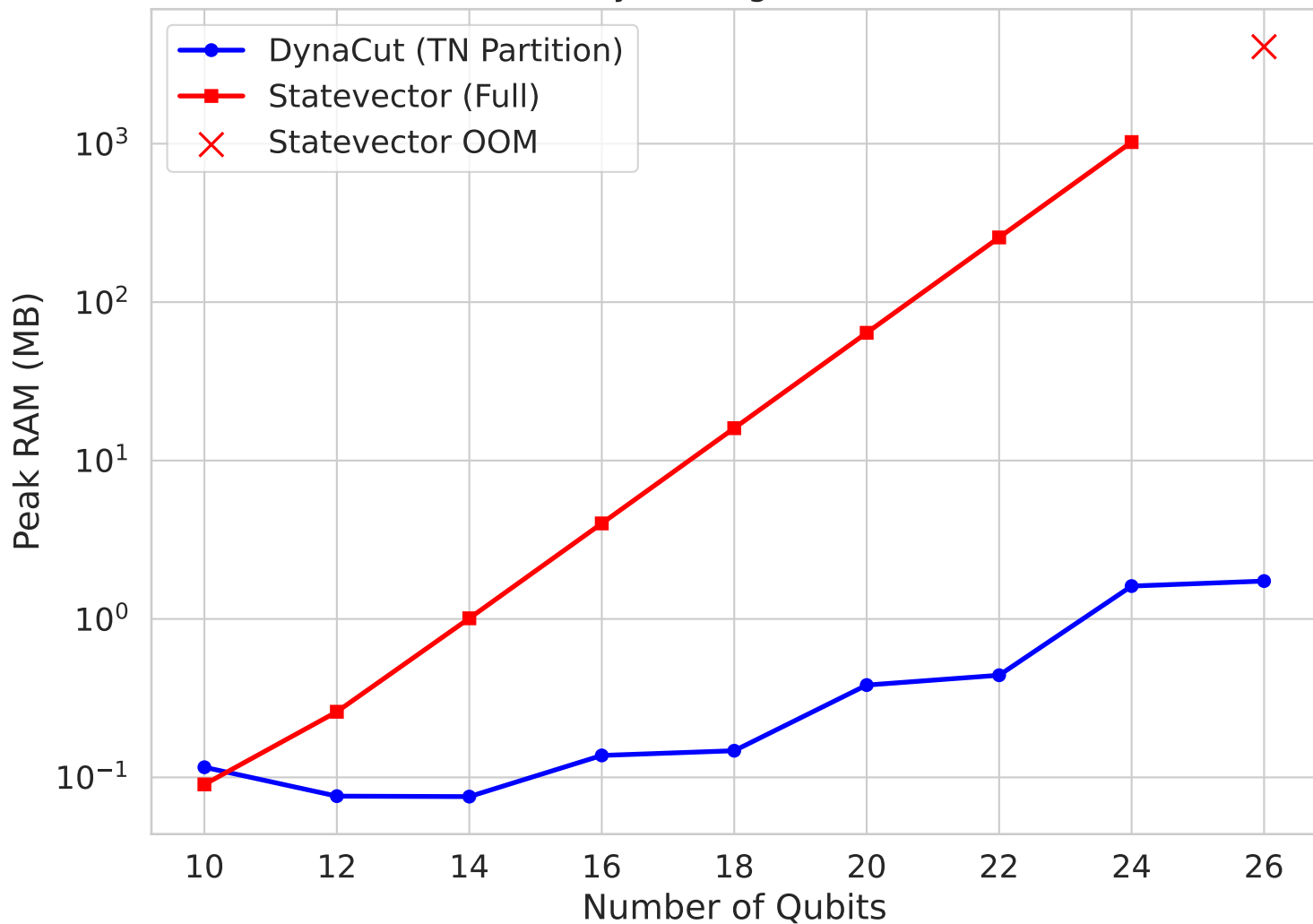
Memory Scaling Benchmark
