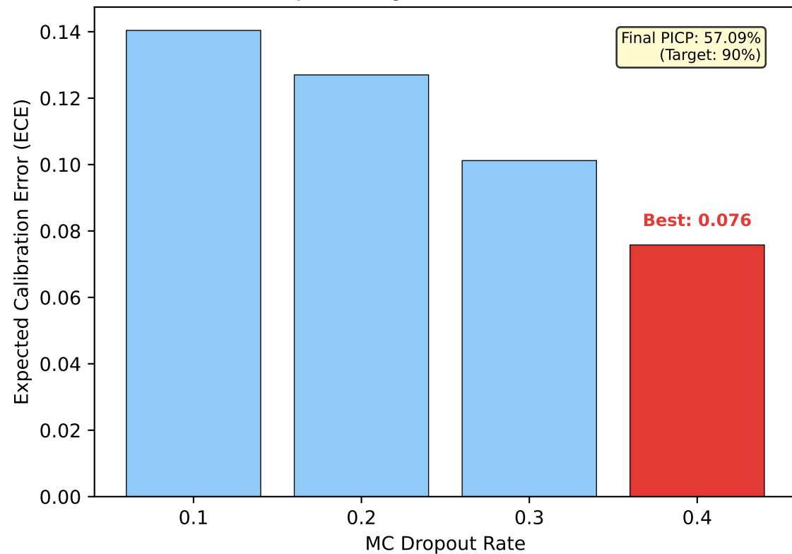
PJM: Dropout Rate vs ECE
