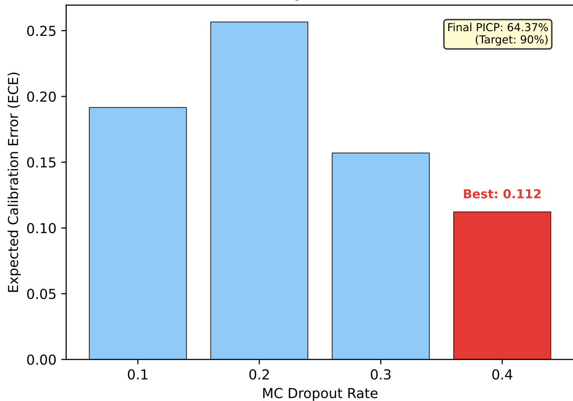
ERCOT: Dropout Rate vs ECE
