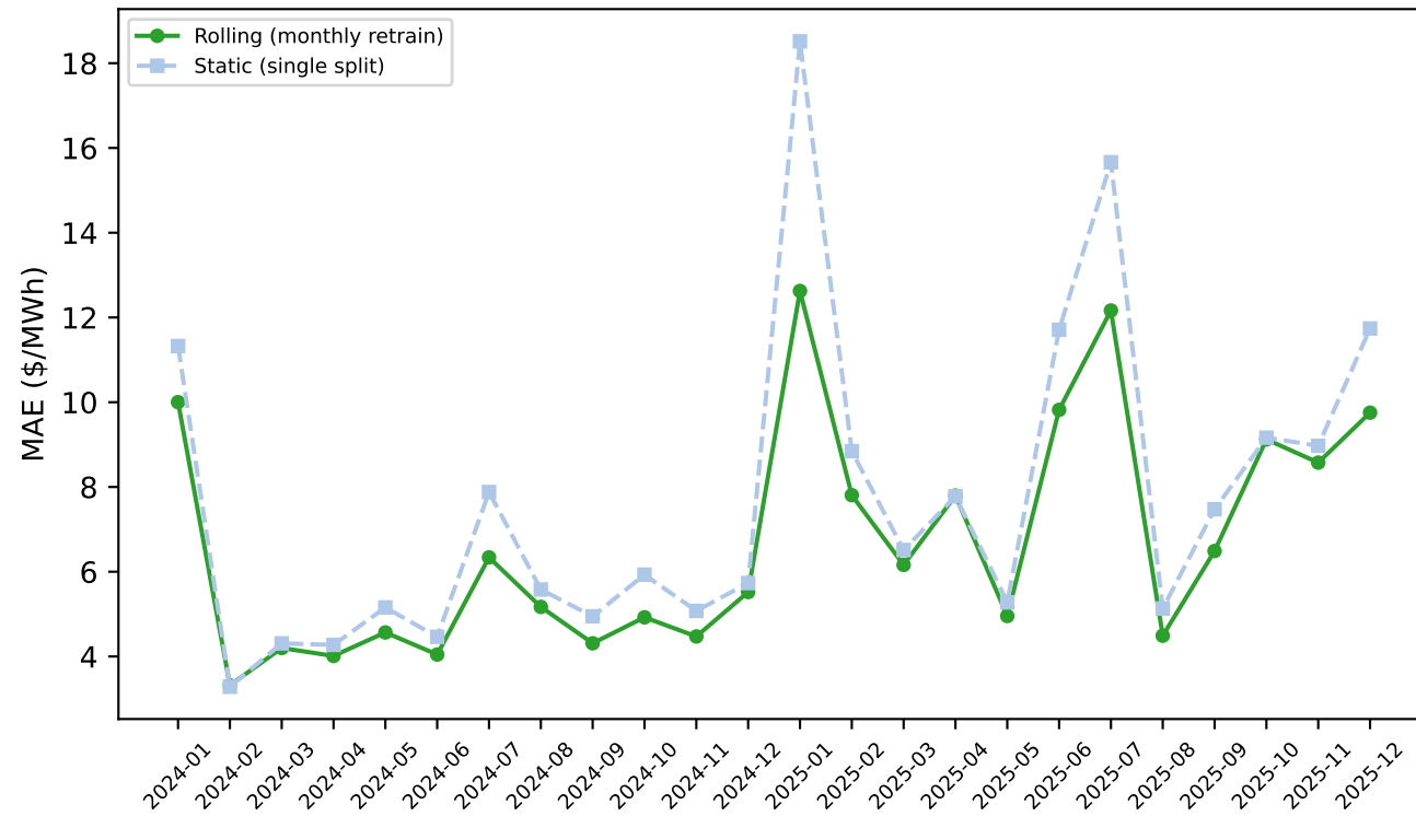
PJM: XGBoost
