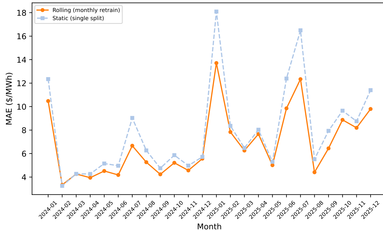
PJM: XGBoost
