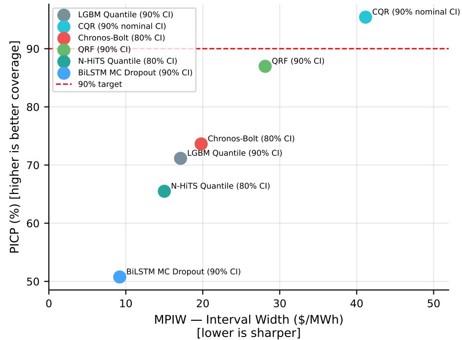
PJM — PICP vs. MPIW
