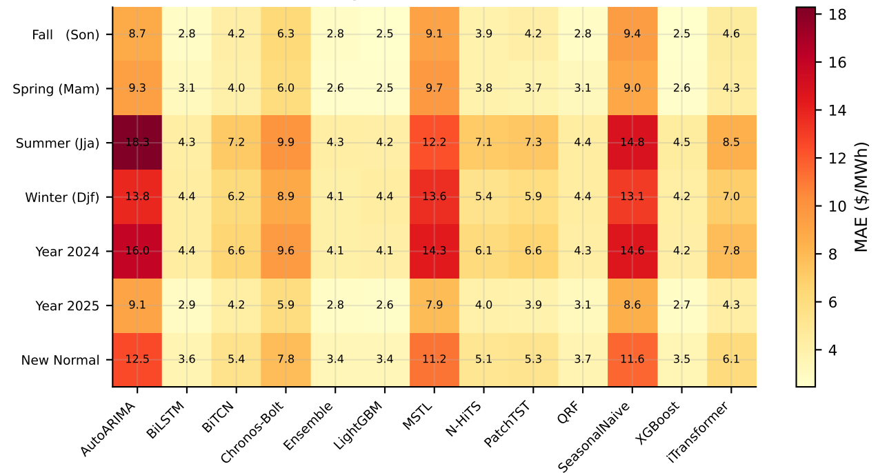
ERCOT — Regime MAE Heatmap ($/MWh)
