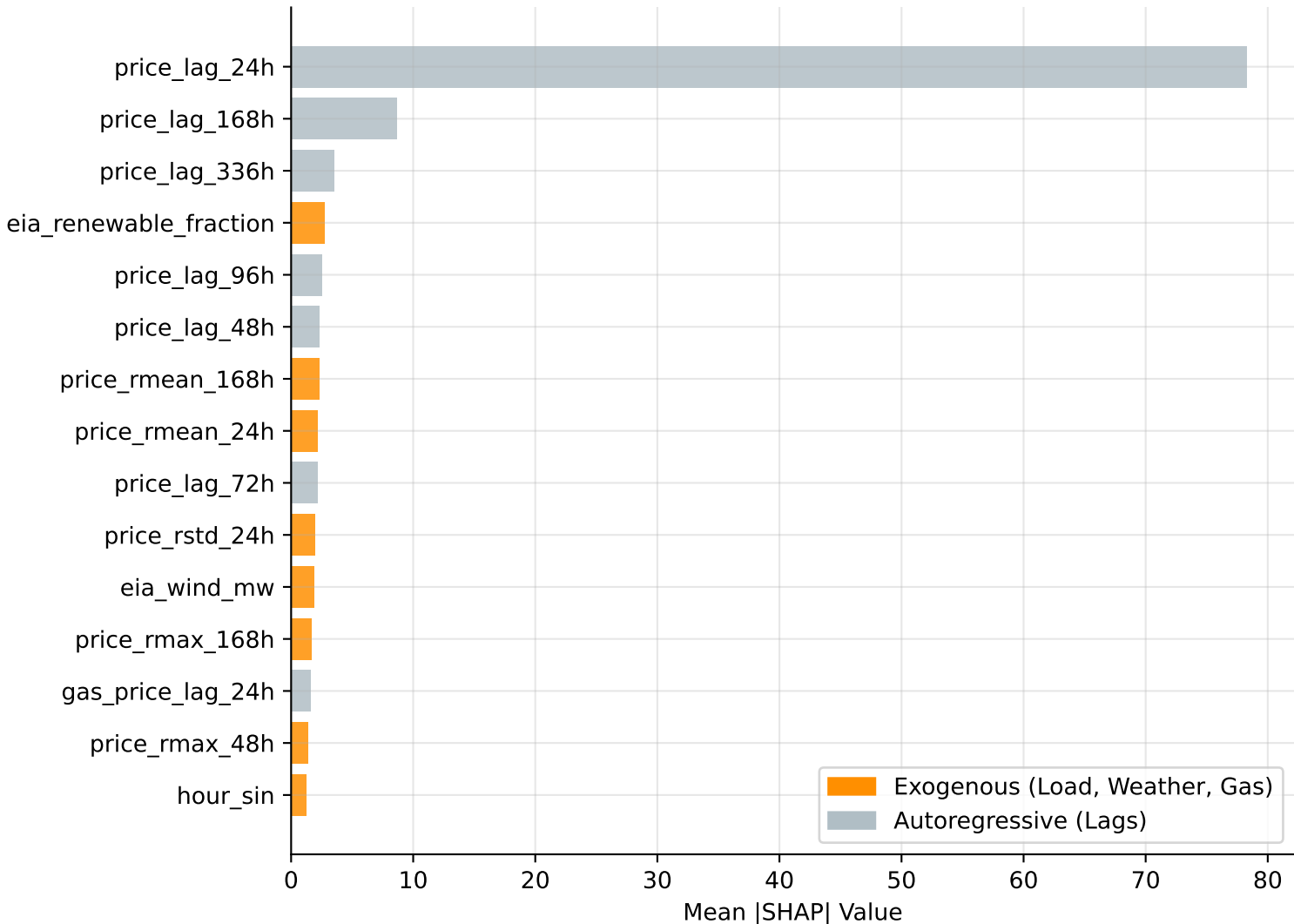
SHAP Feature Importance (LightGBM, ERCOT)
